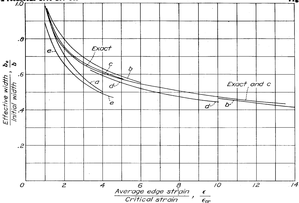
Figure 17.- Effective-width curves for a simply supported square plate according to different sources.
