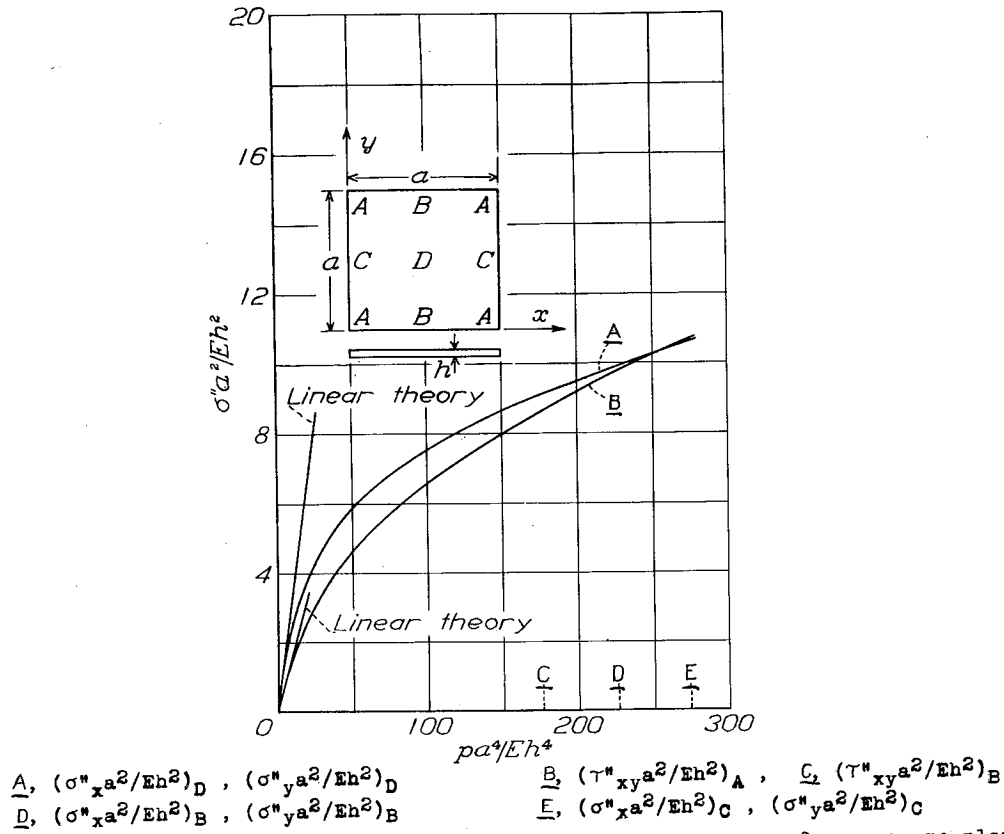
Figure 13.- Extreme-fiber bending stresses at the center and the corner for a square plate under uniform normal pressure. Edge displacement = 0; \mu = 0.316 . Linear theory from reference 9.
