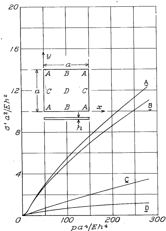
A, (\sigma'_x a^2/Eh^2)_C , (\sigma'_y a^2/Eh^2)_B (tension) B, (\sigma'_x a^2/Eh^2)_D , (\sigma'_y a^2/Eh^2)_D (tension) C, (\sigma'_x a^2/Eh^2)_B , (\sigma'_y a^2/Eh^2)_C (tension) D, (\sigma'_x a^2/Eh^2)_A , (\sigma'_y a^2/Eh^2)_A (tension)
