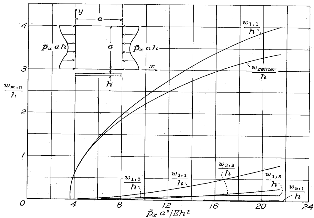
Figure 2.- Values of coefficients in table III for deflection function w = \sum_{m=1}^{\infty} \sum_{n=1}^{\infty} w_{m,n} \sin m\pi x/a \sin n\pi y/a for a square plate under edge compression. Average compressive stress in x-direction = \bar{p}_x ; \mu = 0.316 .
