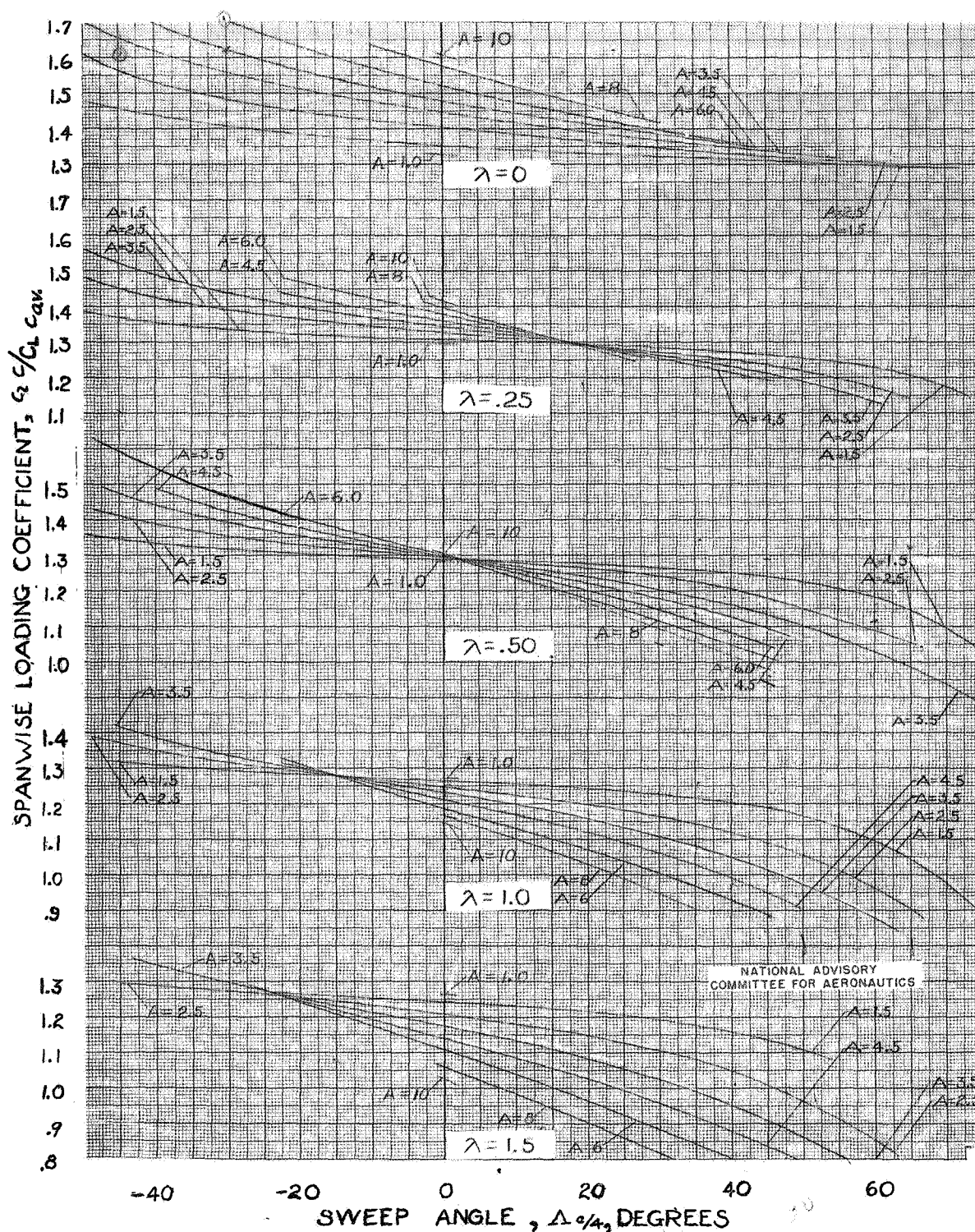
(a) FRACTION OF SEMISPAN, \eta = 0 , \gamma/4 = 1 FIGURE 5.- VARIATION OF SPANWISE LOADING COEFFICIENT WITH SWEEP FOR VARIOUS ASPECT RATIOS AND TAPER RATIOS.
