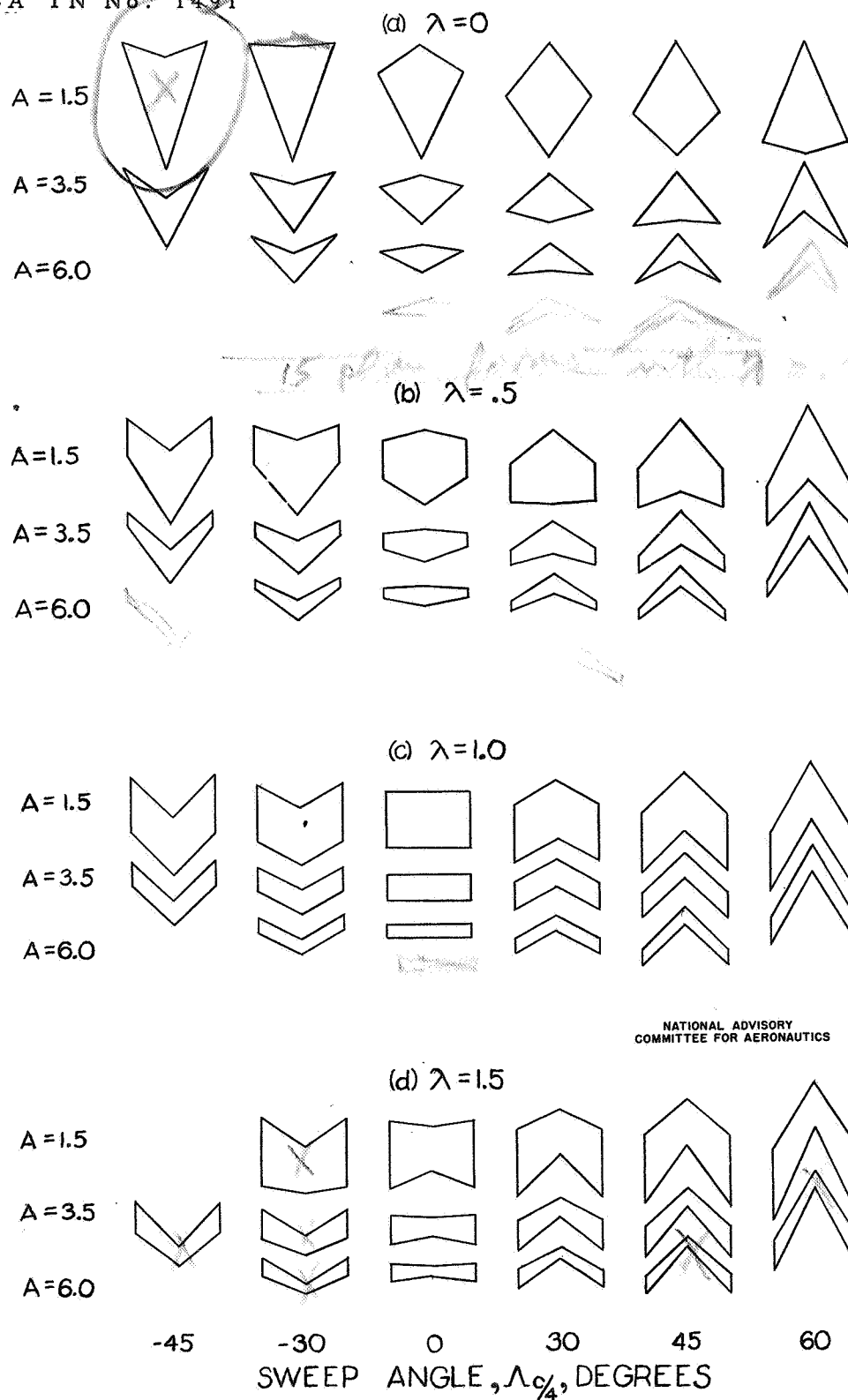
FIGURE 1.- RANGE OF PLAN FORMS INVESTIGATED BY THE WEISSINGER METHOD.
