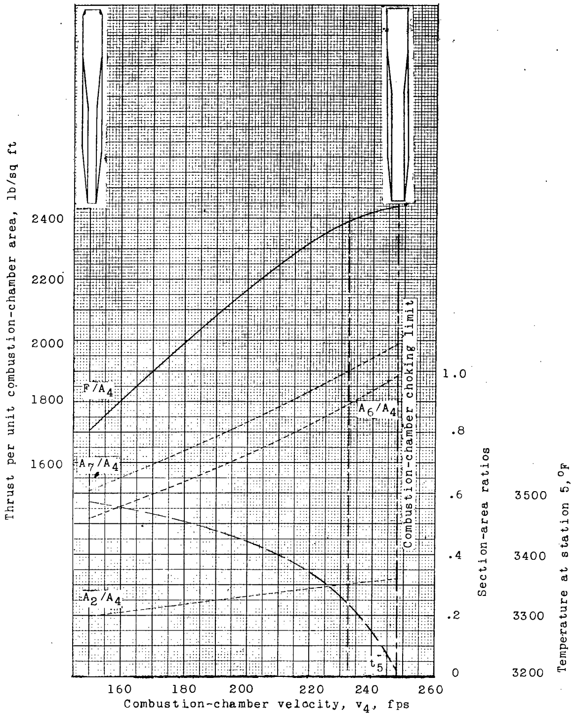
(b) Fuel-air ratio, 0.067. Figure 8. - Continued.
