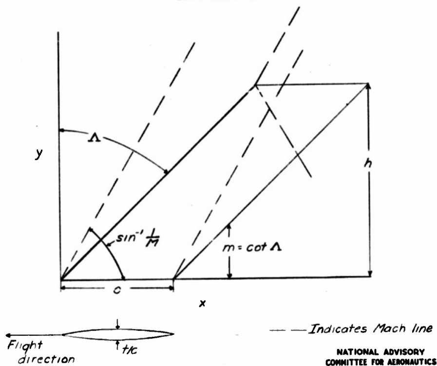
Figure 1. Symbols for wing plan form.
