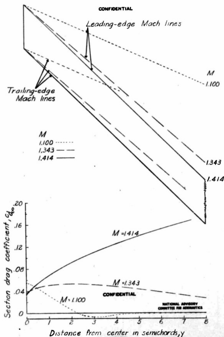
Figure 2. Typical distributions of section wave-drag coefficients along wing span. Biconvex profile at zero lift; sweepback angle, 4.5; thickness ratio in flight direction, 0.10.
