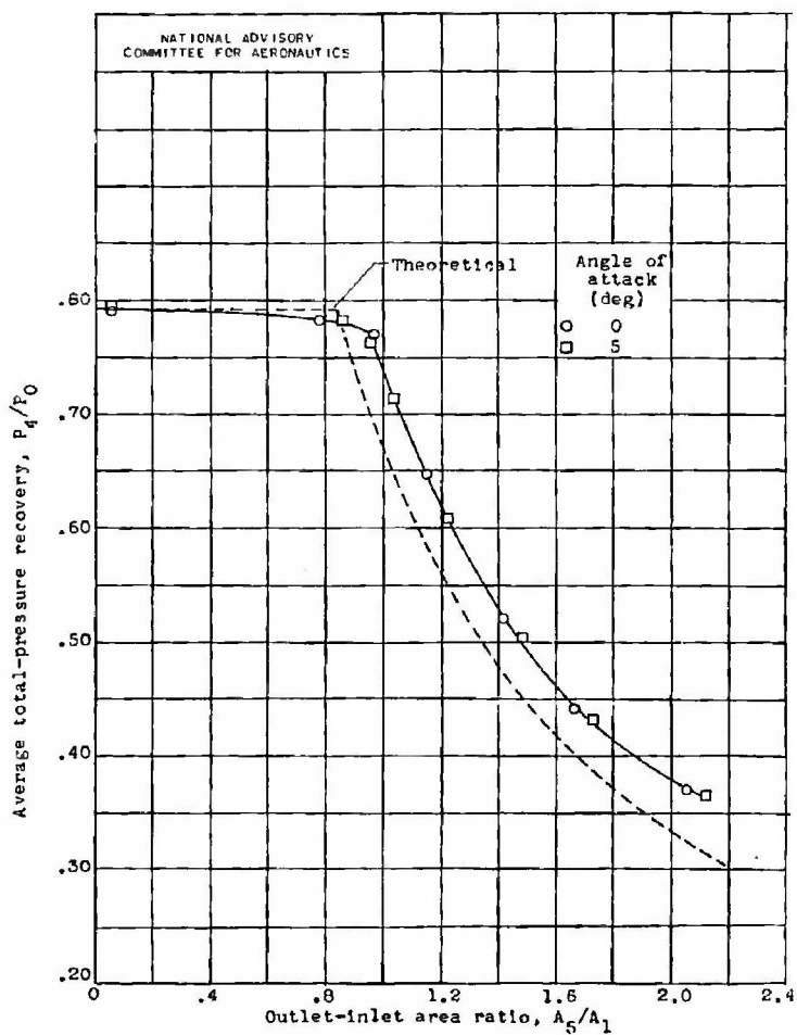
Figure 11.- Effect of combustion-chamber-outlet area on average total-pressure recovery with no throat and cylindrical inlet.
