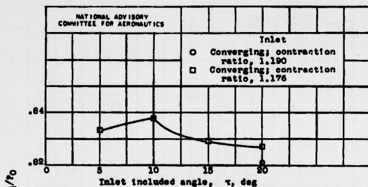
Figure 18.- Effect of inlet angle on maximum total-pressure recovery with normal shock inside diffuser. 2-inch throat, angle of attack of 0^\circ .
