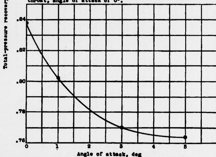
Figure 19.- Effect of angle of attack on maximum total-pressure recovery with normal shock inside diffuser. 10-1.176-0 configuration.
