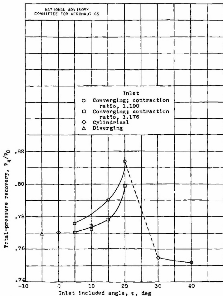
Figure 13.- Effect of inlet angle on maximum total-pressure recovery with normal shock inside diffuser. No throat, angle of attack of 0^\circ .
