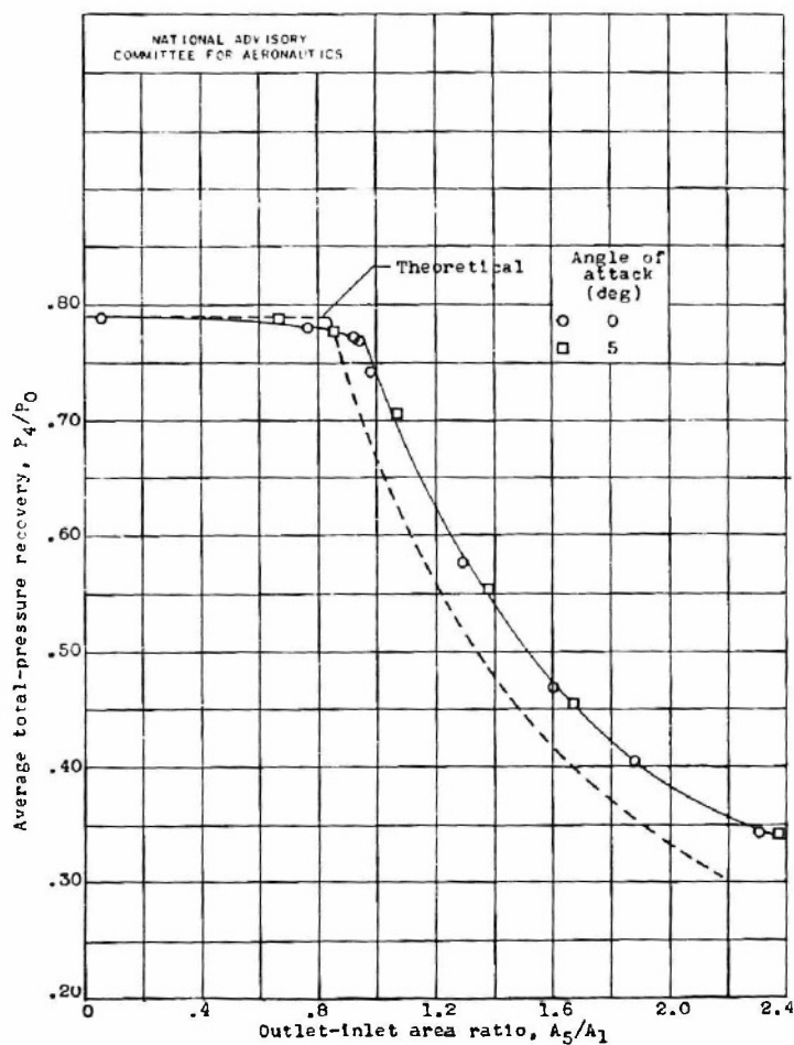
Figure 12.- Effect of combustion-chamber-outlet area on average total-pressure recovery with no throat and diverging inlet.
