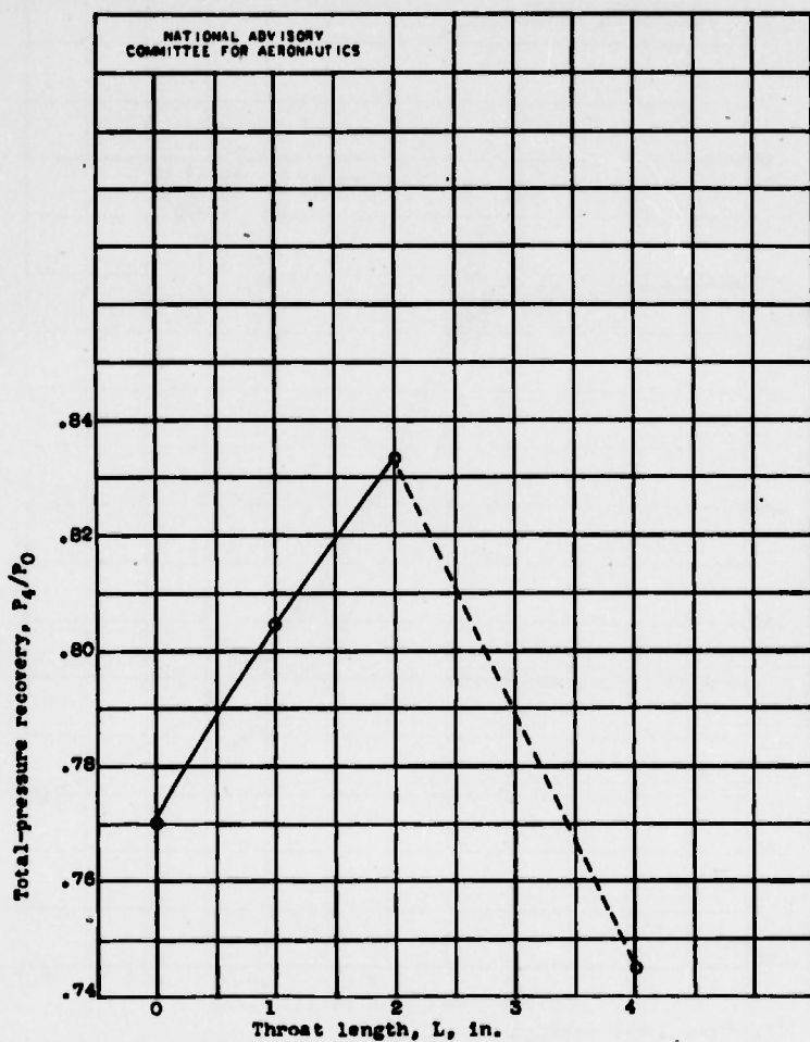
Figure 16.- Effect of throat length on maximum total-pressure recovery with normal shock inside diffuser. S=1.176 inlet, angle of attack of 0^\circ .
