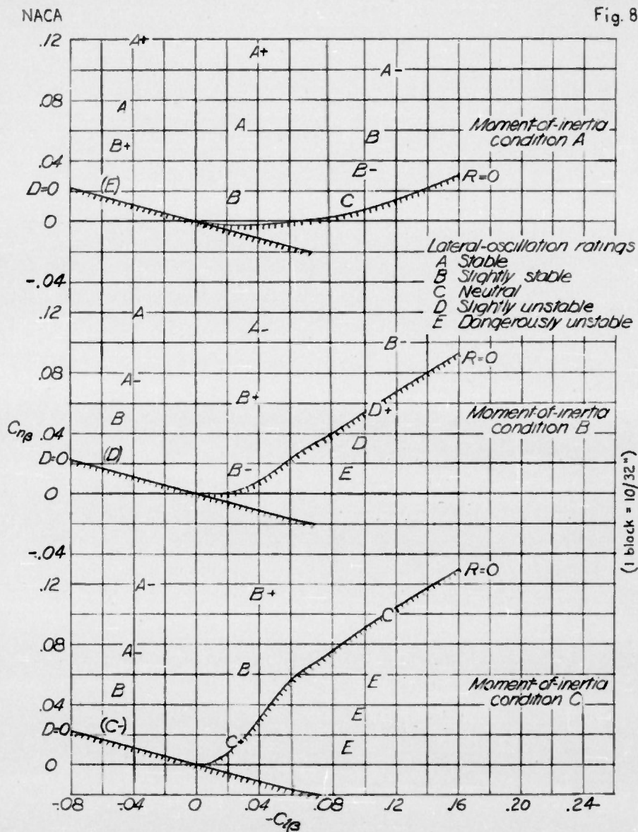
FIGURE 8.—Ratings for damping of lateral oscillation for different test conditions. C_l=1.0 . (Ratings possibly influenced by directional stability enclosed in parentheses)
