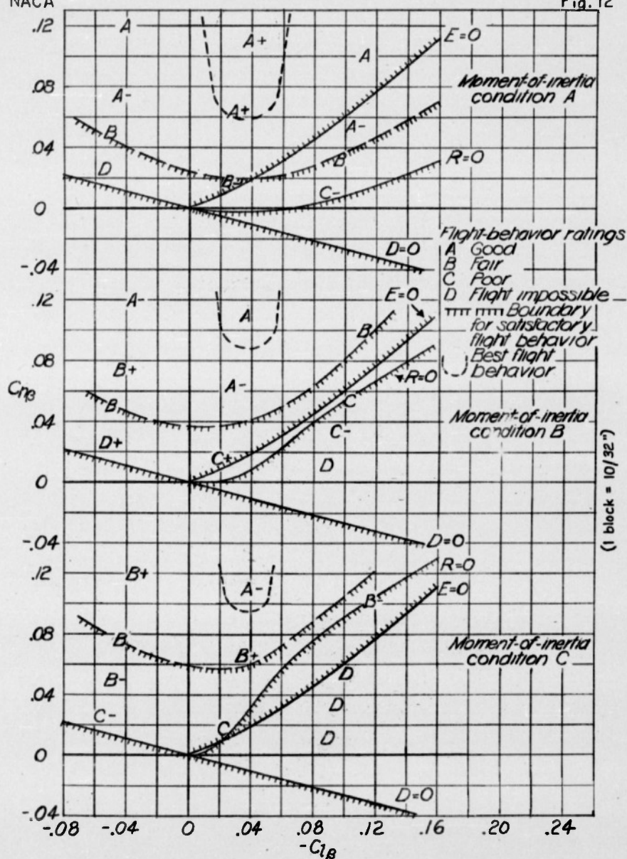
FIGURE 12.- Flight-behavior ratings for different test conditions. C_L=1.0 .
