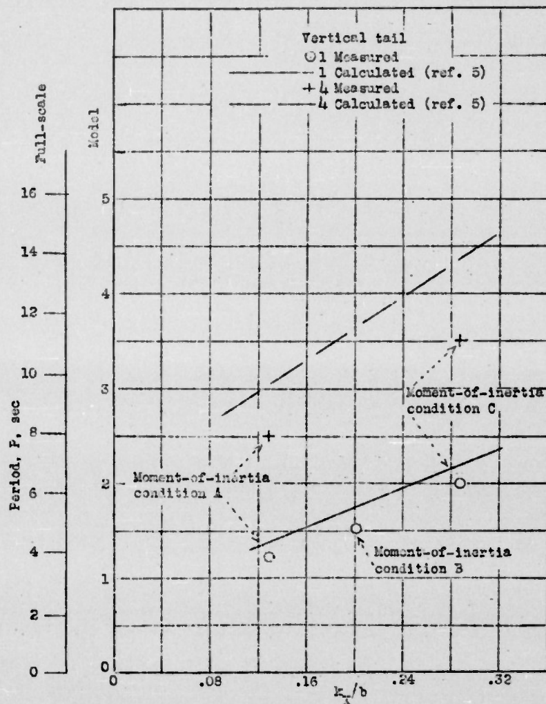
Figure 9.- Effect of moments of inertia on period of lateral oscillation. Small positive dihedral. C_L = 1.0 .
