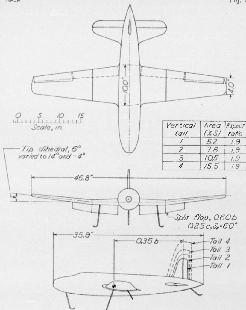
FIGURE 2.—Drawing of model used in free-flight-tunnel mass-distribution investigation
