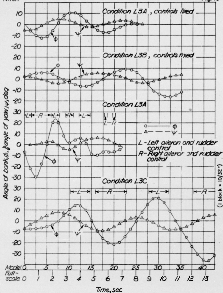
FIGURE 10.— Time histories of banking and yawing motions of model showing effect of increased moments of inertia on damping of lateral oscillation. Large positive dihedral. Vertical tail 3. C_L=1.0 .
