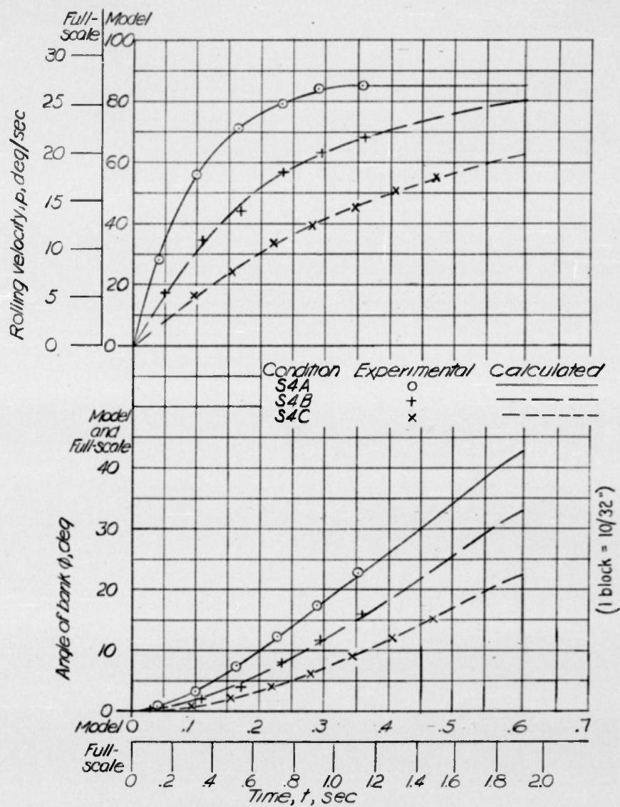
FIGURE 11.— Time histories of abrupt aileron maneuvers with different moment-of-inertia conditions. Small positive dihedral. Vertical tail 4. C_L=1.0 .
