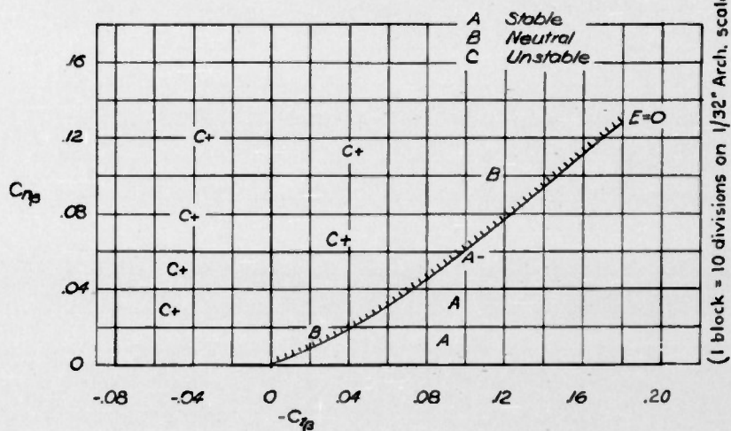
FIGURE 5.- Stability chart showing stability boundaries and model configurations. C_L=1.0 for all boundaries and configurations.
