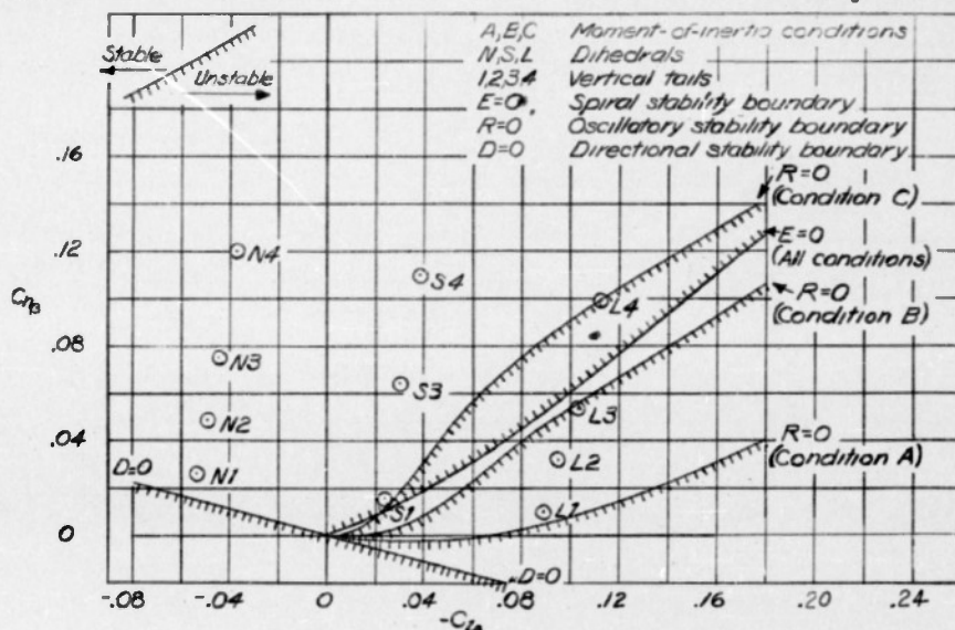
FIGURE 5.- Stability chart showing stability boundaries and model configurations. C_L=1.0 for all boundaries and configurations.
