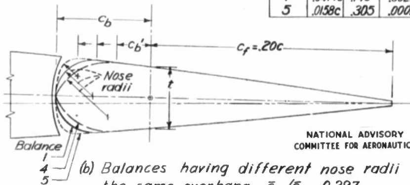
Figure 14.- Various plain-overhang balances derived for ailerons of wing used for illustrative example. NACA 23012 airfoil; \bar{c}_f/\bar{c} , 0.20; \frac{\bar{t}}{c_f} , 0.131; \bar{c}_b/\bar{c}_f , 0.397.
