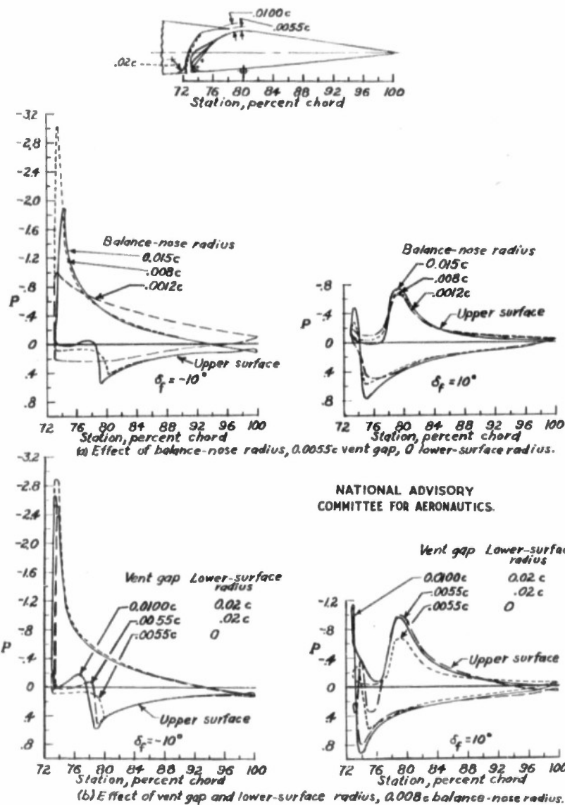
Figure 13.- Pressure distributions on a 0.20c flap with a 0.35c Frise balance. NACA 23012 airfoil section; model XVI of table II; data from reference 26; \alpha, 0^\circ ; M, 0.36 .
