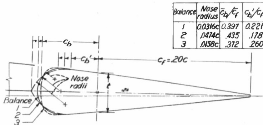
(a) Balances having different nose radii and different overhangs but the same balance factor. K_1 , 0.074; \frac{\bar{t}}{c_f} , 0.131; estimated Ch_\delta , -0.0011.
