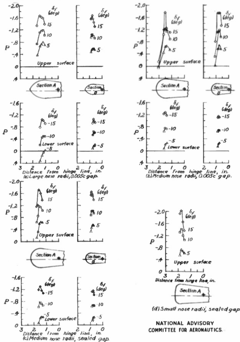
Figure 10.- Effect of aileron deflection and nose shape on the peak pressures at the nose of a 0.155c aileron with a 0.35c f balance. Model IX of table II, data from reference 19; \alpha , 0°; M \approx 0.1 .
