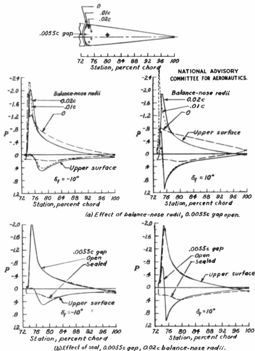
Figure 9.- Pressure distributions on a 0.20c flap with a 0.35c f blunt-nose balance. NACA 23012 airfoil section (model I of table II); data from reference 26; \alpha , 0°; M \approx 0.36 .
