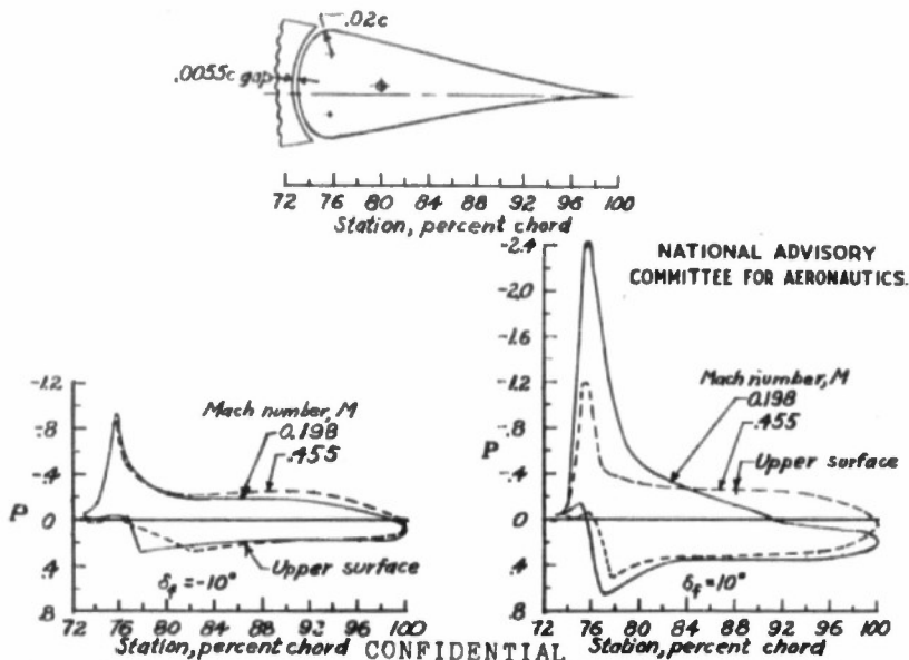
Figure 11.- Pressure distributions on a 0.20c flap with a 0.35c f blunt-nose balance. NACA 66(215)-216, a=1.0 airfoil section; model II of table II; data from reference 26; \alpha, 0^\circ ; gap, 0.0055c.
