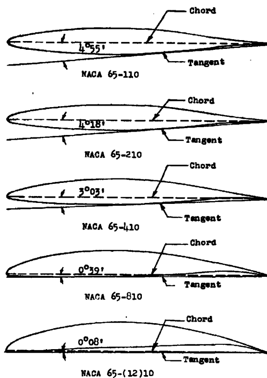
Figure 2.- NACA 65-series blower-blade sections.
