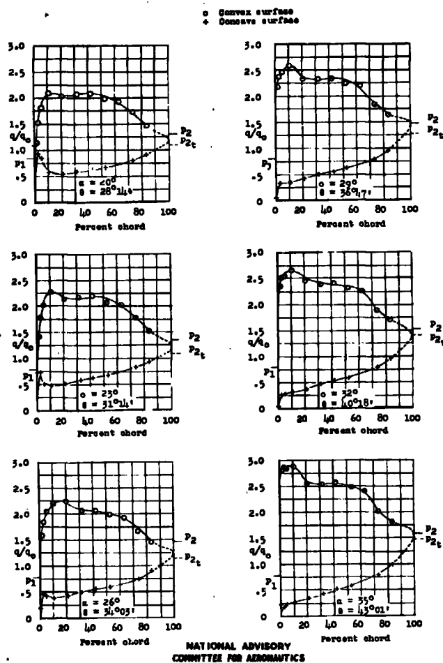
Figure 23.- Section pressure distributions for experimentally designed blower blade NACA 64-6108; stagger, 0^\circ ; solidity, 0.986; no recommended design condition.
