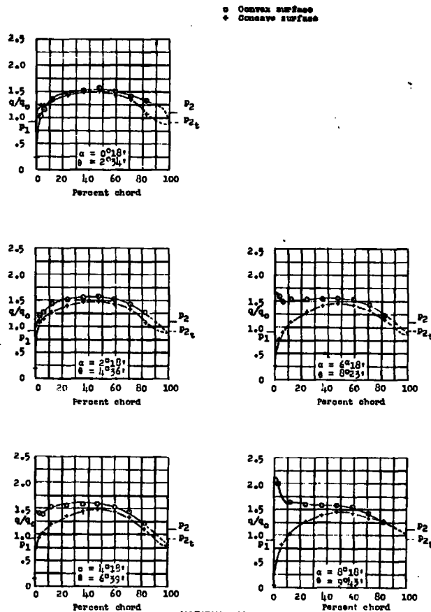
Figure 11.- Section pressure distributions for NACA 65-210 blower blades; stagger, 0°; solidity, 1.50; \alpha_d = 4^{\circ}18' .
