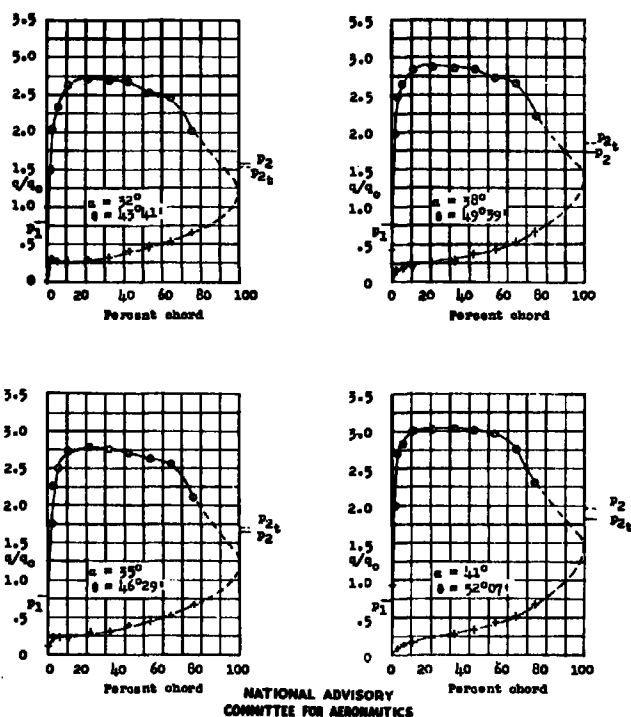
Figure 25. - Section pressure distributions for experimentally designed blower blade SAG 64-C106; stagger, 0^\circ ; solidity, 0.932; no recommended design condition.
