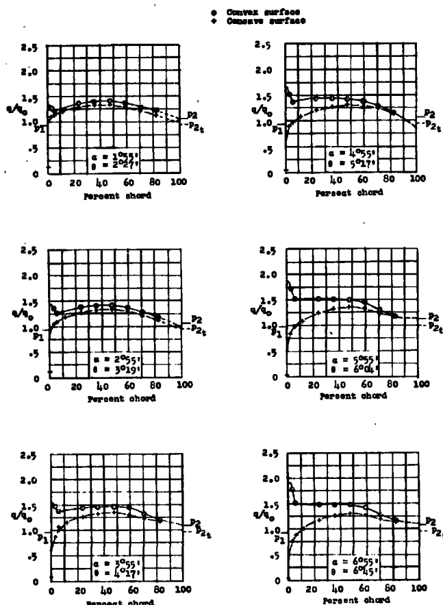
Figure 6.- Section pressure distributions for NACA 65-110 blower blade; stagger, 65°; solidity, 0.88; \alpha_0 .
