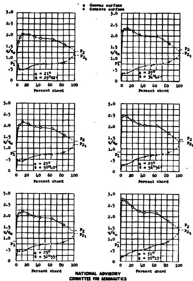
Figure 21.- Section pressure distributions for experimentally designed blower blade NACA 64-1A106; stagger, 0°; solidity, 0.976; no recommended design condition.
