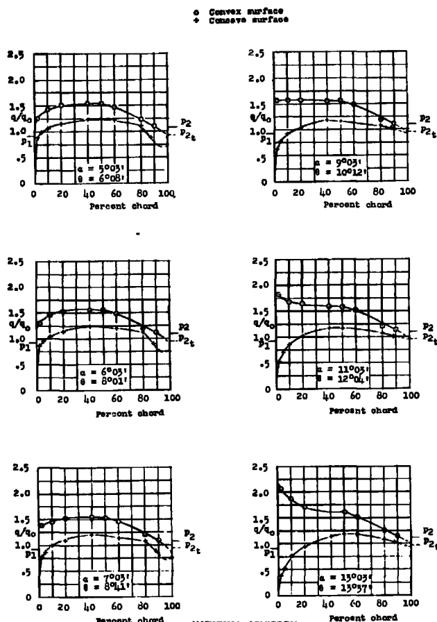
Figure 12.- Section pressure distributions for NACA 65-410 blower blade; stagger, 0^\circ ; solidity, 0.88; \alpha_0 = 7^\circ 05' .
