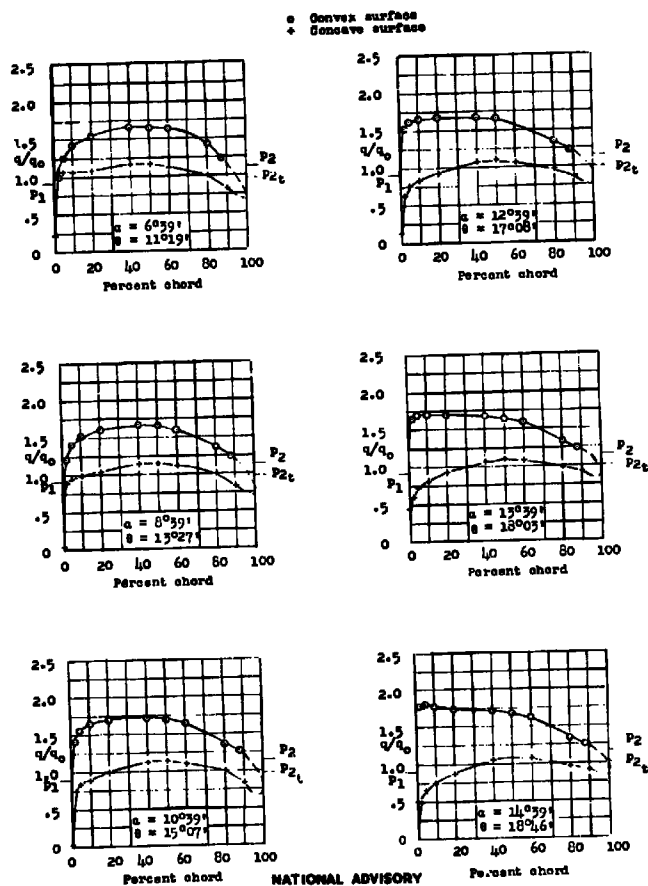
Figure 16.- Section pressure distributions for NACA 65-310 blower blade; stagger, 0^\circ ; solidity, 1.00; \alpha_0 = 11^\circ 59' .
