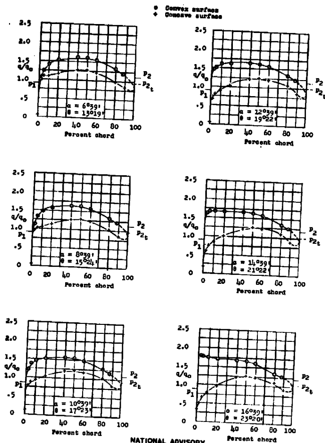
Figure 17.- Section pressure distributions for NACA 65-210 blower blade; stagger, 0°; solidity, 1.50; \alpha_d = 15^\circ 39' .
