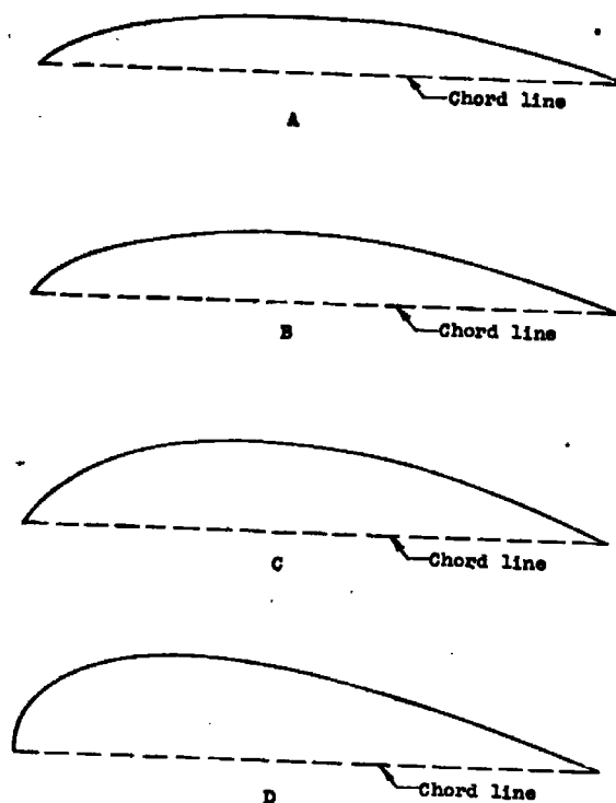
NATIONAL ADVISORY COMMITTEE FOR AERONAUTICS Figure 3.- Mean lines obtained from tests of flexible plates in cascade.
