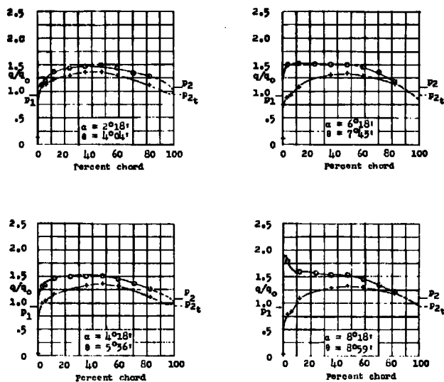
Figure 10.- Section pressure distributions for NACA 65-210 blower blade; stagger, 0^\circ ; solidity, 1.00; \alpha_d = 4^\circ 18' .
