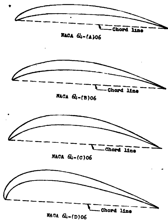
Figure 4.- Experimentally designed blower-blade sections.
