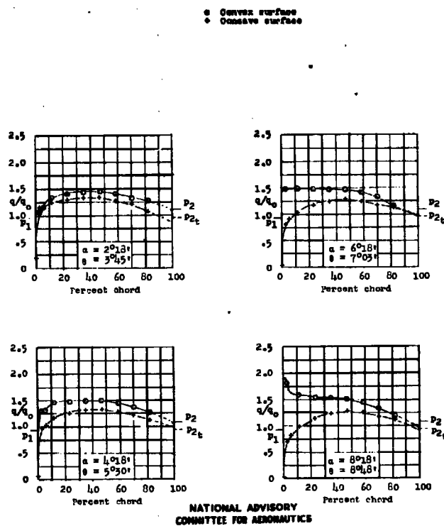
Figure 9.- Section pressure distributions for NACA 65-210 blower blade; stagger, 0^\circ ; solidity, 0.88; \alpha_d = 4.018^\circ .
