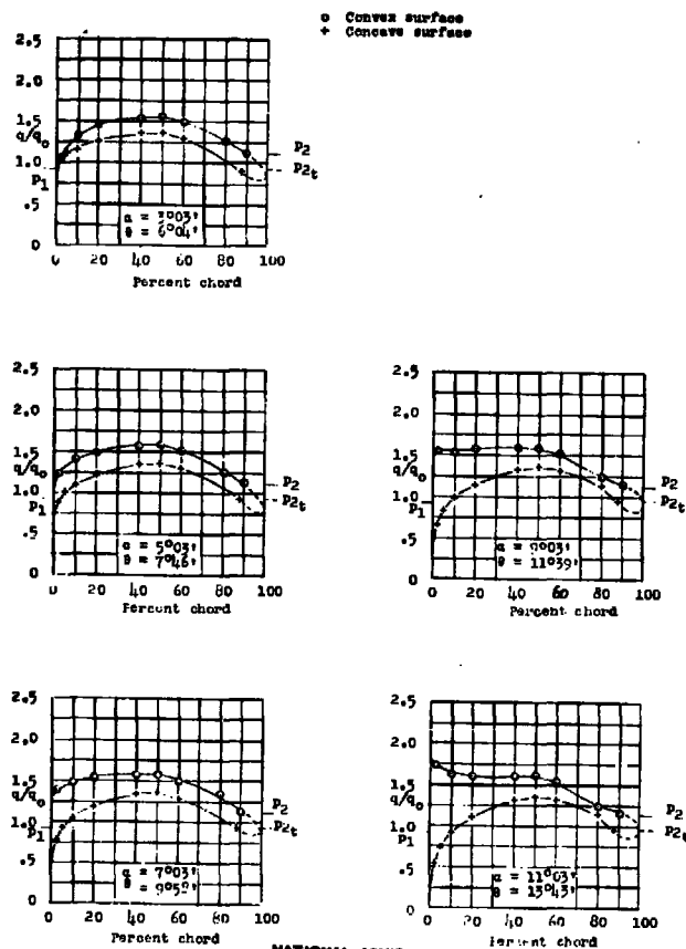
Figure 14.- Section pressure distributions for NACA 65-410 lower blades; stagger, 0°; solidity, 1.50; \alpha_0 = 5.00^\circ .
