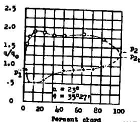
Figure 22.- Section pressure distributions for experimentally designed blower blade NACA 64-(A)06; stagger, 0^\circ ; solidity, 1.465; range of \alpha , 21^\circ to 33^\circ .
