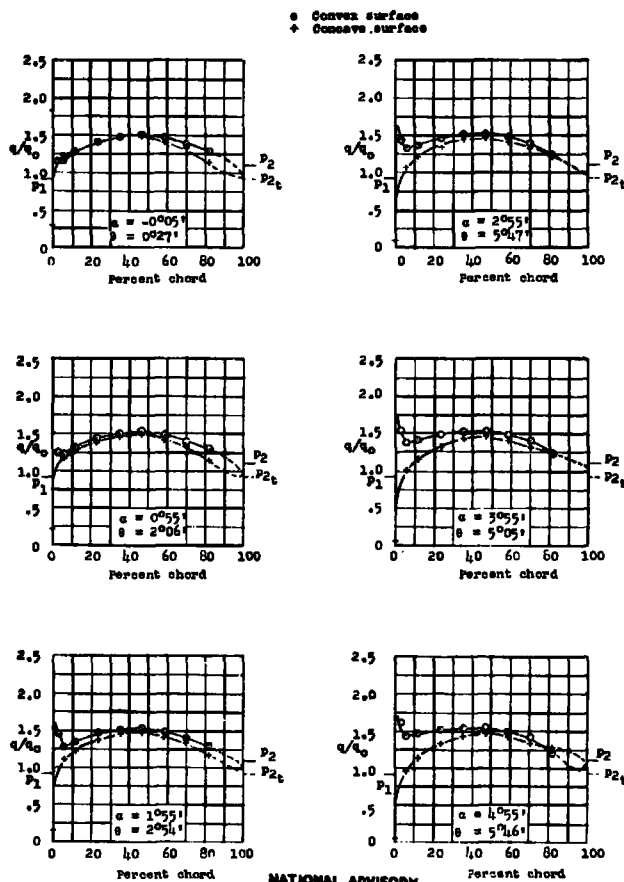
Figures 8.- Section pressure distributions for NACA 65-110 blower blade; stagger, 0°; solidity, 1.50; no \alpha_d .
