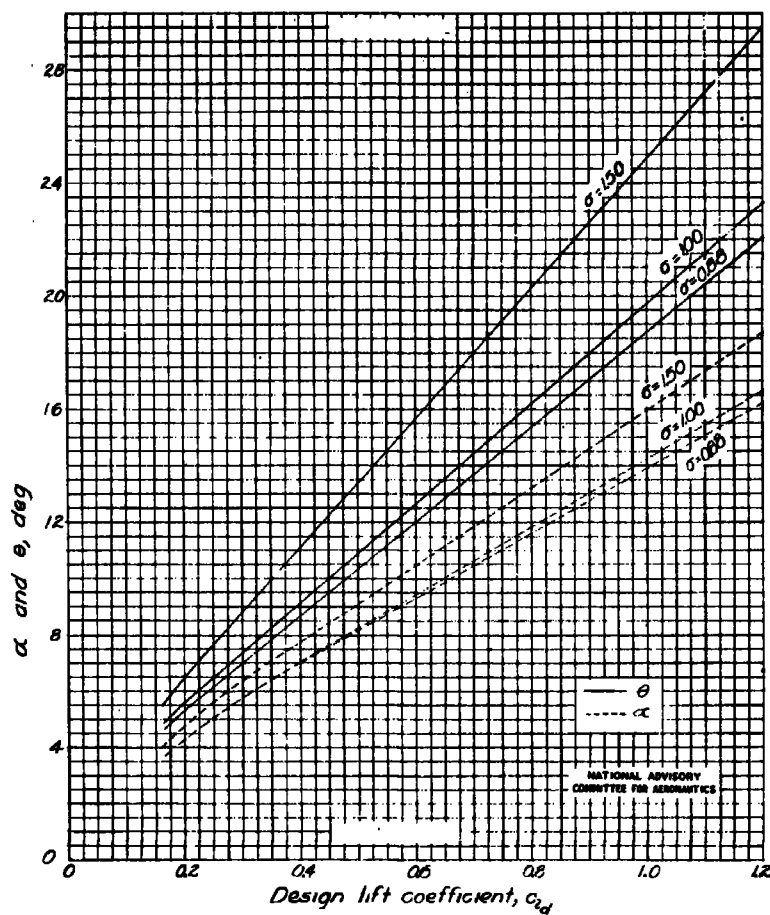
Figure 33- Design chart for NACA 65-series blower-blade sections; stagger, 0^\circ .
