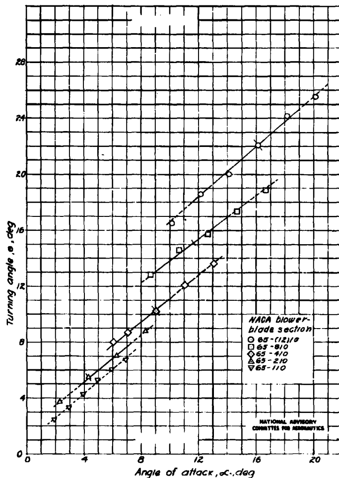
Figure 29.- Angle through which the air is turned in passing through a cascade. NACA 65-series blower-blade sections; stagger, 0°; solidity, 0.88. (Cross bar indicates design point; solid line indicates range of peak-free pressure distributions.)
