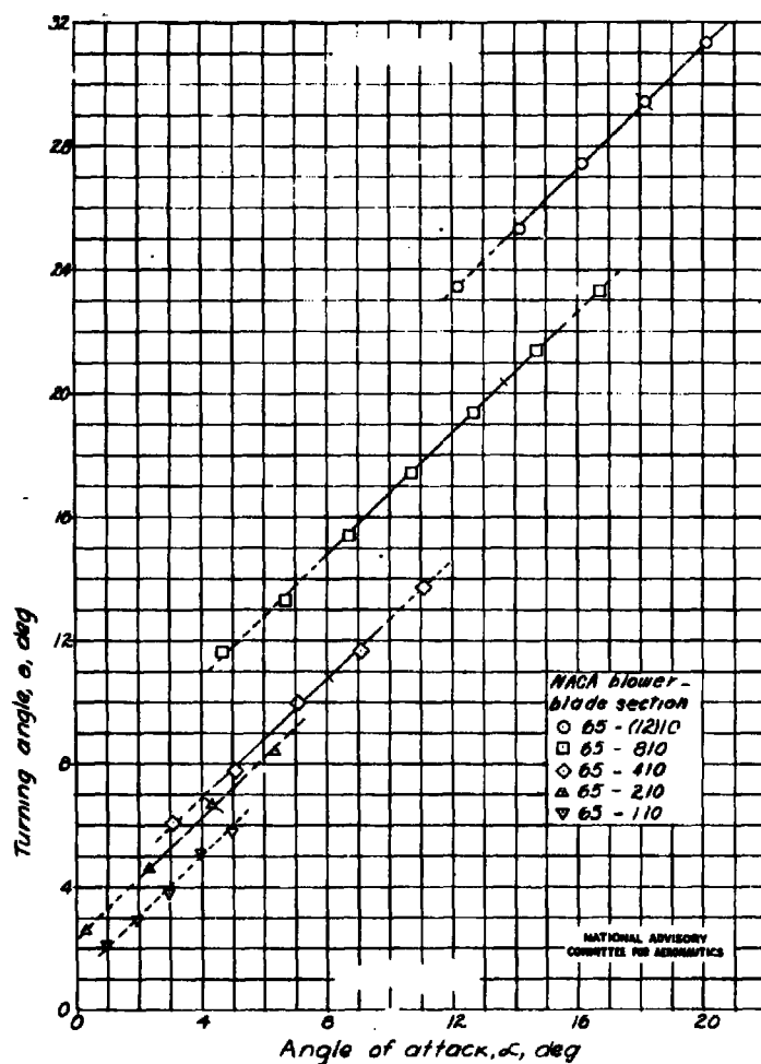
Figure 31.- Angle through which the air is turned in passing through a cascade. NACA 65-series blower-blade sections; stagger, 0°; solidity, 1.50. (Cross bar indicates design point; solid line indicates range of peak-free pressure distributions)
