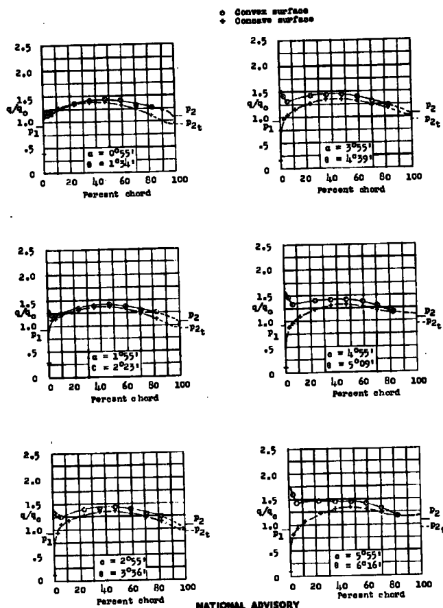
Figure 7.- Section pressure distributions for NACA 65-110 blower blade; stagger, 0^\circ ; solidity, 1.00; no a_1 .
