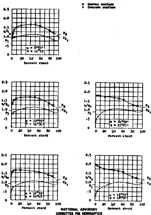
Figure 15.- Section pressure distributions for NACA 65-810 blower blade; stagger, 0^\circ ; solidity, 0.88; \alpha_0 = 11.039^\circ .
