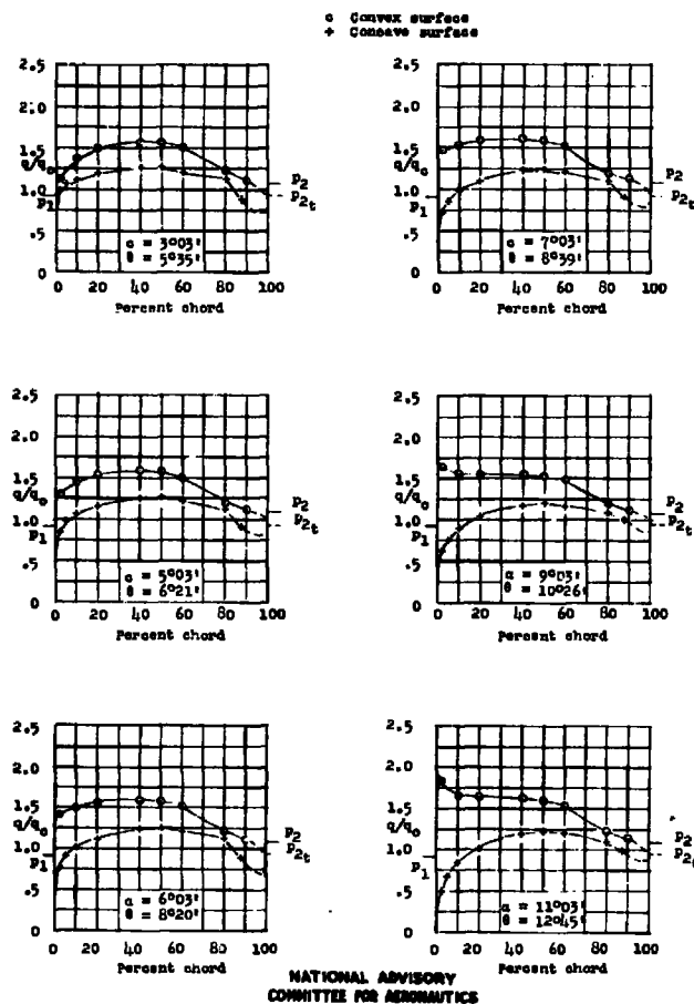
Figure 13.- Section pressure distributions for NACA 65-410 blower blade; stagger, 0°; solidity, 1.00; \alpha_d = 7.003^\circ .
