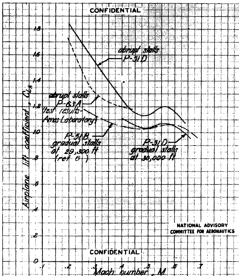
Figure 4-Comparison between maximum lift coefficients obtained in abrupt stalls of P-51D and P-63A airplanes and those obtained in gradual stalls of P-51D and P-51B airplanes.
