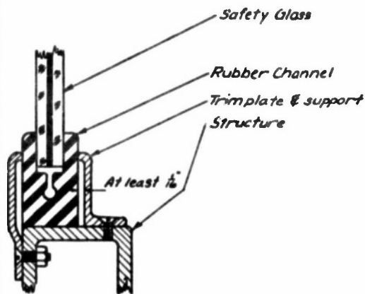
Figure 12.- Showing the construction of a proper window mounting (U.S. Patent #19991832); vibration damping is obtained by allowing space for the rubber channel to deform under the action of stresses.
