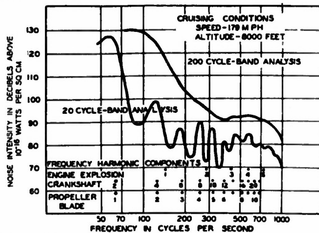
Figure 23.- Frequency analysis of noise in the pilot's compartment of an airplane with direct driven propeller.
