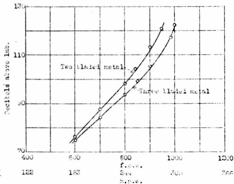
Figure 10.- Noise level (in db above 1 millibar; add 13.8 db to convert to usual reference level) produced by airscrews at various tip speeds.
