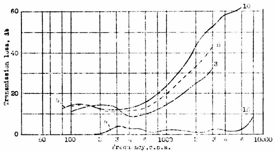
Figure 18.-Transmission loss of multiple walls: Curve a: 15 sheet cellophane wall ( f_c = 6700 c.p.s.); curves b: 3, 5, and 10 sheet roofing-paper wall ( f_c = 200 c.p.s.).
