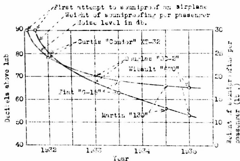
Figure 25.- Progress of soundproofing of aircraft showing the reduction of noise level and reduction in weight of acoustical treatment required. Approximately 14 db should be added to noise levels to convert to usual reference level.
