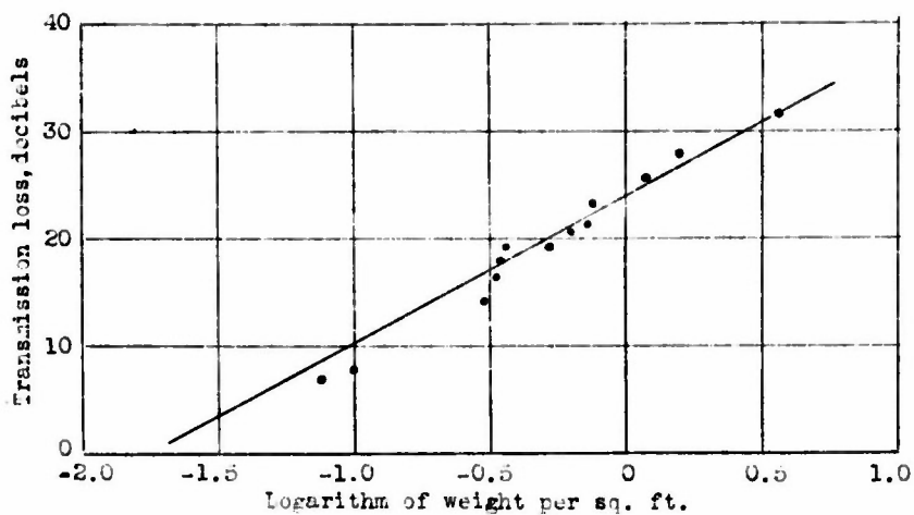
Figure 17.- Dependence of the transmission loss homogeneous panels on the logarithm of weight in lb/sq. ft.
