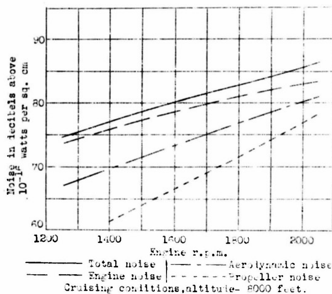
Figure 24.- Relation of the various components to the total noise in the cabin of an airplane with a three blade geared propeller.
