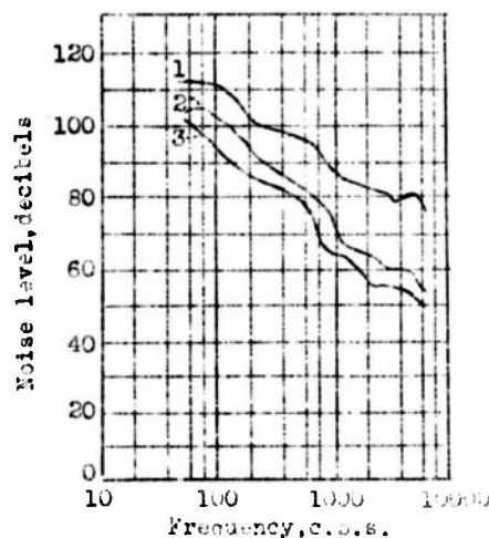
Figure 20.- Frequency analysis of the noise within the cabin; 1-FW200 without treatment, 2-FW200 with treatment, 3-Ju52 with treatment.
