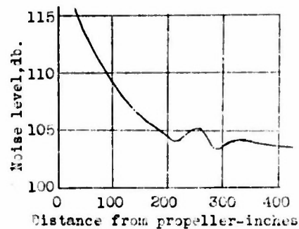
Figure 9.- Variation of noise level outside of cabin wall with distance from the plane of the propeller. Observations made at fuselage wall.
