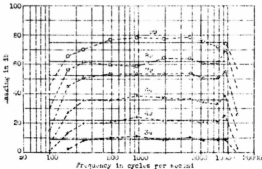
Figure 7.- Decibel shift of threshold of hearing (masking in db) in presence of noise containing a wide range of audible frequencies; numbers on the curves represent the sound level in db of the masking noise. For example, for a masking noise of 70 db, the threshold for a 500 cycle note is shifted by 43 db.
