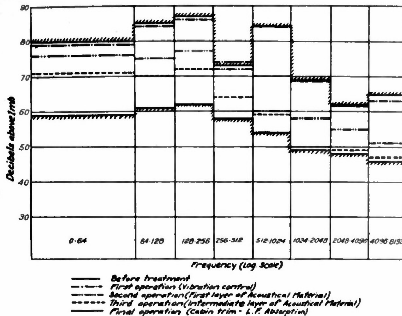
Figure 22.- Progress of noise reduction at various stages of the treatment. Approximately 14 db should be added to noise levels to convert to usual reference level.
