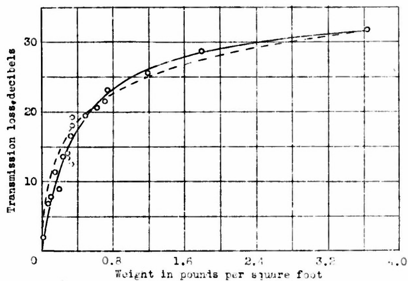
Figure 16.- Variation of transmission loss with weight for homogeneous panels.
