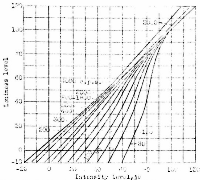
Figure 3.- Loudness level of pure tones at different intensity levels.
