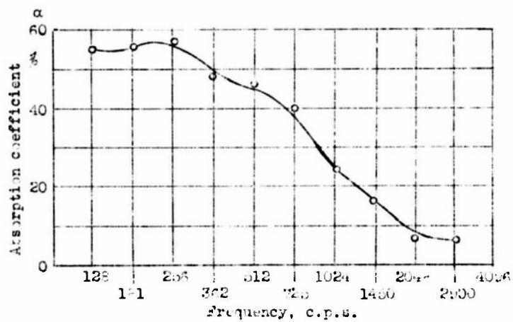
Figure 15.- Sound absorption coefficient of 3 layers of oilcloth with 5 cm air-space between layers.
