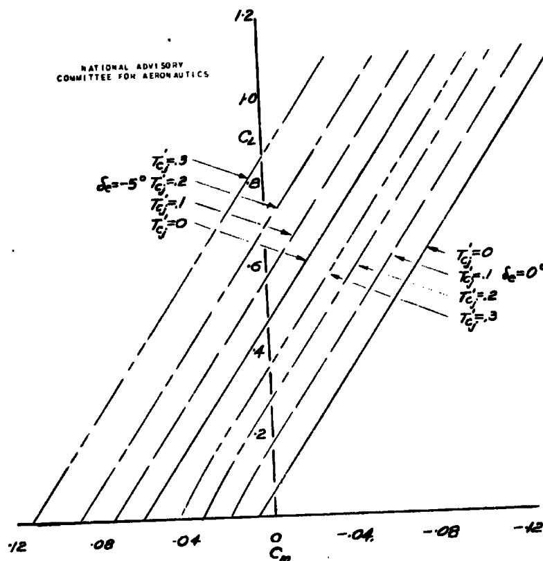
FIGURE 13.—VARIATION OF PITCHING-MOMENT COEFFICIENT WITH LIFT COEFFICIENT AT CONSTANT THRUST COEFFICIENT FOR TWO-ENGINE AIRPLANE MODEL. FLAPS RETRACTED.
