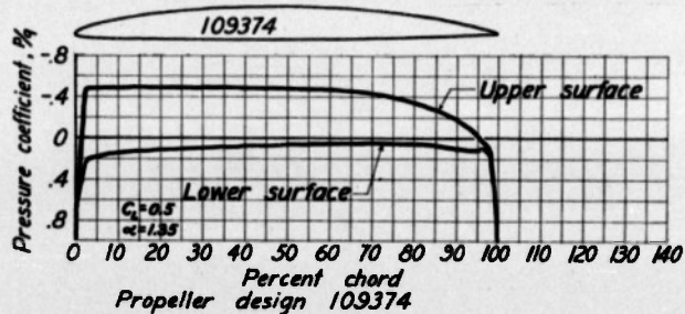
Figure 5.— Blade section and theoretical pressure distribution at the 0.7 radius for each propeller design.
