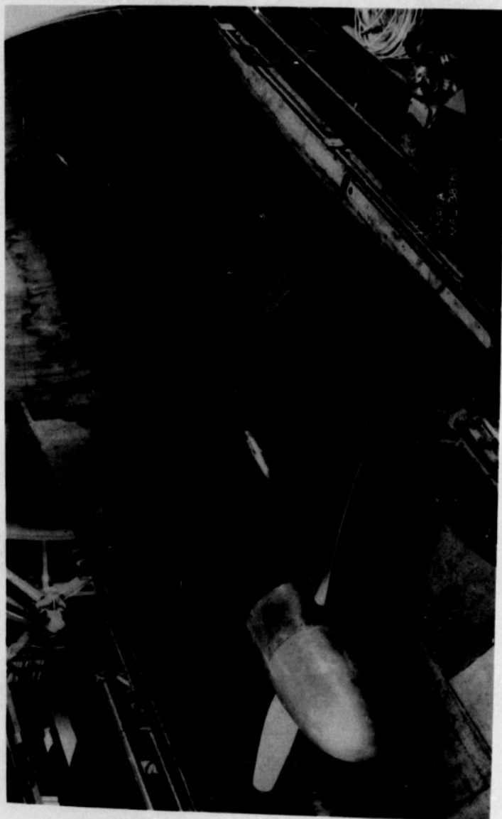
Figure 1.- Propeller dynamometer in test section, blades with no trailing-edge extension, tunnel open.
