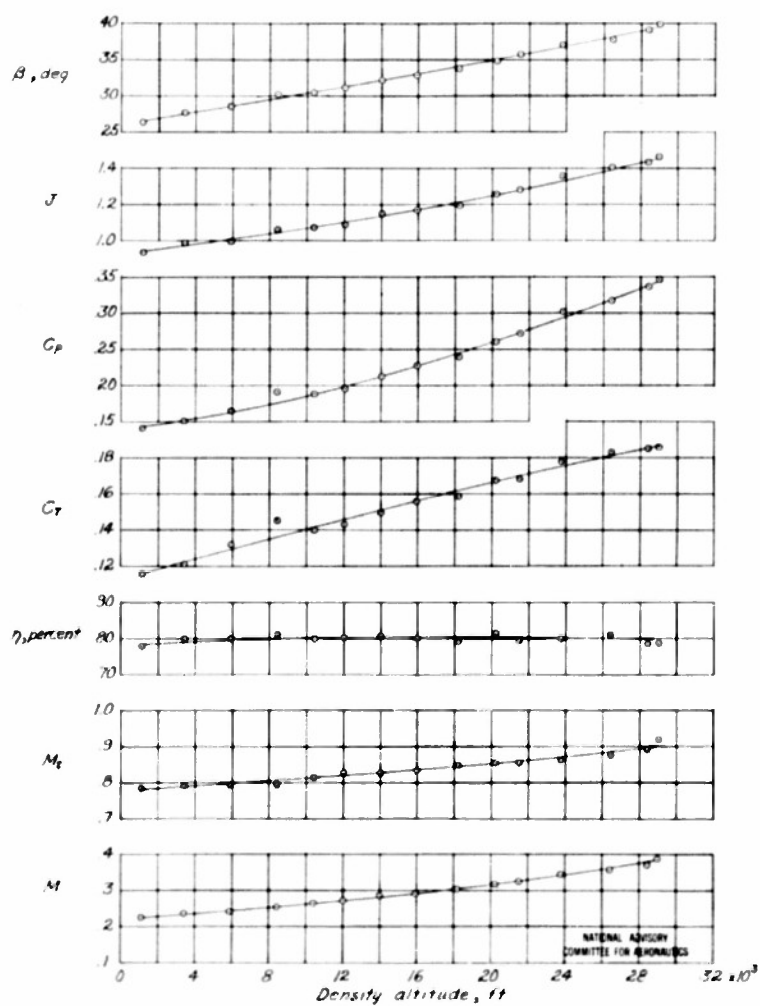
Figure 5.- Normal-power climb at an indicated airspeed of 160 miles per hour. Curtiss No 714-102-12 four-blade propeller on Republic P-47C airplane.
