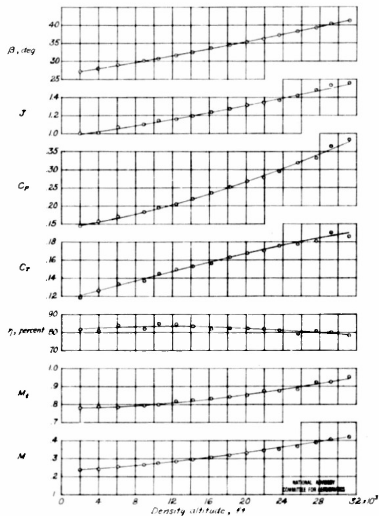
Figure 6.- Normal-power climb at an indicated airspeed of 165 miles per hour. Curtiss No. 74-102-12 four-blade propeller on Republic P-47C airplane.
