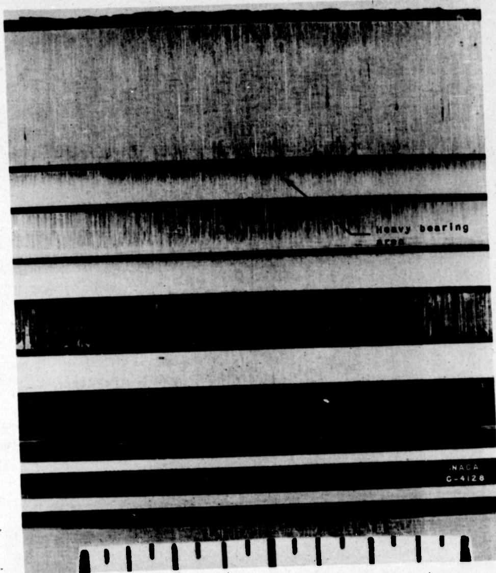
Figure 10. - Condition of surface of the top five piston rings, 180° from gaps, after operation in previously used, straight-bore porous chrome-plated cylinder barrel with standard ring assembly after test 7. X5.
