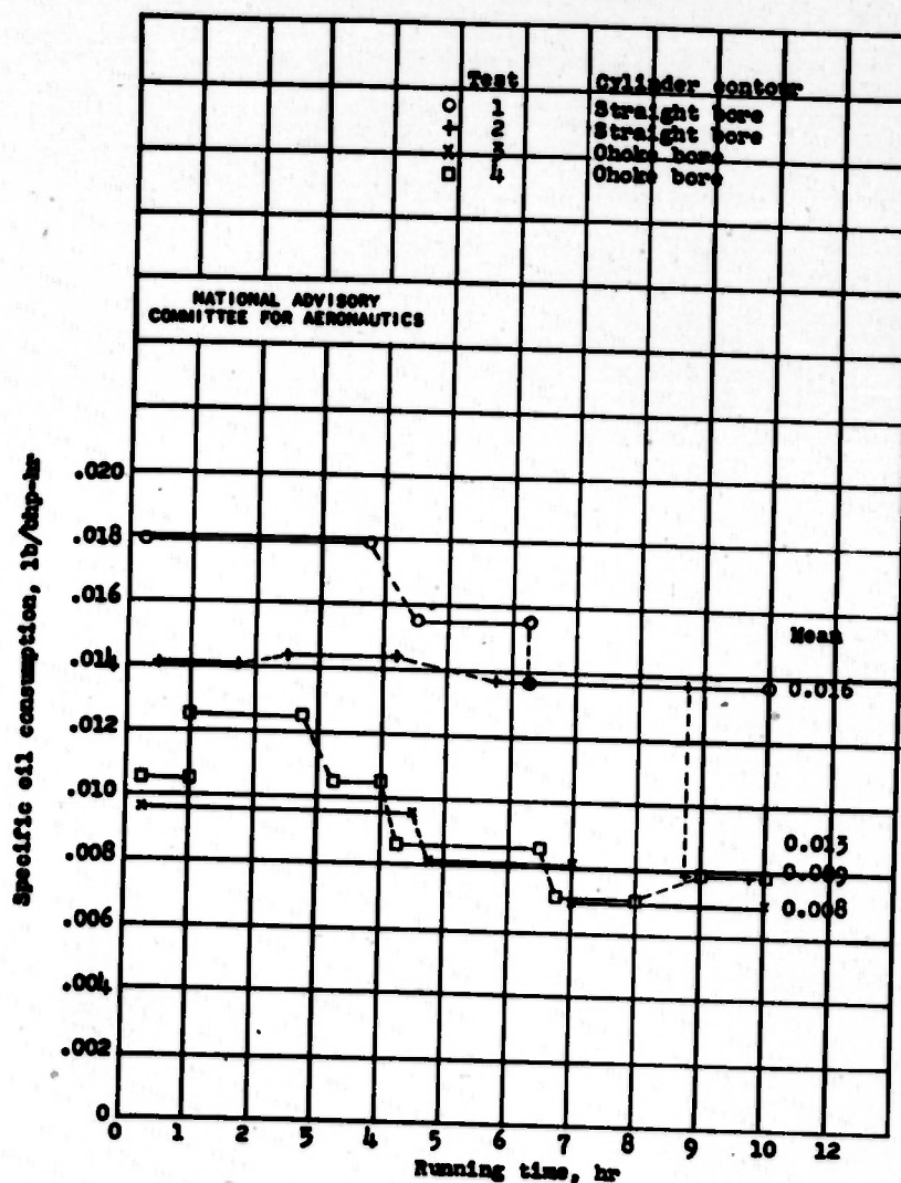
Figure 4. - Specific oil consumption for tests 1, 2, 3, and 4 of straight-bore and choke-bore porous chrome-plated cylinder barrels with standard rings. Engine speed, 2400 rpm; brake mean effective pressure, 192 pounds per square inch.
