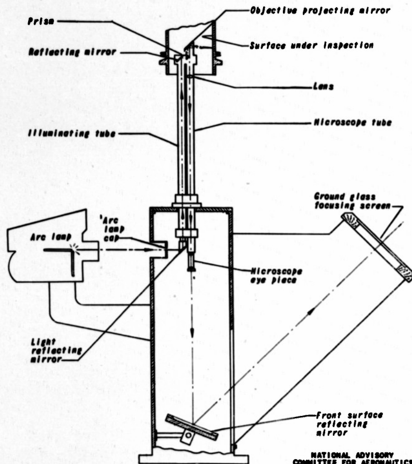
Figure 3. - Optical system of the internal-surface projector.
