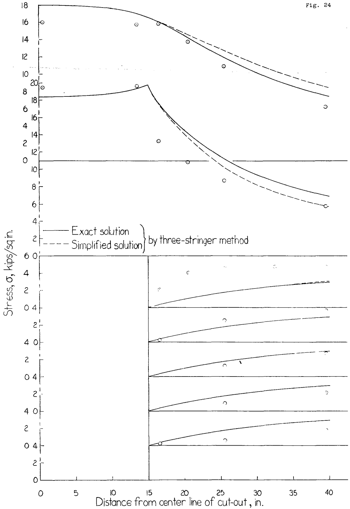
Figure 24.-Stringer stresses in 16 stringer panel with 12 stringers cut and L=15.0 inches.
