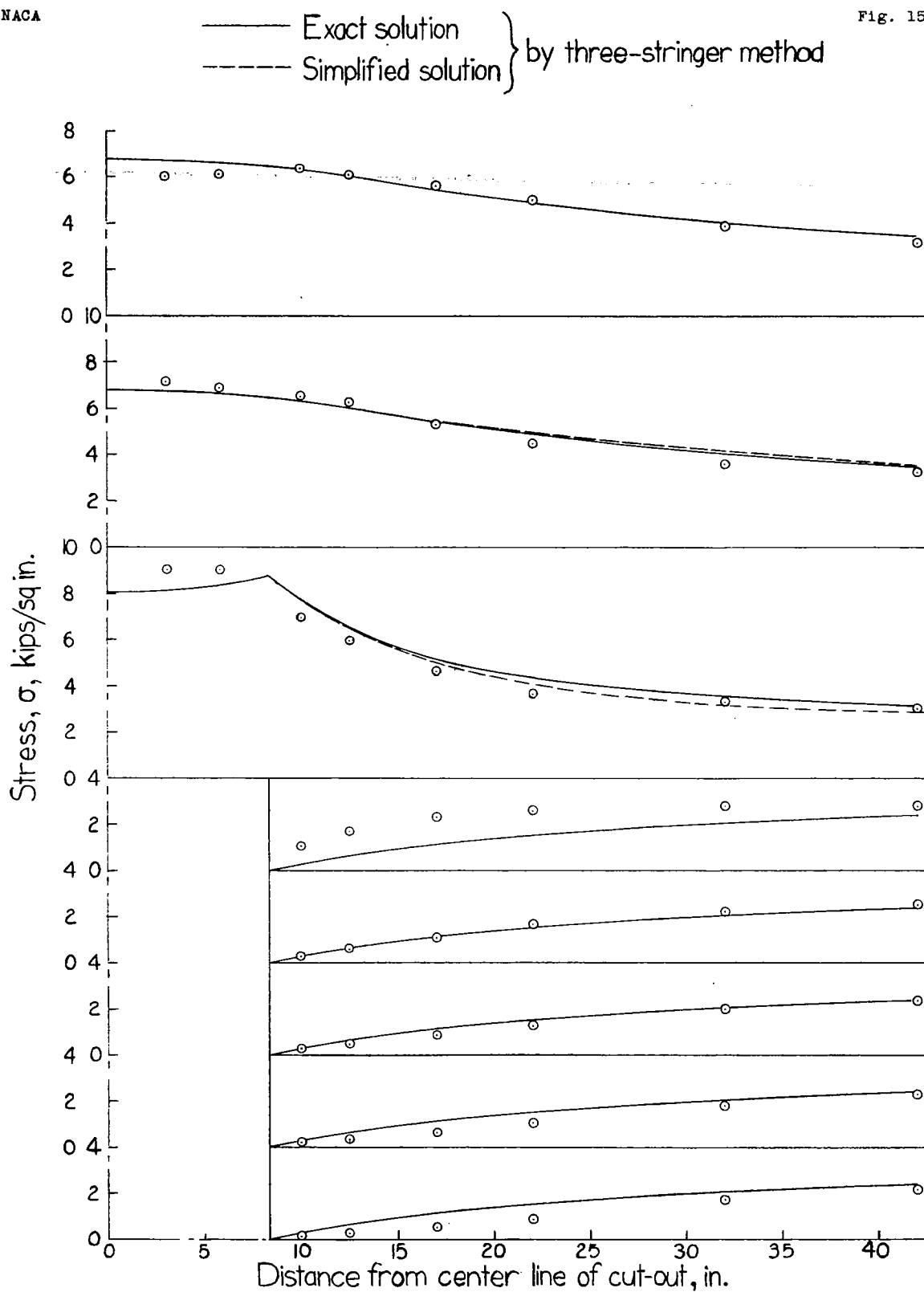
Figure 15.-Stringer stresses in 15-stringer panel with 9 stringers cut and L=8.3 inches.
