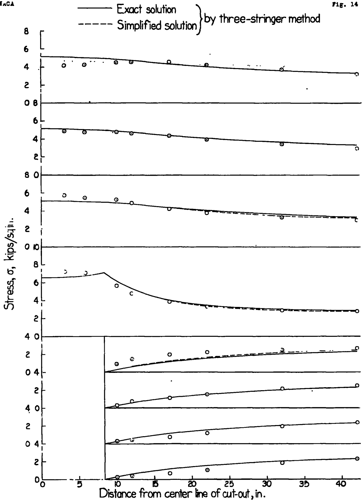
Figure 14.—Stringer stresses in 15-stringer panel with 7 stringers cut and L=8.3 inches.
