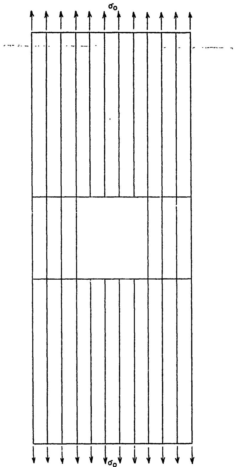
Figure 1.- Axially loaded panel with cut-out.
