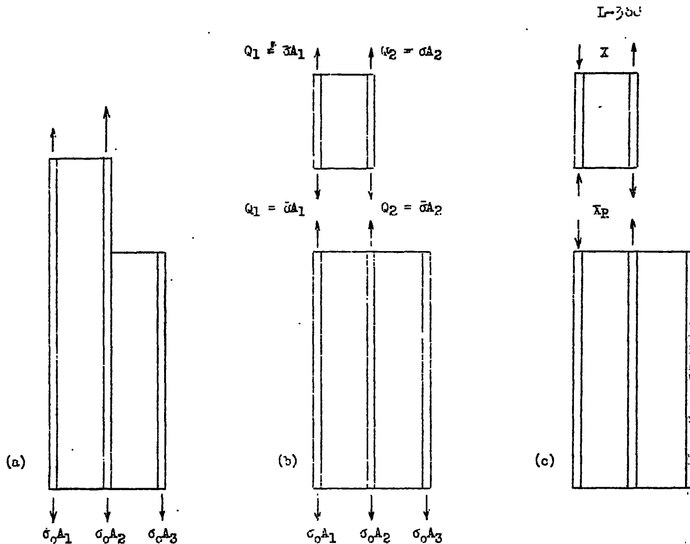
Figure 34.- Resolution of loads on three-stringer structure.
