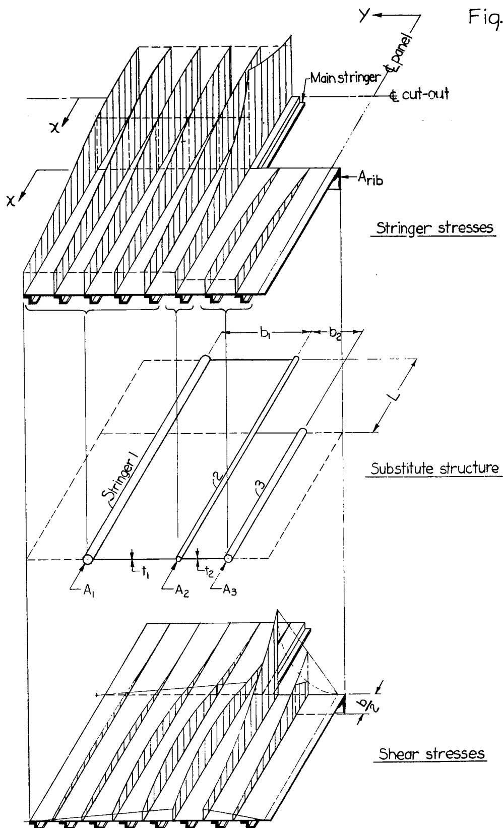
Figure 2.- Stress distribution around cut-out by three-stringer method.
