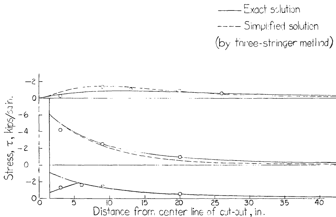
Figure 26.—Shear stresses in 16-stringer panel with 4 stringers cut and L=1.5 inches.
