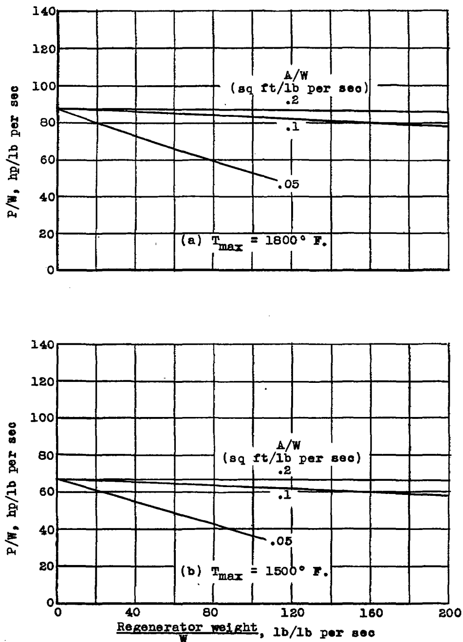
Figure 15.- Variation of thrust power per pound of air per second with heat-exchanger weight per pound of air per second. Altitude, sea level; R_c = 3 .
