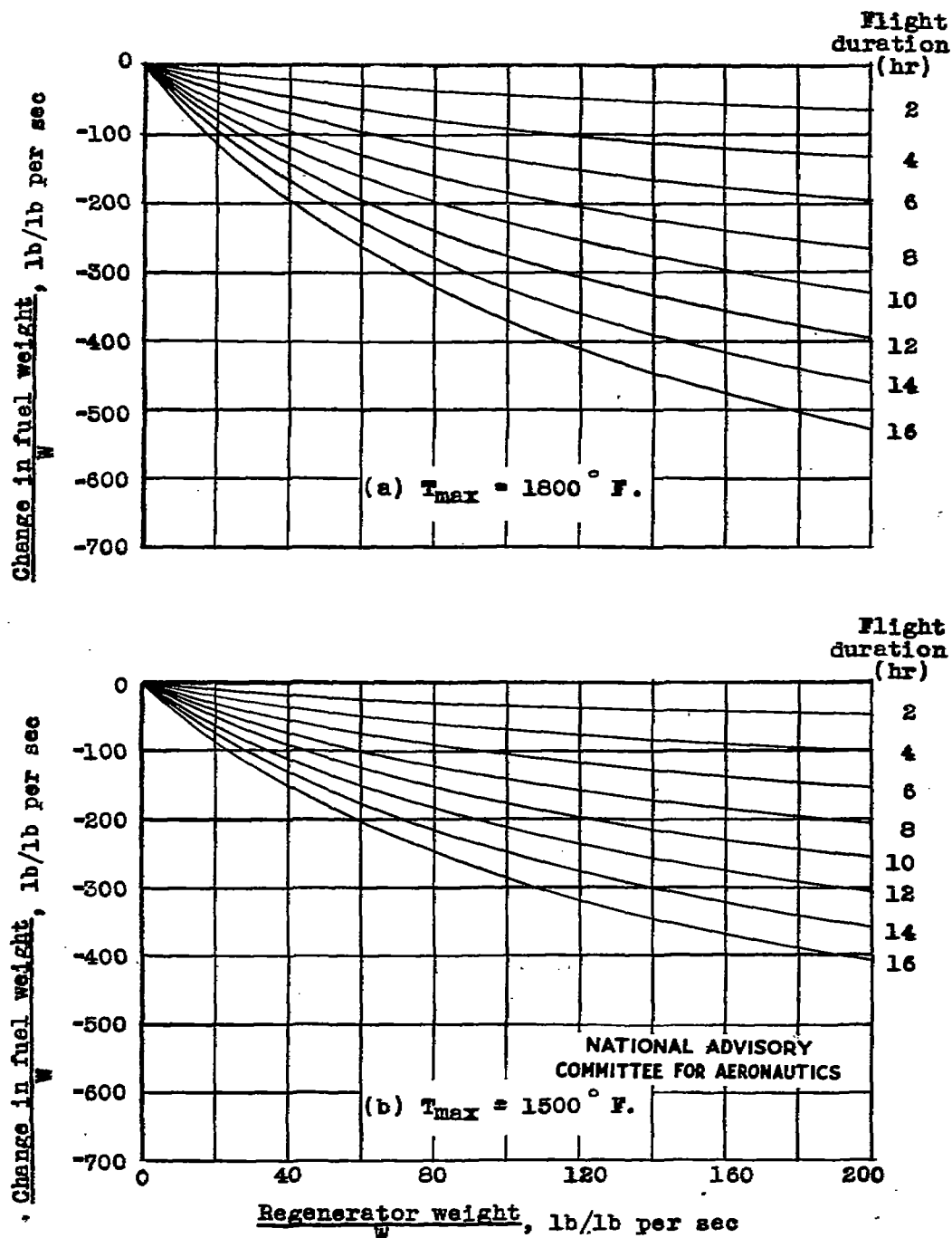
Figure 28.- Change in fuel weight per pound of air per second as a function of heat-exchanger weight per pound of air per second. Altitude, 25,000 feet; R_c = 3 ; A/W = 0.3 square foot per pound of air per second.
