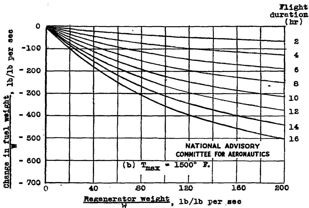
Figure 32.- Change in fuel weight per pound of air per second as a function of heat-exchanger weight per pound of air per second. Altitude, 25,000 feet; R_c = 2 ; A/W = 0.3 square foot per pound of air per second.
