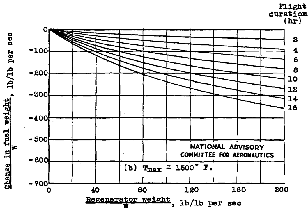
Figure 36.- Change in fuel weight per pound of air per second as a function of heat-exchanger weight per pound of air per second. Altitude, 40,000 feet; R_c = 3 ; A/W = 0.4 square foot per pound of air per second.
