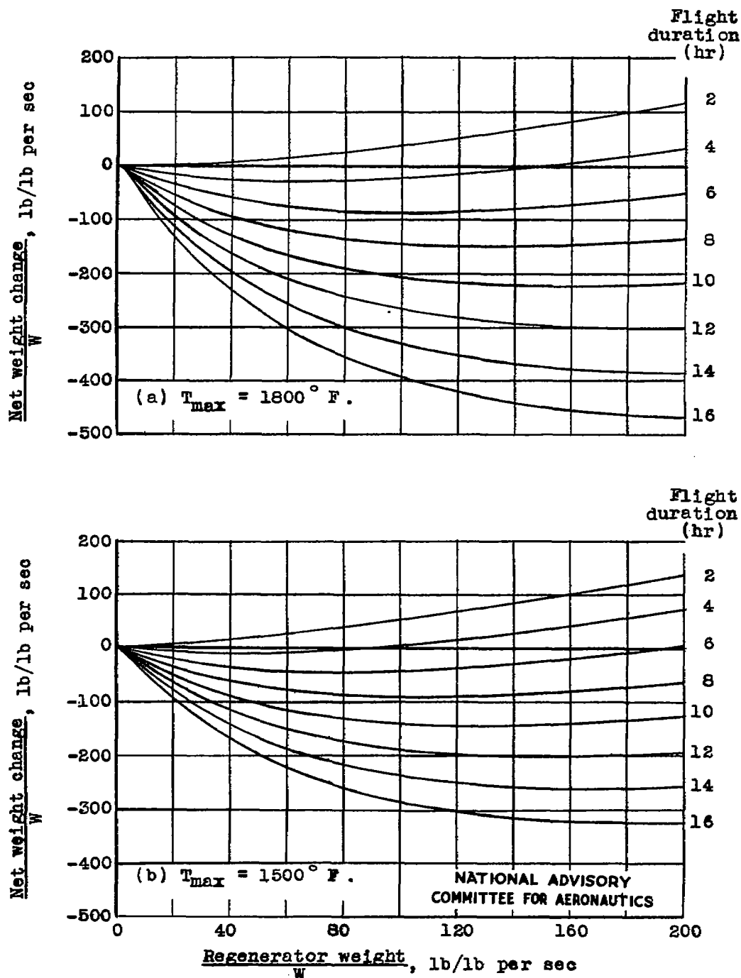
Figure 21.- Net change in weight of power plant and fuel per pound of air per second as a function of heat-exchanger weight per pound of air per second. Altitude, sea level; R_c = 2 ; A/W = 0.2 square foot per pound of air per second.
