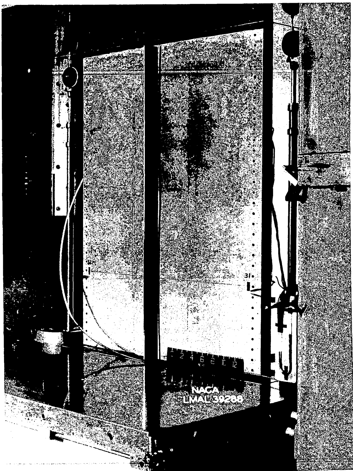
Figure 4.- Test panel under load, showing typical quilting of skin between ribs. Note shadow of straight edge.
