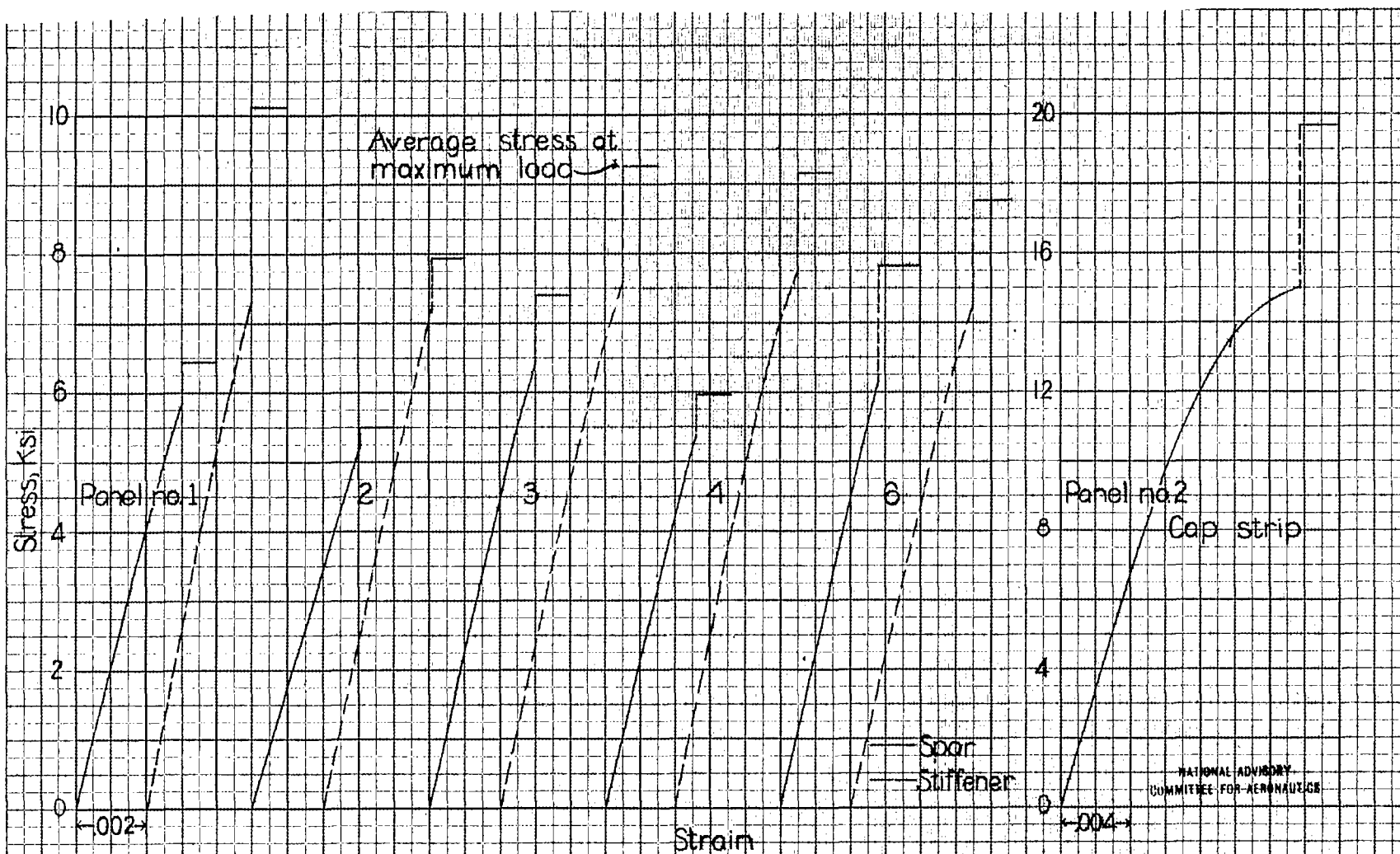
Figure 2.- Average compressive stress-strain curves for component parts of test panels. Curves for stiffeners of panels no. 1, 3, 4, and 6 include cap strip.
