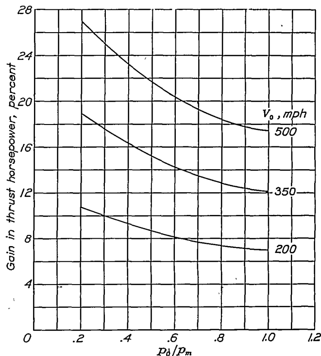
FIGURE 24.—Example of gain in thrust horsepower with exhaust-gas jet propulsion with optimum v_d n/A . Exhaust-gas flow, 0.002 pound per second per bhp; \eta_p , taken from figure 9; \eta_p , 0.85; 25-inch stack.
