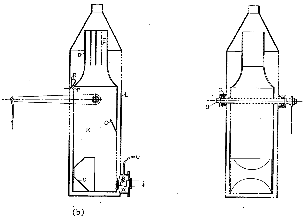
FIGURE 2.—Diagram of thrust-measuring device.
