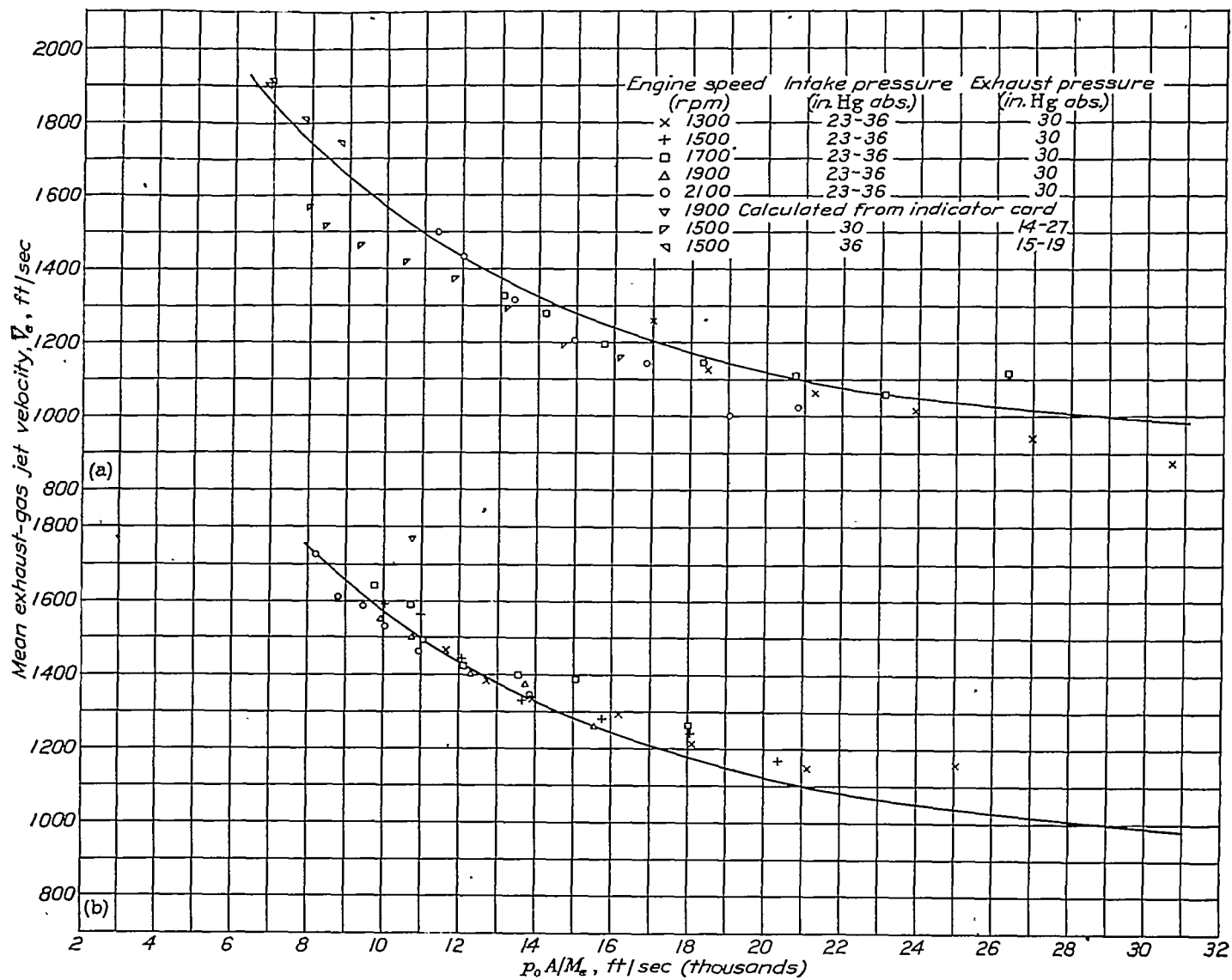
FIGURE 19.—Variation of mean exhaust-gas jet velocity \bar{V}_e with p_0 A/M_e for 25-inch stack.
