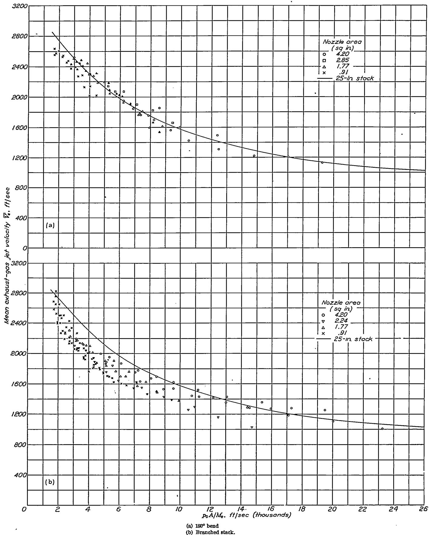
FIGURE 20.—Variation of \bar{V}_e with p_0 A / M_e .
