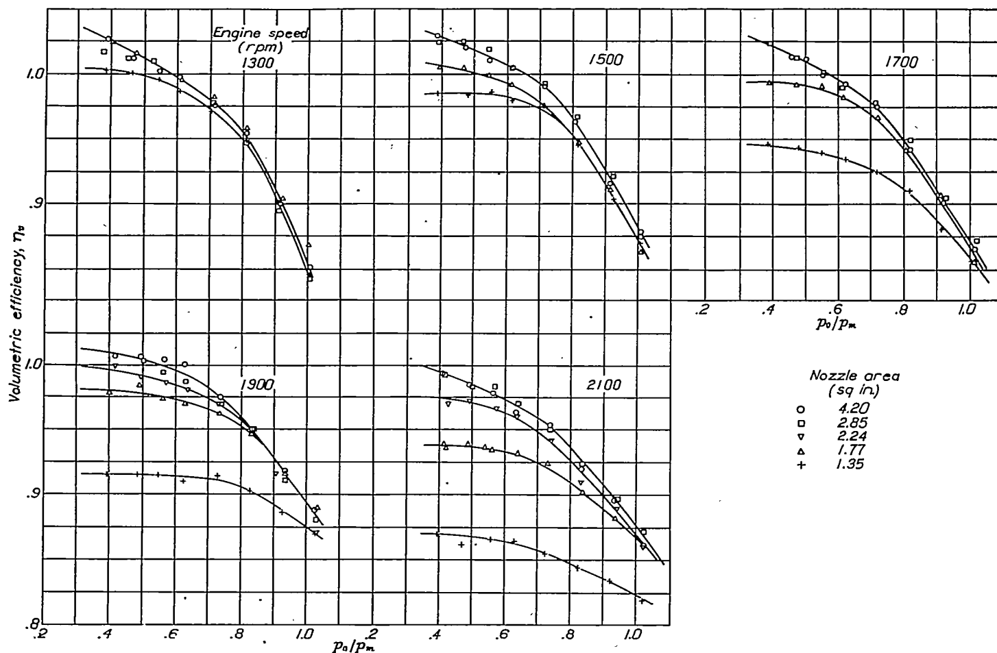
FIGURE 10.—Variation of volumetric efficiency \eta_v with p_o/p_m and nozzle area at constant engine speeds for S-shaped stack.
