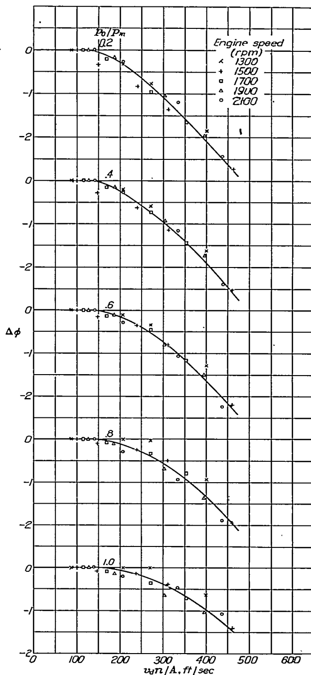
FIGURE 12.—Variation of \Delta\phi with v_2 n/A for 90° bend.
