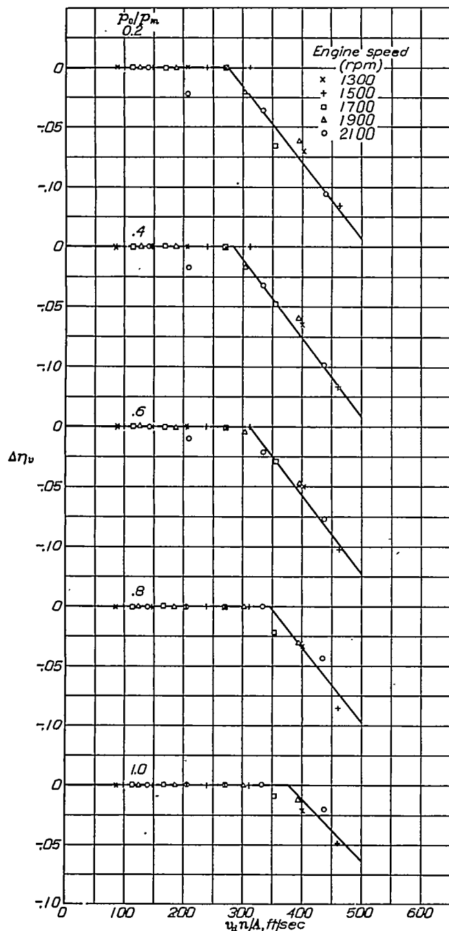
FIGURE 15.—Variation of \Delta\eta_v with v_a n/A for 90° bend.
