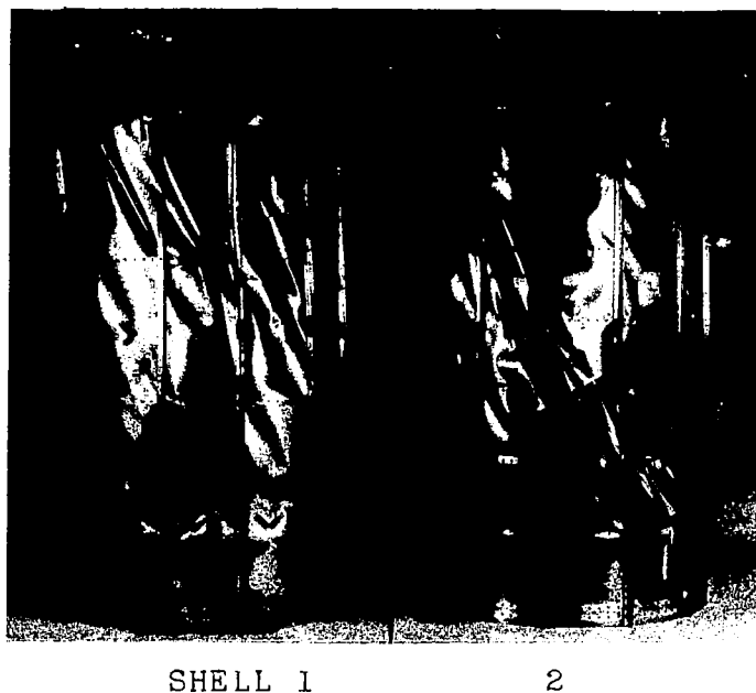
Figure 3.- Cylindrical shells 1 and 2 after failure.
