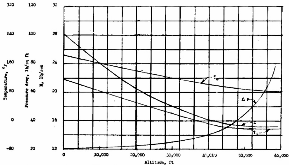
Figure 18.-Variation with altitude of M , T_1 , T_0 , and \Delta P for the 1.5-inch copper fins in high-speed flight. Army air.
