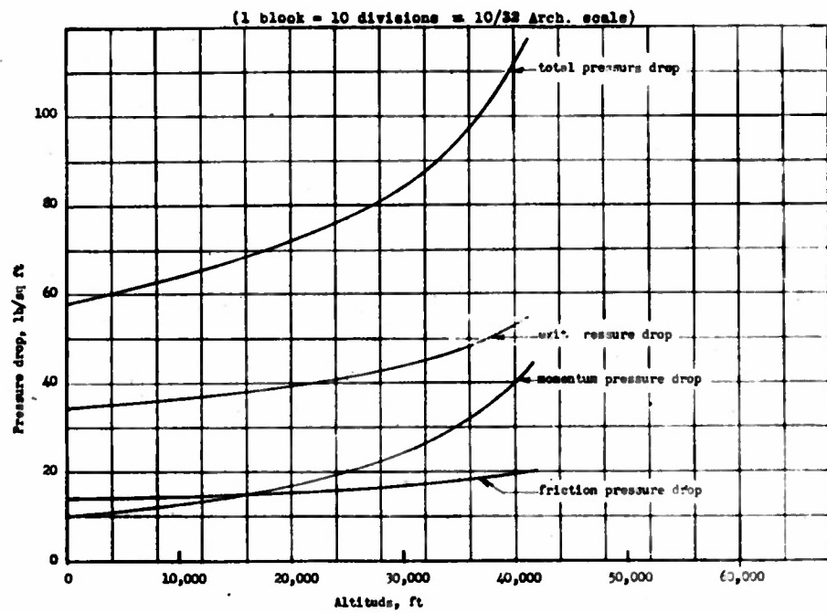
Figure 15.- Variation with altitudes of friction pressure drop, momentum pressure drop, exit pressure drop and total pressure drop for the original fins in high-speed flight. Army air.
