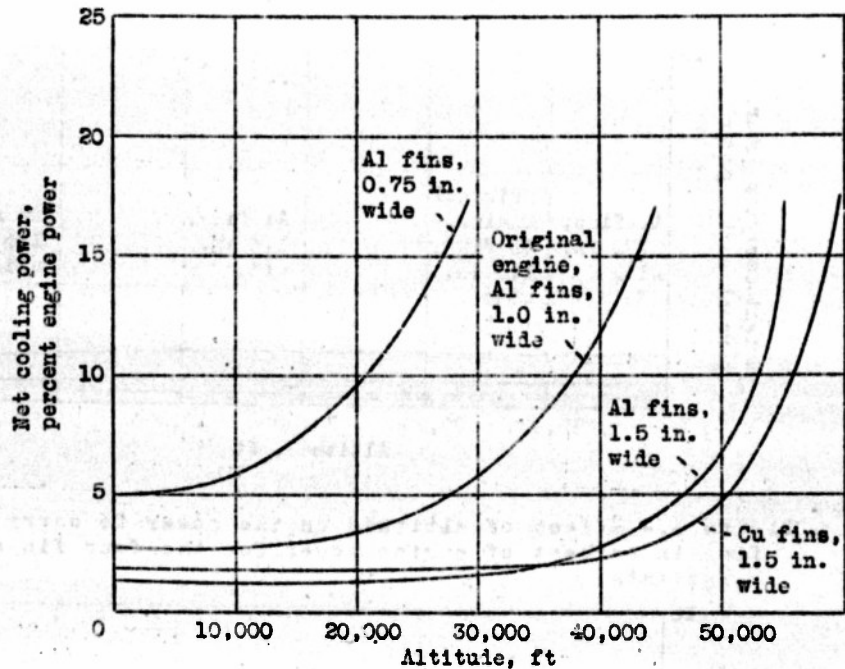
Figure 6.- Net cooling power in percent of engine power for an air-cooled engine as affected by altitude. High-speed flight condition.
