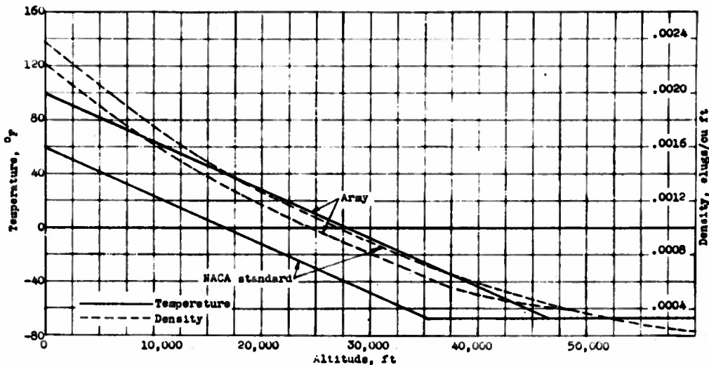
Figure 12.- Variation of temperature and density with altitudes for NACA standard air and Army air.
