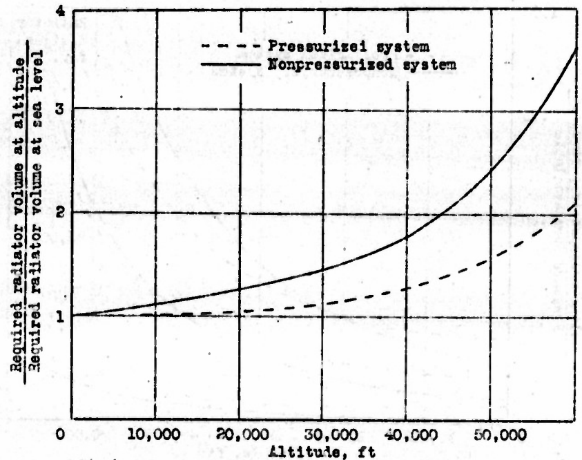
Figure 7.- Variation of required optimum radiator volume with altitude. Liquid-cooled engine; high-speed flight condition.
