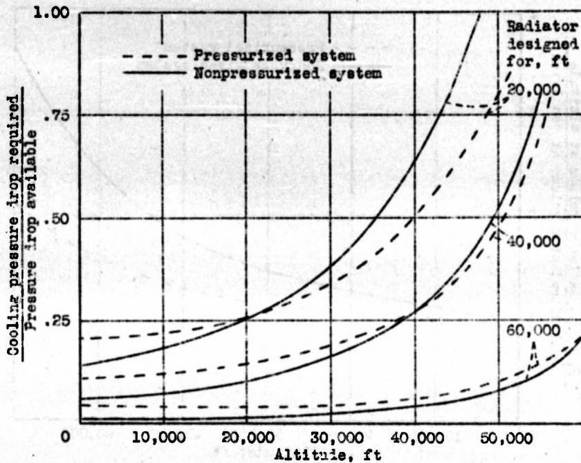
Figure 8.- The effect of altitude on the ratio of cooling pressure drop required to pressure drop available for the liquid-cooled engine. High-speed flight condition.
