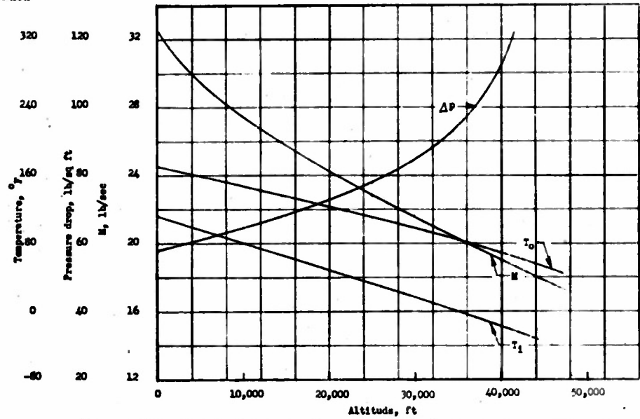
Figure 14.- Variation with altitudes of M , T_i , T_e , and \Delta p for the original fins in high-speed flight. Army air.
