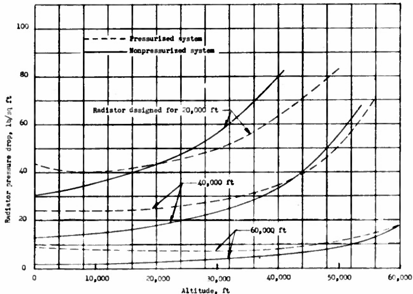
Figure 29.- Variation with altitude of pressure drop through radiators of optimum design for 20,000, 40,000, and 60,000 feet. Army air.
