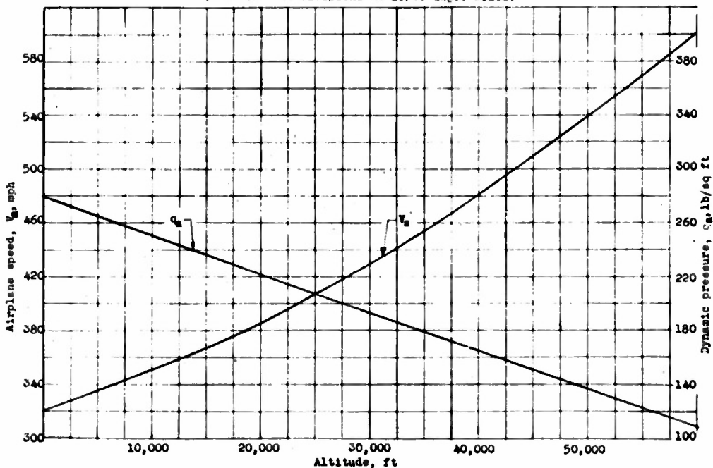
Figure 13.- Variation of speed and dynamic pressure with altitudes for a modern pursuit-type airplane.
