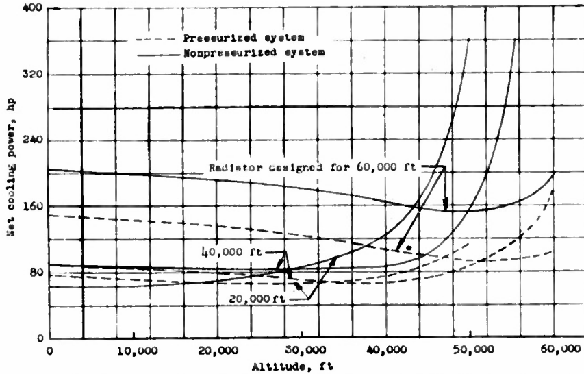
Figure 33.- Variation with altitude of the net cooling power for the three radiator installations considered. High-speed condition; Army air.
