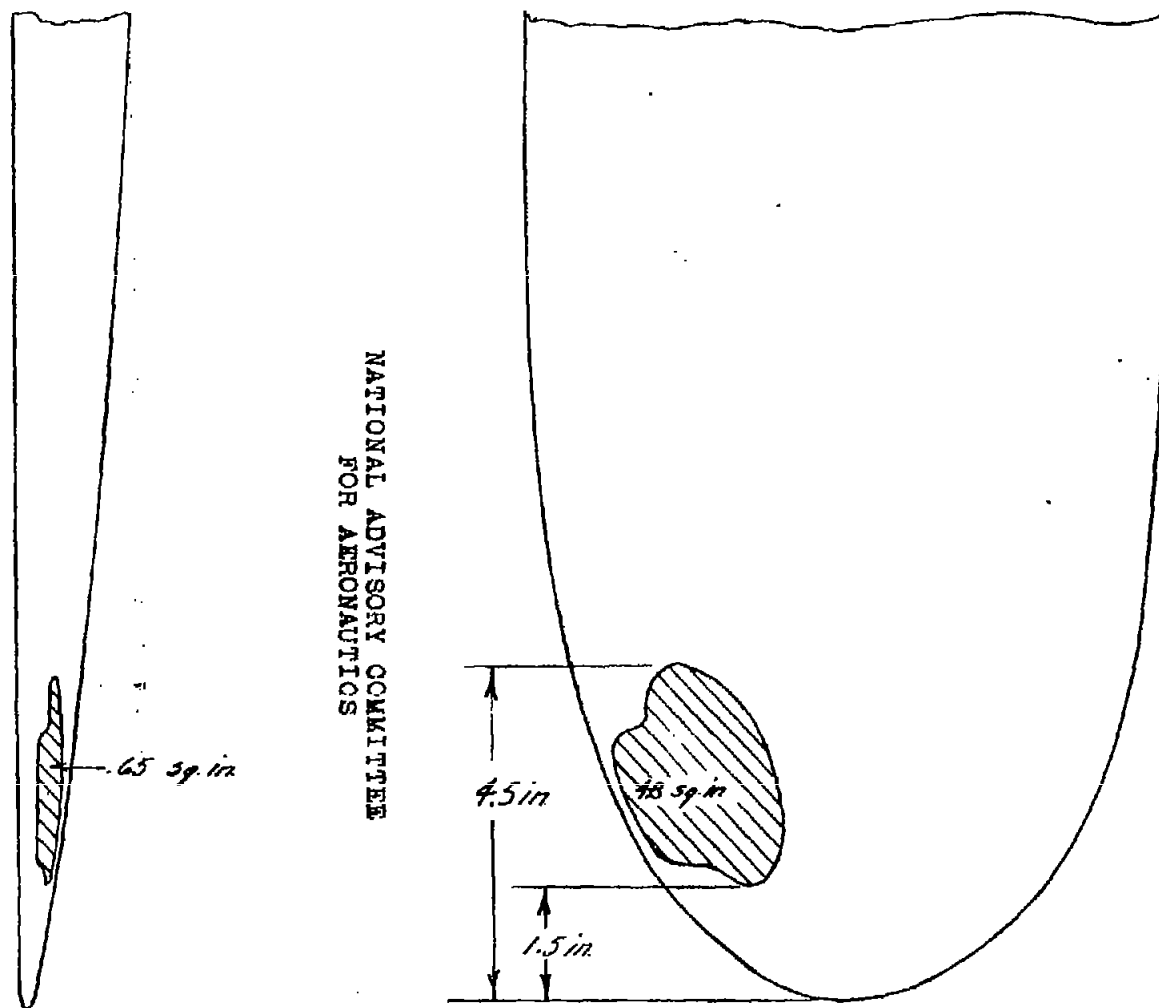
Figure 5.- Sketch of air-heated propeller-tip discharge nozzle.
