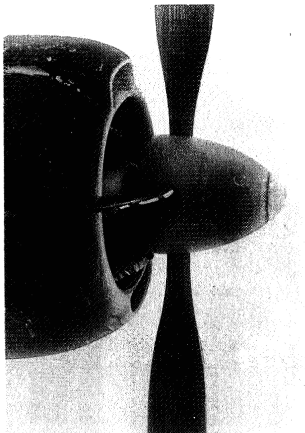
Figure 9.- Ice accretion on leading edge of air-heated propeller after flight in light-icing conditions.
