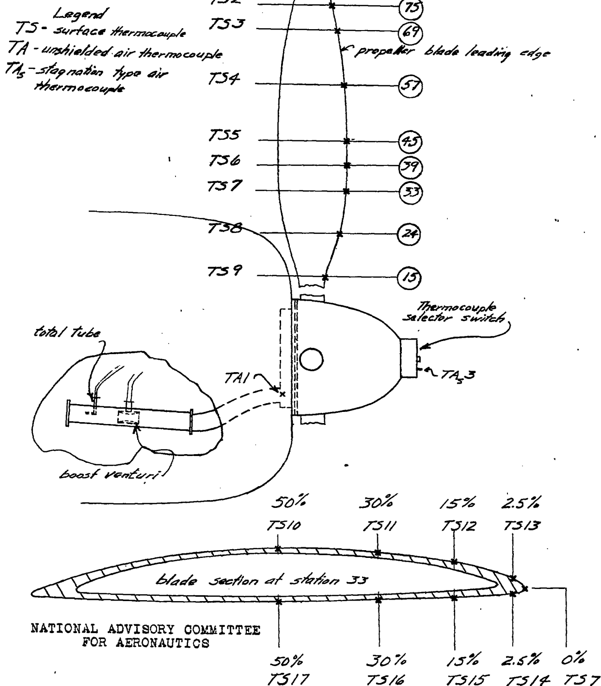
Figure 6.- Instrumentation of air-heated propeller for thermal performance tests.
