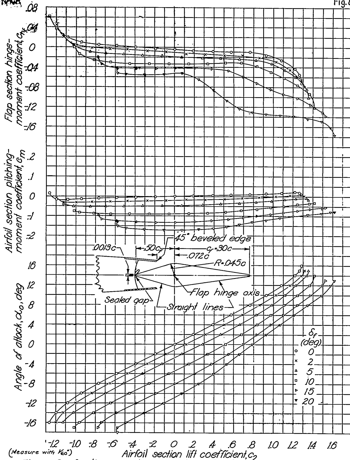
Figure 8.- Section aerodynamic characteristics of an NACA 0015 airfoil with a 0.30c straight-contour flap having a 0.50c f balance with sharp nose shape. Narrow cover plates; sealed gap.
