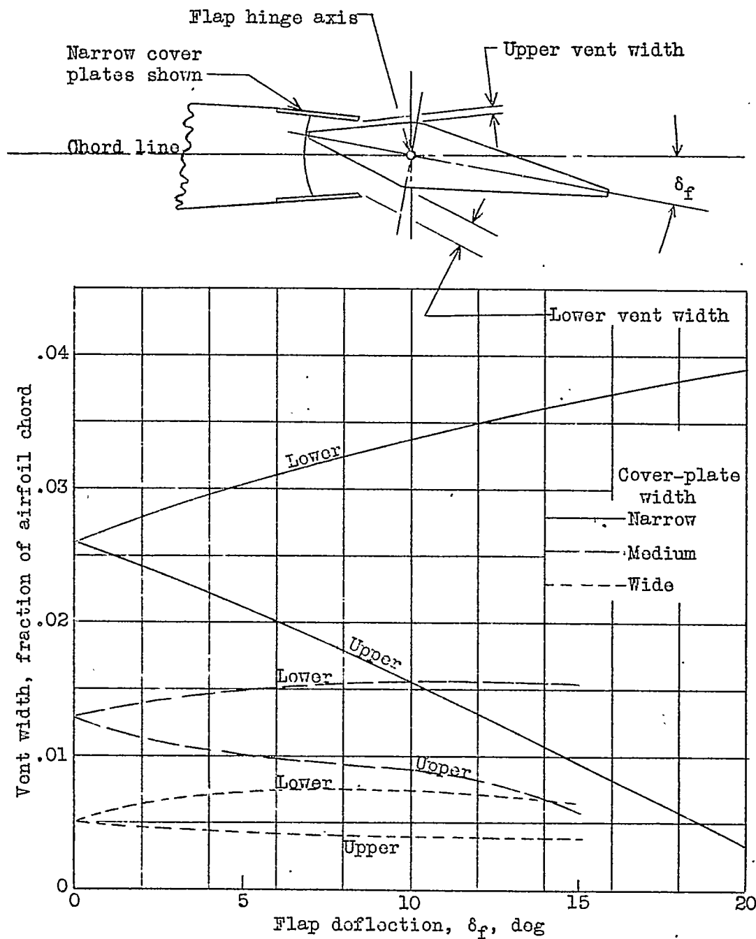
Figure 2.- Variation of upper and lower vent widths with flap deflection for the 0.30c flap with 0.50c f sharp-nose balance on the NACA 0015 airfoil.
