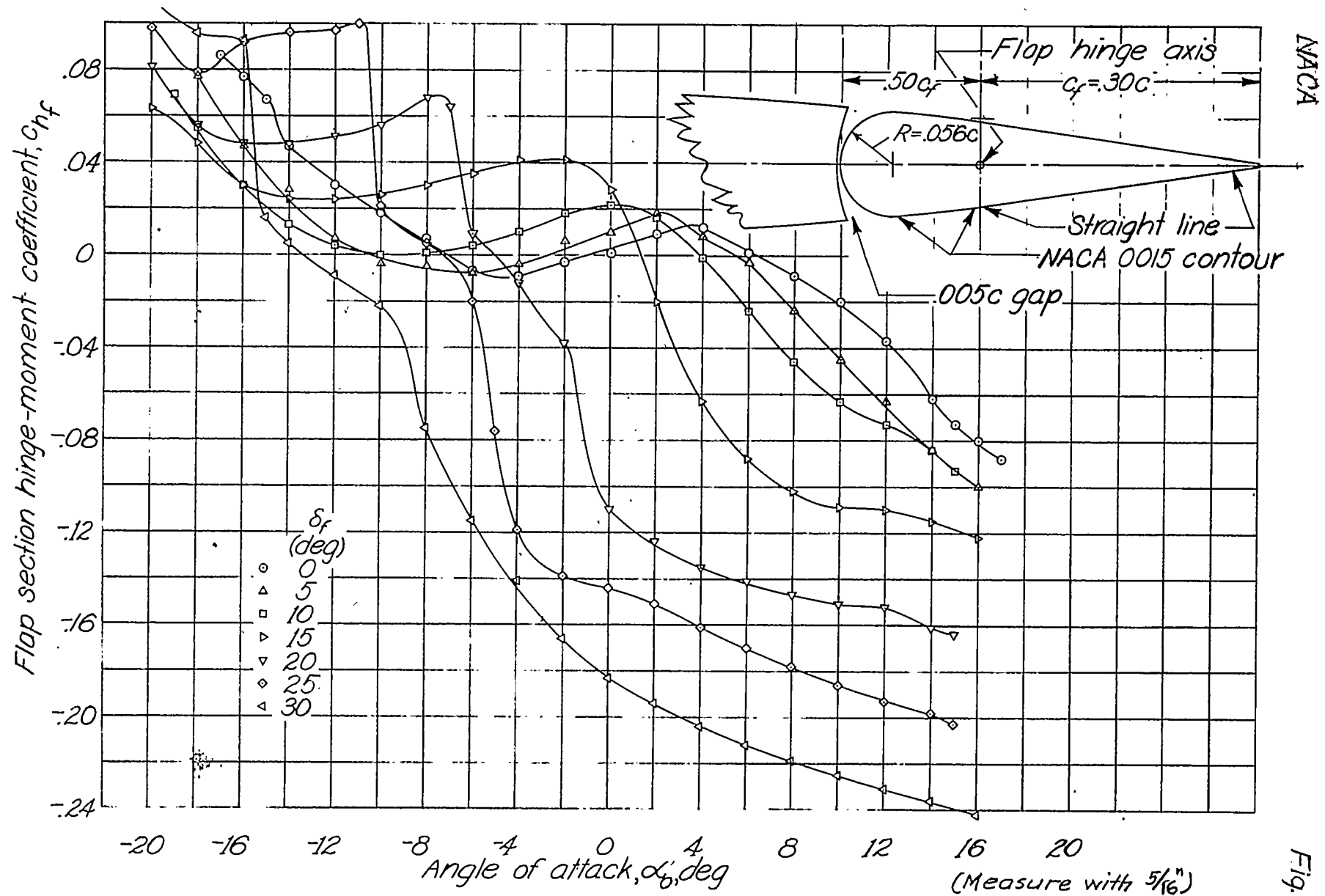
Figure 3 - Flap section hinge-moment characteristics of an NACA 0015 airfoil with a 0.30c straight-contour flap having a 0.50c_f balance with blunt nose shape. 0.005c gap.
