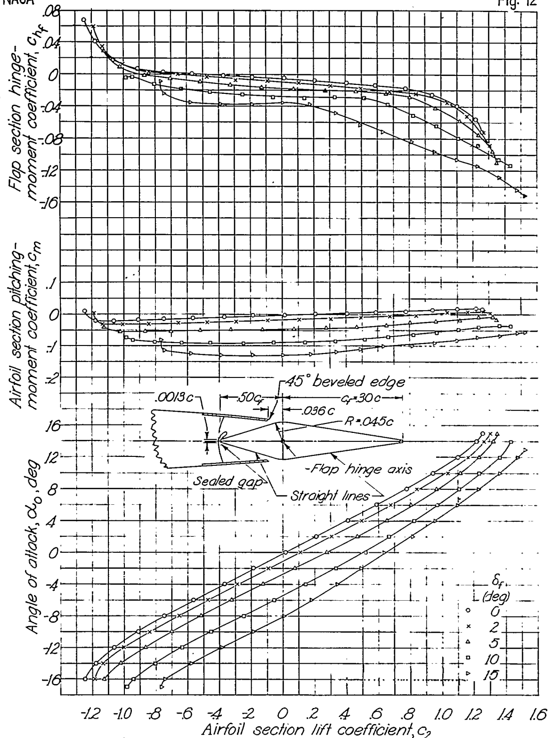
Figure 12. - Section aerodynamic characteristics of an NACA 0015 airfoil with a 0.30c straight-contour flap having a 0.50c flap balance with sharp nose shape. Medium cover plates; sealed gap
