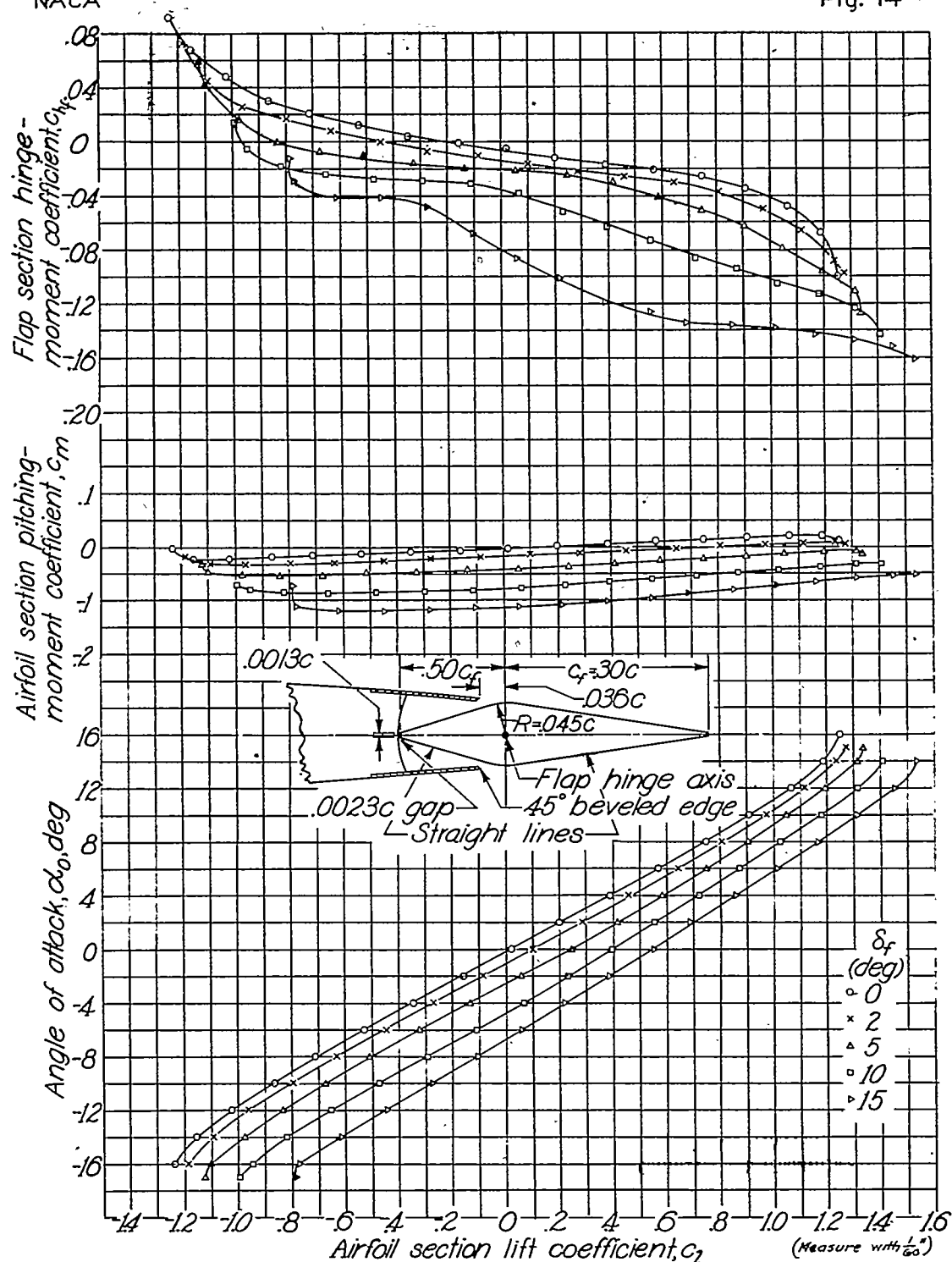
Figure 14.—Section aerodynamic characteristics of a NACA 0015 airfoil with a 0.30c straight-contour flap having a 0.50c f balance with sharp nose shape. Medium cover plates; .0023c gap.
