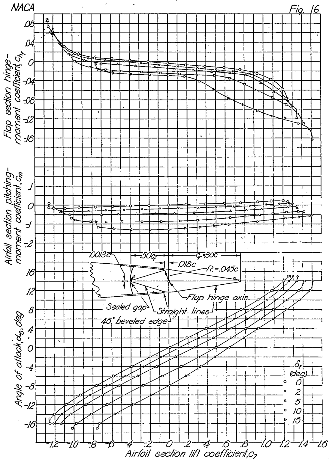
Figure 16.- Section aerodynamic characteristics of an NACA 0015 airfoil with a 0.30c straight-contour flap having a 0.50 c_f balance with sharp nose shape. Wide cover plates; sealed gap. (Measure with 1/60")
