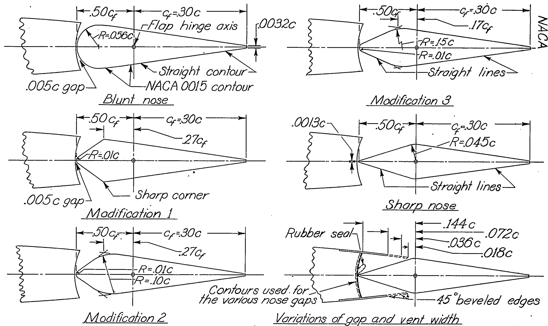
Figure 1.-Details of several 0.50c_f balances tested on the 0.30c straight-contour flap of an NACA 0015 airfoil.
