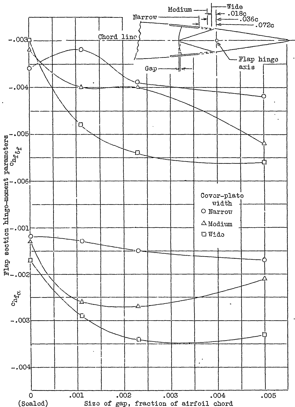
Figure 21.- Variation of flap section hinge-moment-coefficient parameters with gap size for three cover-plate widths.
