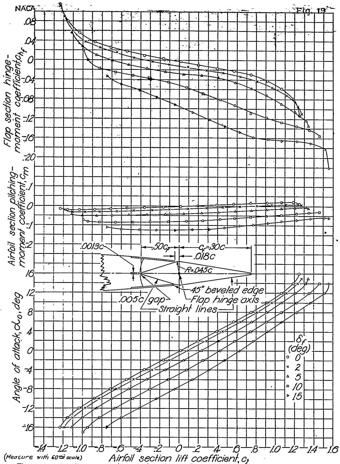
Figure 19.-Section aerodynamic characteristics of an NACA 0015 airfoil with a 0.30c straight-contour flap having a 0.50c_f balance with sharp nose shape. Wide cover plates; 0.005c gap.
