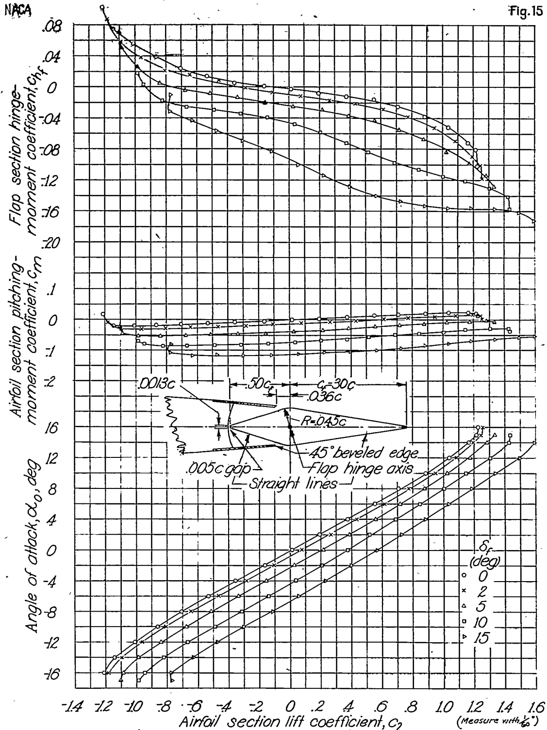
Figure 15.-Section aerodynamic characteristics of an NACA 0015 airfoil with a 0.30c straight-contour flap having a 0.50c_f balance with sharp nose shape. Medium cover plates; 0.005c gap.
