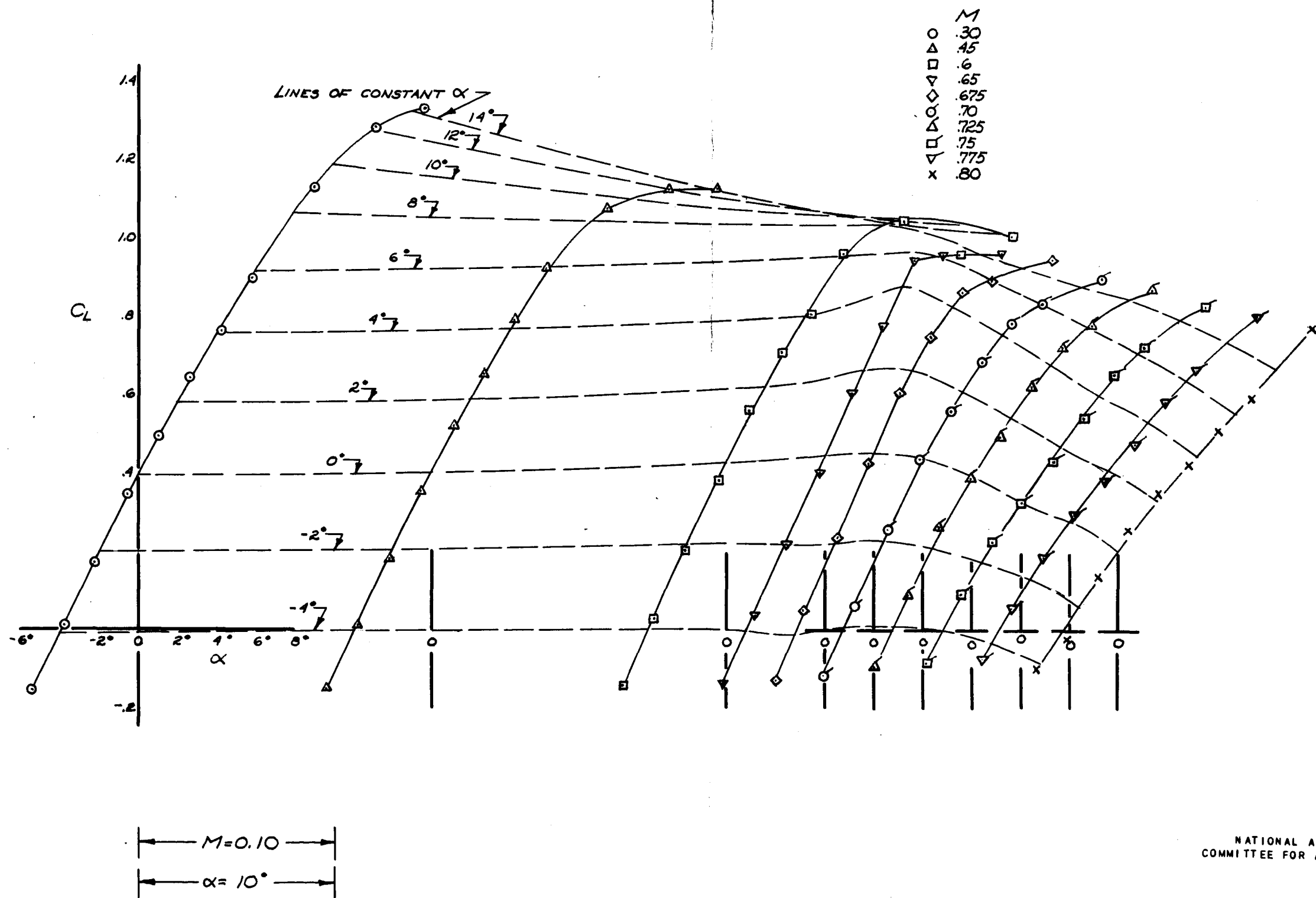
FIGURE 30.-THE LIFT COEFFICIENT FOR THE MODEL.
