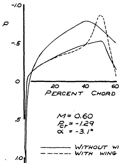
(a) M = 0.30, 0.45, 0.60, 0.65 FIGURE 16.- THE PRESSURE DISTRIBUTION AT WING STATION 12 OF THE MODEL WITH AND WITHOUT WING BUMP, AT A LIFT COEFFICIENT OF 0.1 FOR THE COMPLETE MODEL.
