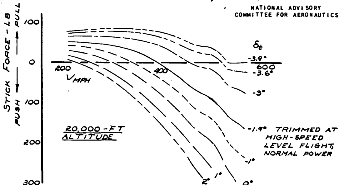
FIGURE 27.- THE STICK FORCE FOR SEVERAL TAB ANGLES FOR THE AIRPLANE WITH THE WING BUMP.
