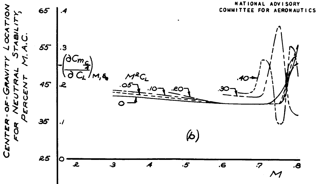
FIGURE 12.- THE EFFECT OF MACH NUMBER ON THE STICK-FIXED STABILITY CHARACTERISTICS OF THE MODEL.
