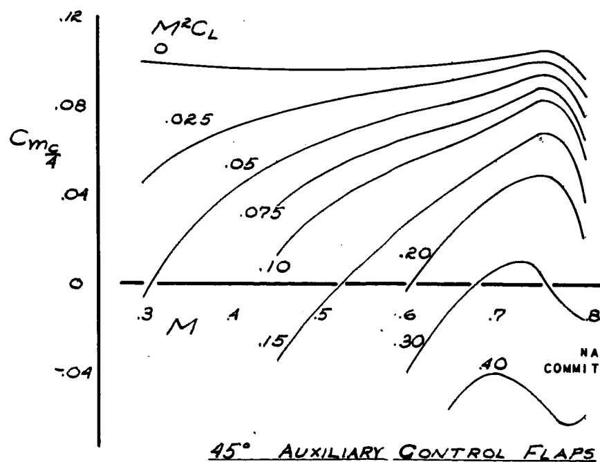
FIGURE 19.—THE STICK-FIXED STABILITY CHARACTERISTICS OF THE MODEL WITH AUXILIARY CONTROL FLAPS.
