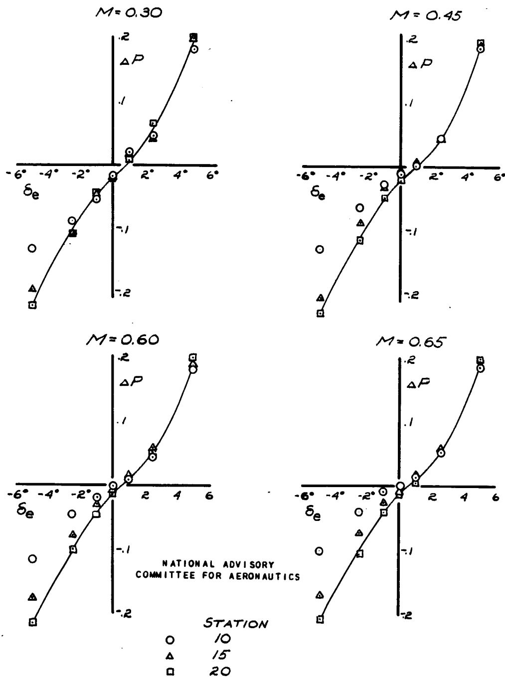
6) M = 0.30, 0.45, 0.60, 0.65 FIGURE 22.-THE ELEVATOR BALANCE PRESSURES AT THREE SPANWISE STATIONS ON THE MODEL.
