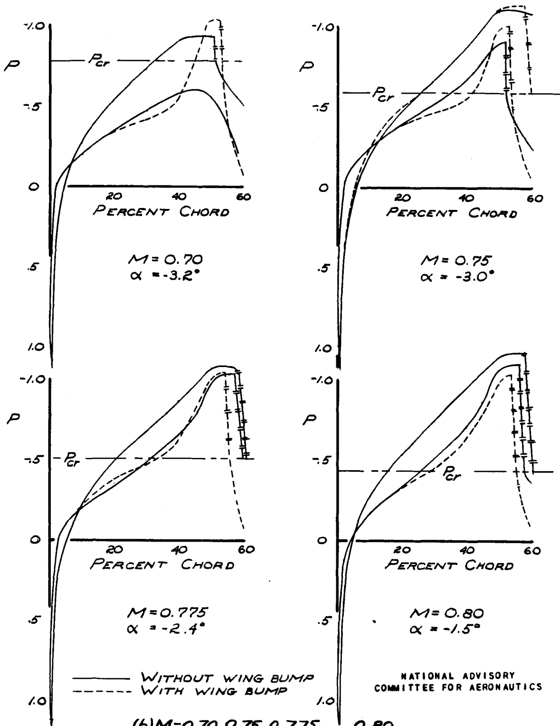
(b) M = 0.70, 0.75, 0.775, 0.80 FIGURE 16-(CONCLUDED) THE PRESSURE DISTRIBUTION AT WING STATION 12 OF THE MODEL WITH AND WITHOUT WING BUMP AT A LIFT COEFFICIENT OF 0.1 FOR THE COMPLETE MODEL.
