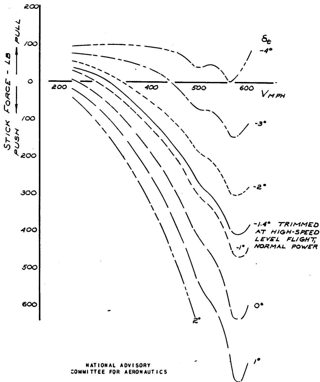
(a) SEA LEVEL FIGURE 26.-THE STICK FORCE FOR SEVERAL TAB ANGLES IN RELATION TO THE VELOCITY FOR THE AIRPLANE.
