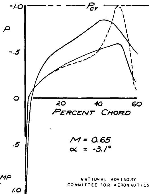
(a) M = 0.30, 0.45, 0.60, 0.65 FIGURE 16.- THE PRESSURE DISTRIBUTION AT WING STATION 12 OF THE MODEL WITH AND WITHOUT WING BUMP, AT A LIFT COEFFICIENT OF 0.1 FOR THE COMPLETE MODEL.
