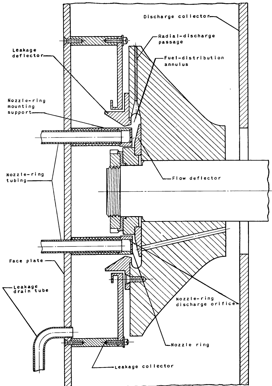
Figure 2. - Direct-flow injection-impeller installation.
