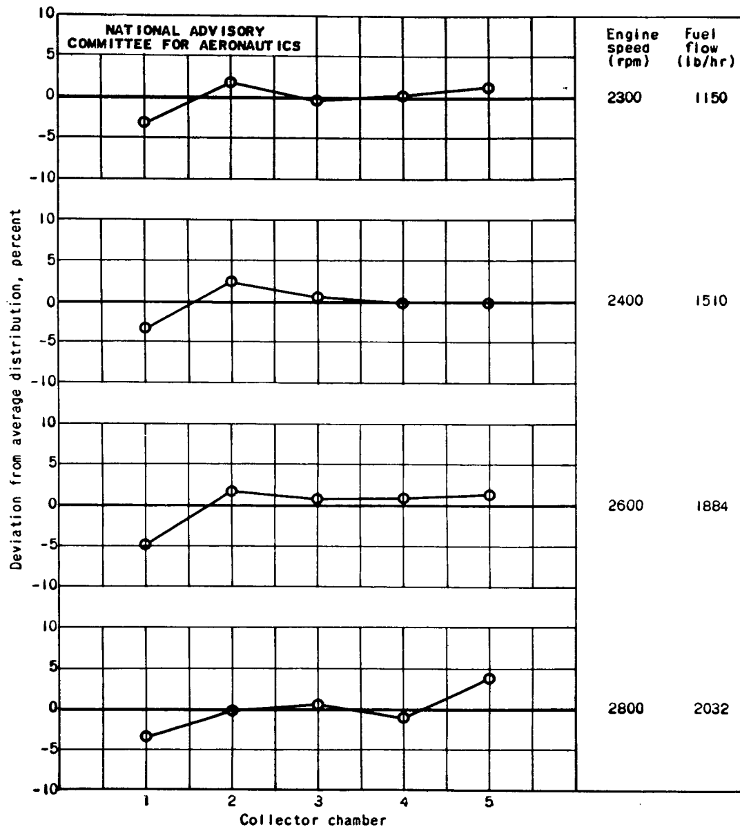
(a) Test range of engine operation. - Concluded.
