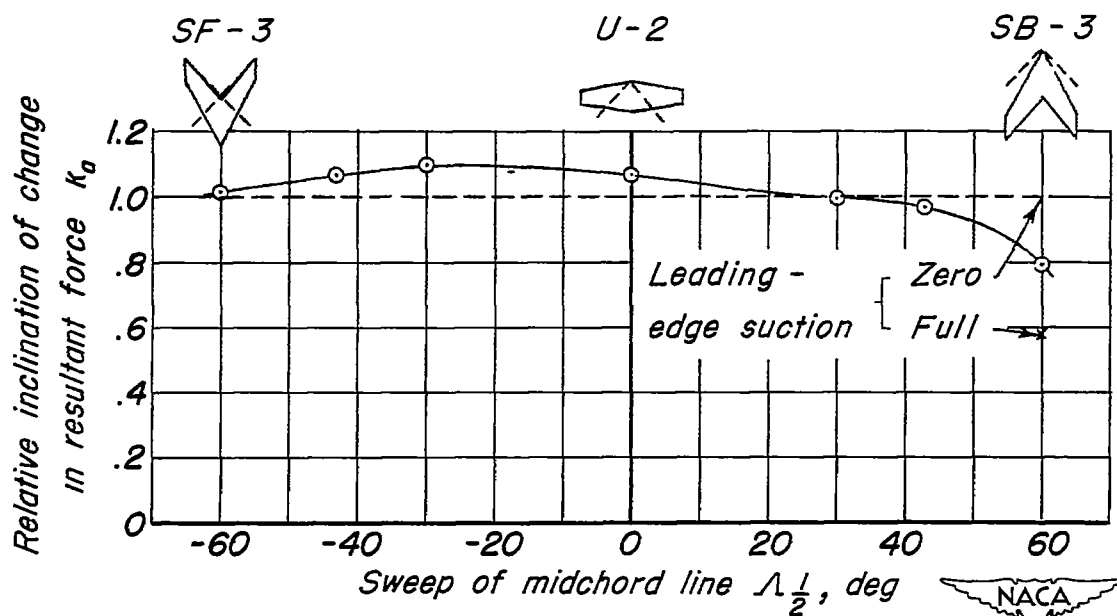
(b) Relative inclination of change in resultant force.
