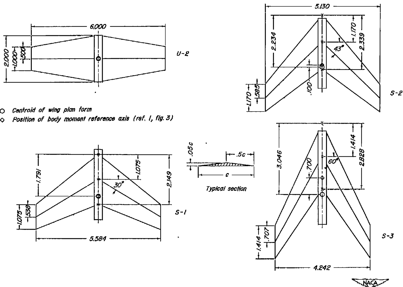
Figure 2.- Dimensions of models.
