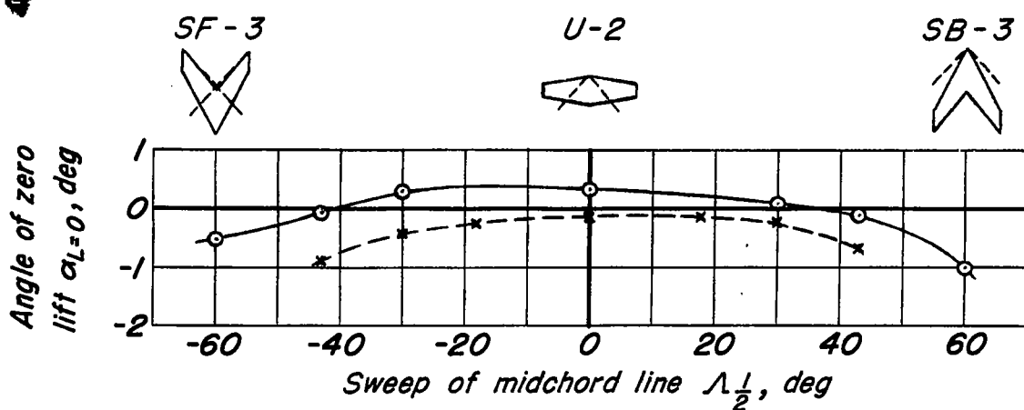
(b) Angle of zero lift.
