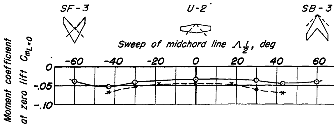
(b) Moment coefficient at zero lift.
