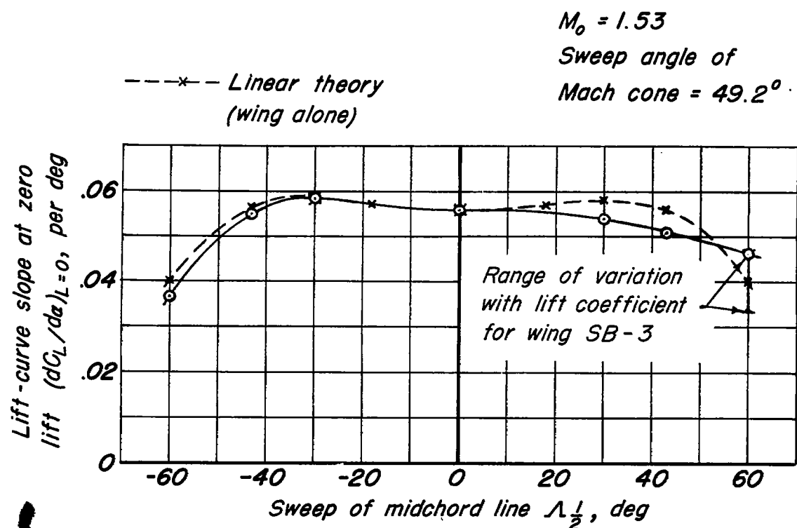
(a) Lift-curve slope.
