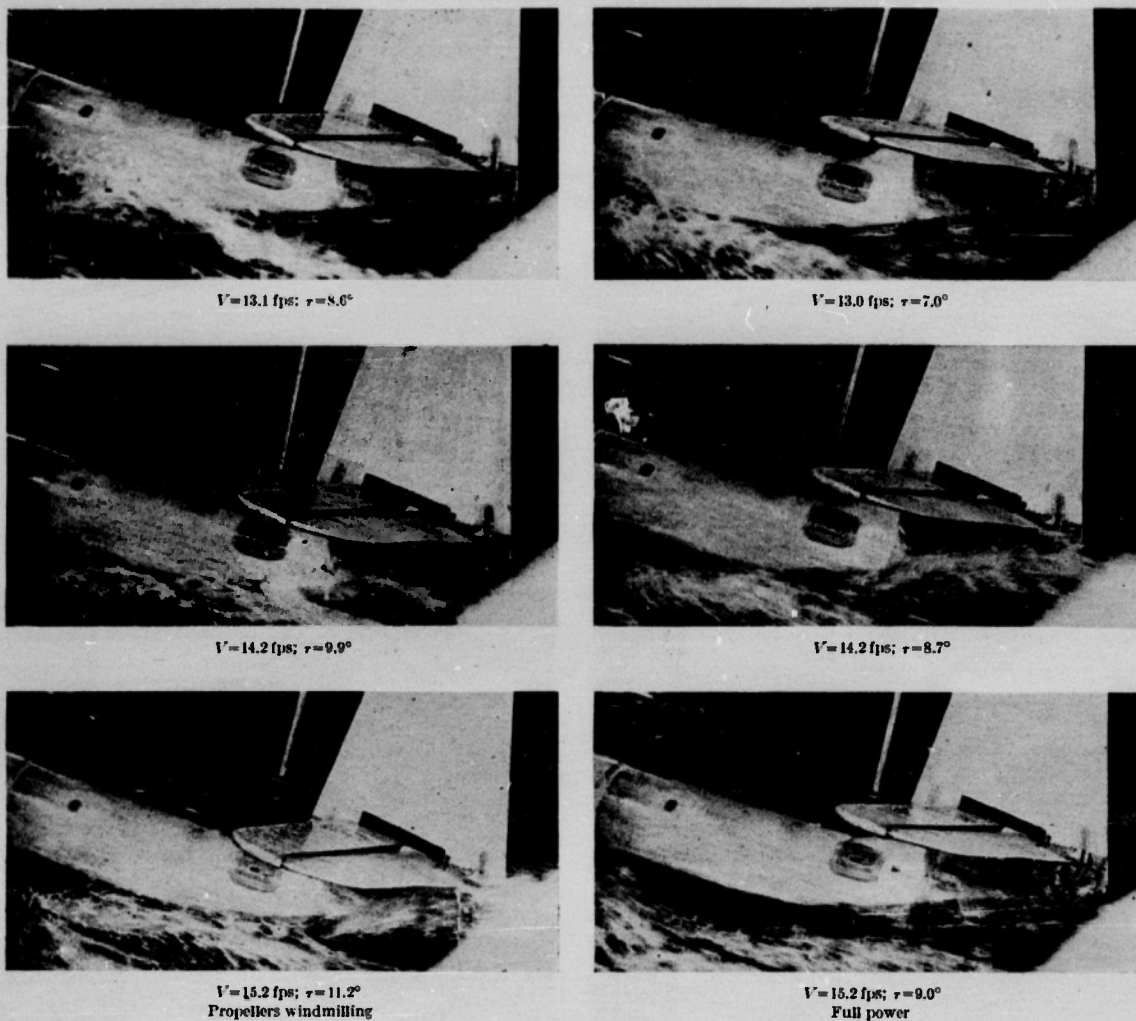
FIGURE 21.—Flow of water around afterbody and tail extension. Model 180-1; gross load, 91.3 pounds (165,000 lb, full size); \delta_a=0^\circ ; \delta_f=30^\circ ; center of gravity, 28 percent mean aerodynamic chord.
