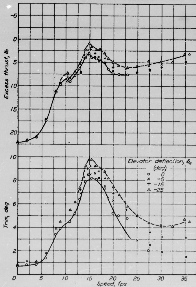
FIGURE 18.—Variation of excess thrust and trim with speed. Model 180; gross load, 54.3 pounds (165,000 lb, full size); \delta_f = 30^\circ ; center of gravity, 28 percent mean aerodynamic chord.
