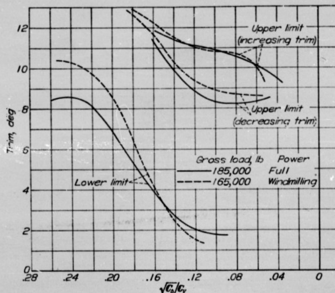
FIGURE 14.—Nondimensional trim limits of stability. Model 180-1.
