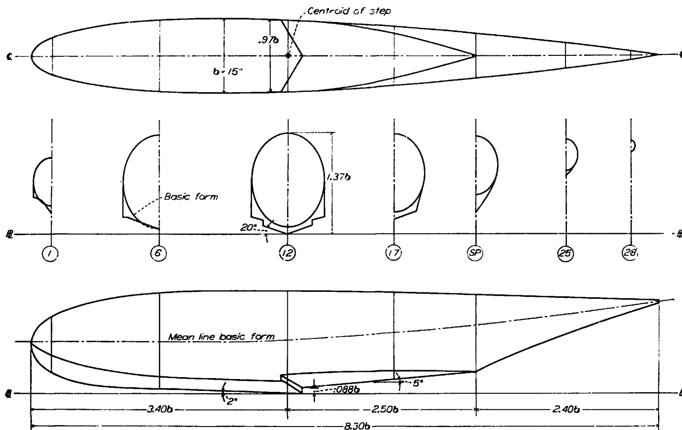
FIGURE 3.—Lines of hull. Model 180.
