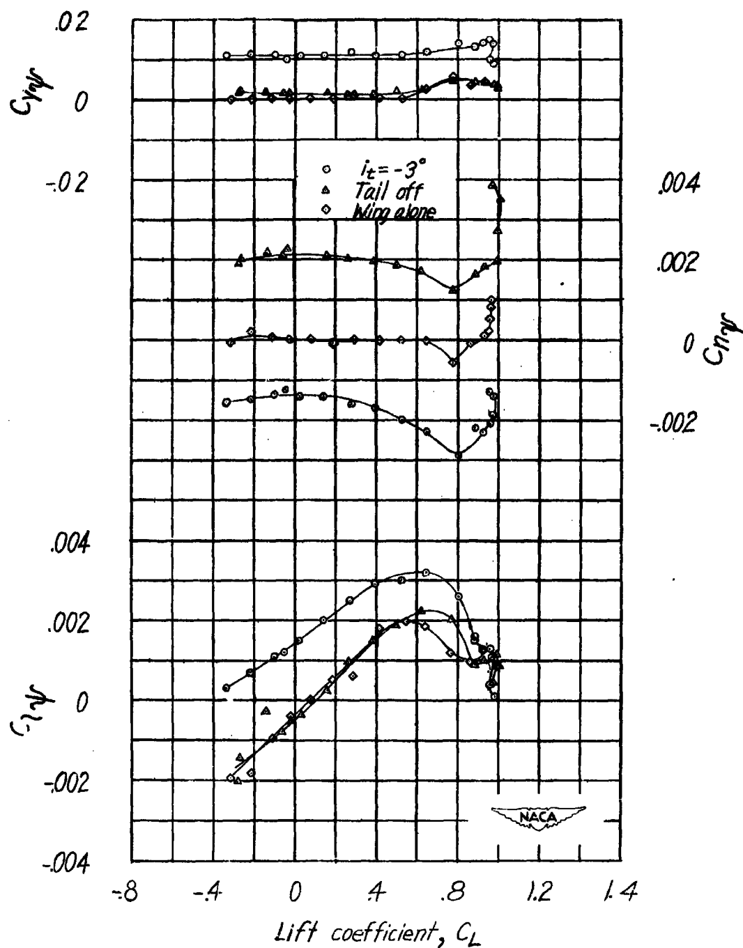
Figure 24.- Variation of lateral-stability derivatives with lift coefficient for test model. Revised dorsal; steel vertical tail; \Gamma = 0^\circ .
