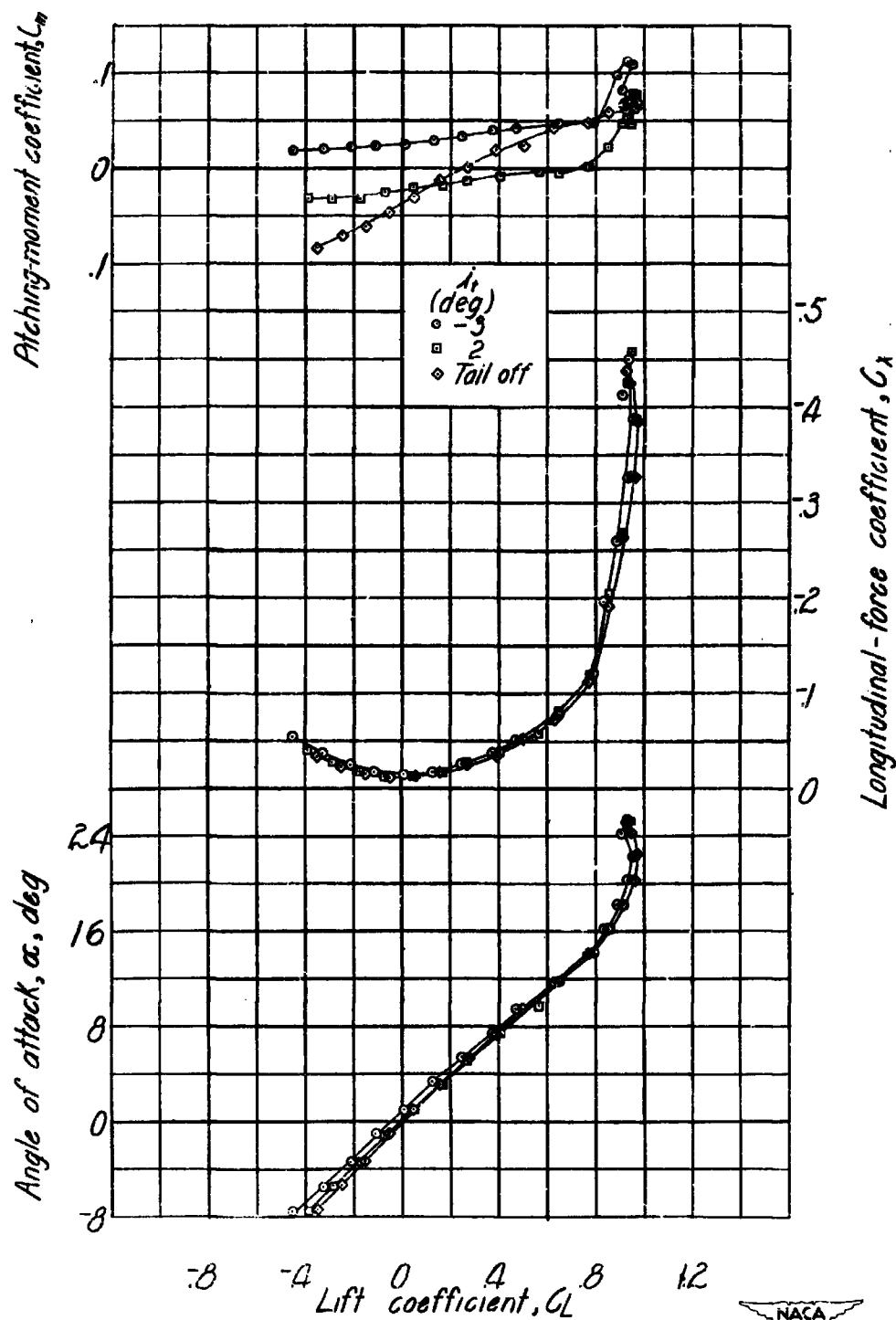
Figure 11.- Effect of stabilizer on the aerodynamic characteristics in pitch of test model. \delta_T = 0^\circ ; \psi = 0^\circ ; \Gamma = 0^\circ ; test center of gravity at 35.9 percent M.A.C.
