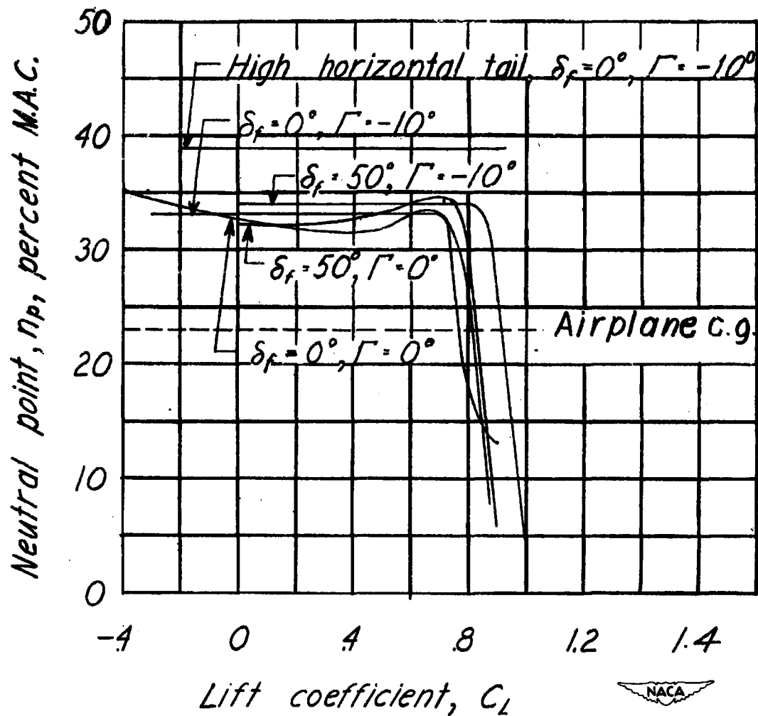
Figure 19.- Neutral points for test model.
