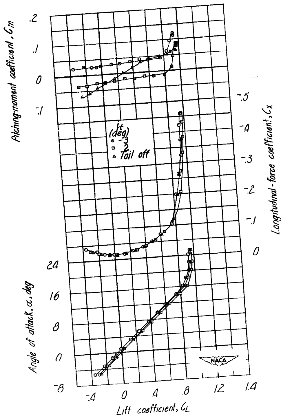
Figure 13.- Effect of stabilizer on the aerodynamic characteristics in pitch of test model. \delta r = 0^\circ ; \psi = 0^\circ ; \Gamma = -10^\circ ; test center of gravity at 35.9 percent M.A.C.
