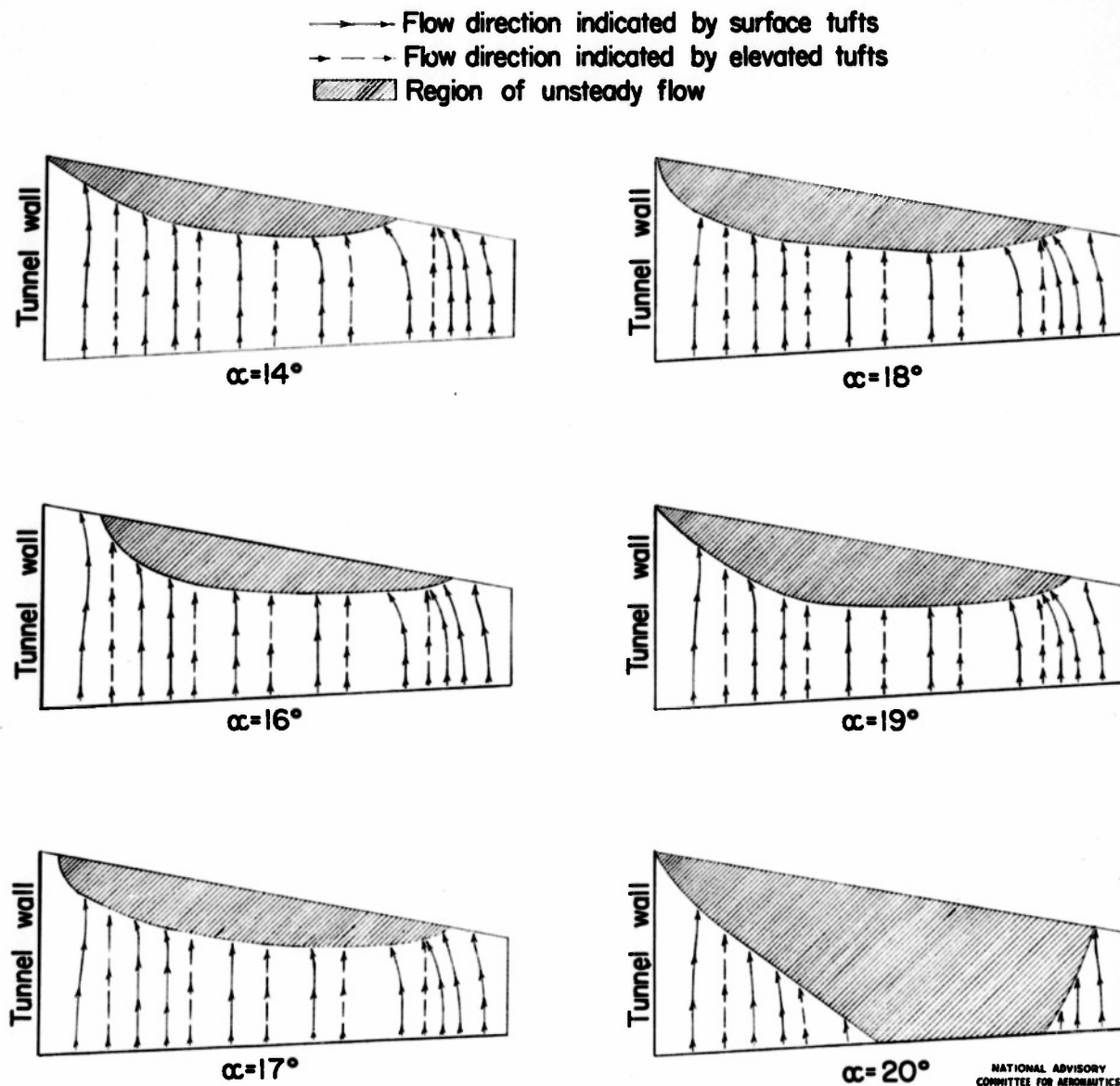
Figure 10.—Flow patterns indicated by tufts on a 65 2 -215 wing at various angles of attack. \Lambda = 0^\circ . M = .13 .
