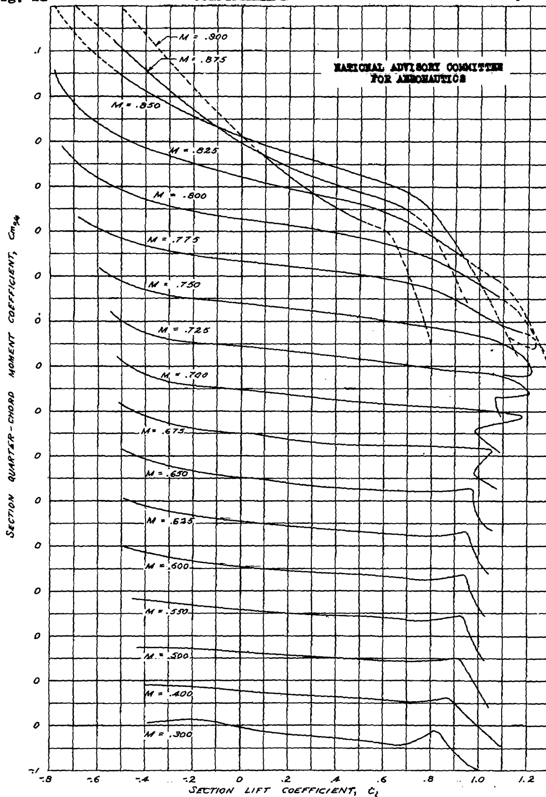
FIGURE 21. — VARIATION OF SECTION QUARTER-CHORD MOMENT COEFFICIENT WITH LIFT COEFFICIENT FOR THE NACA 65-206 AIRFOIL.
