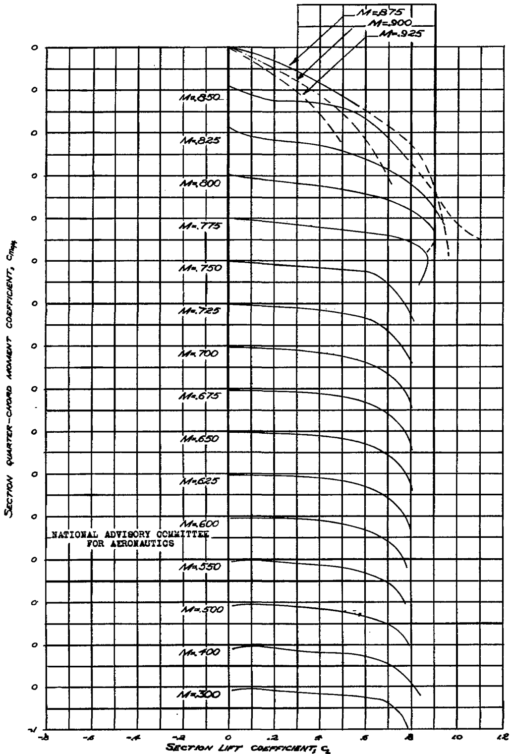
FIGURE 15.- VARIATION OF SECTION QUARTER-CHORD MOMENT COEFFICIENT WITH LIFT COEFFICIENT FOR A SYMMETRICAL DOUBLE-WEDGE AIRFOIL, \theta/c = 0.01 .
