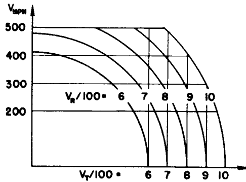
Figure 29.- Chart for evaluation of V_T .
