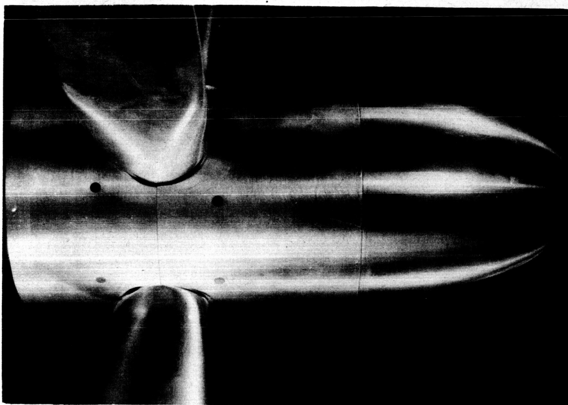
Figure 4.- Small spinner - plain blade roots.
