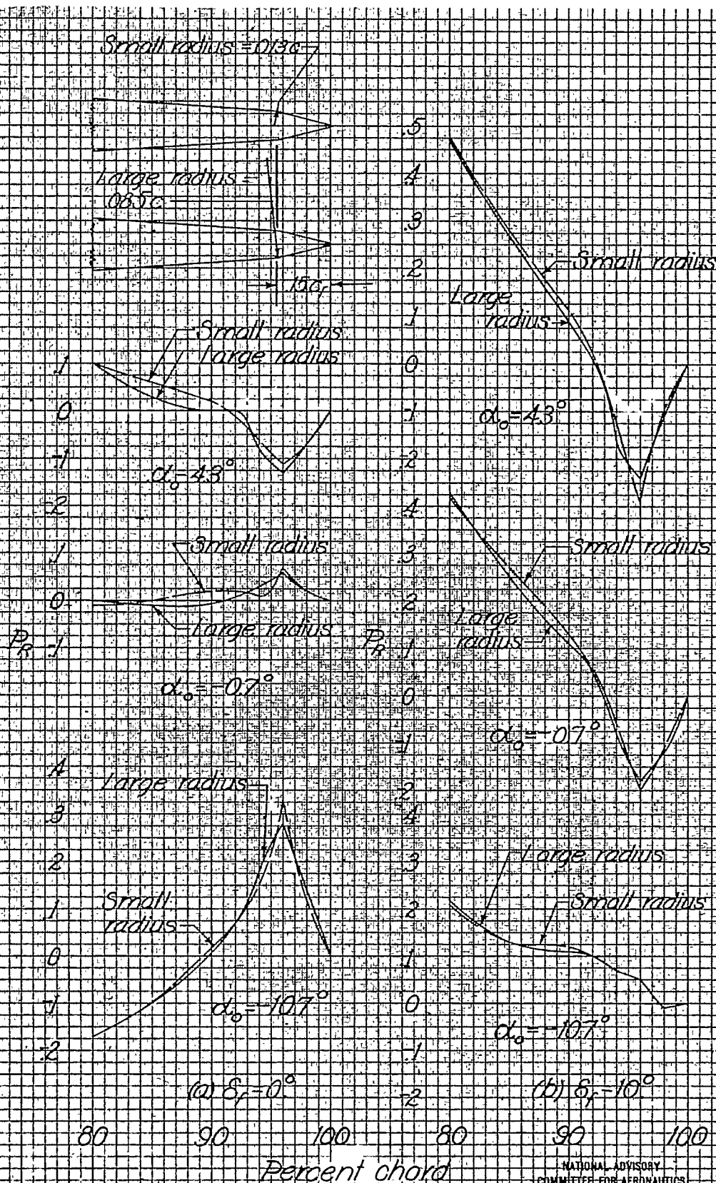
Figure 11. Comparison of resultant pressures over a 0.15c bevel with large and small radii. NACA 0009 airfoil, 0.30c flap, sealed gap.
