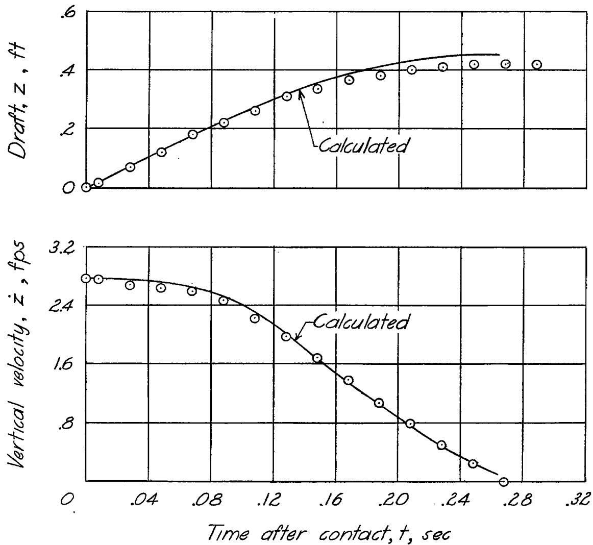
Figure 9.—Calculated and experimental time histories of vertical motion during impact of scalloped-bottom float. Smooth water; W = 1350 pounds; V_{i0} = 2.77 feet per second; V_{h0} = 55.56 feet per second; \tau = 3^\circ .
