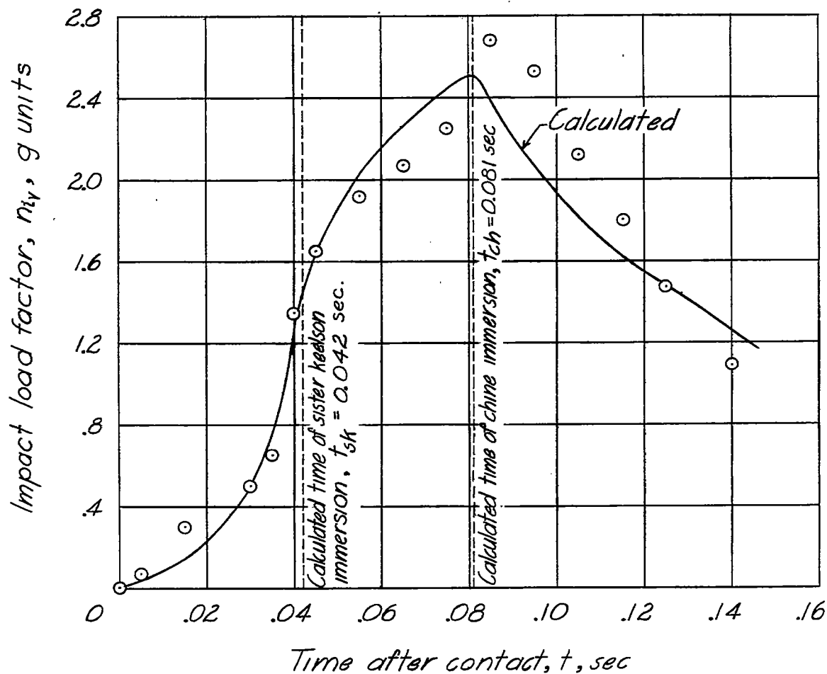
Figure 10.- Calculated and experimental time history of hydrodynamic impact load on scalloped bottom float. Smooth water; W = 1350 pounds; V_0 = 6.96 feet per second; V_{h0} = 68.75 feet per second; \tau = 7^\circ .
