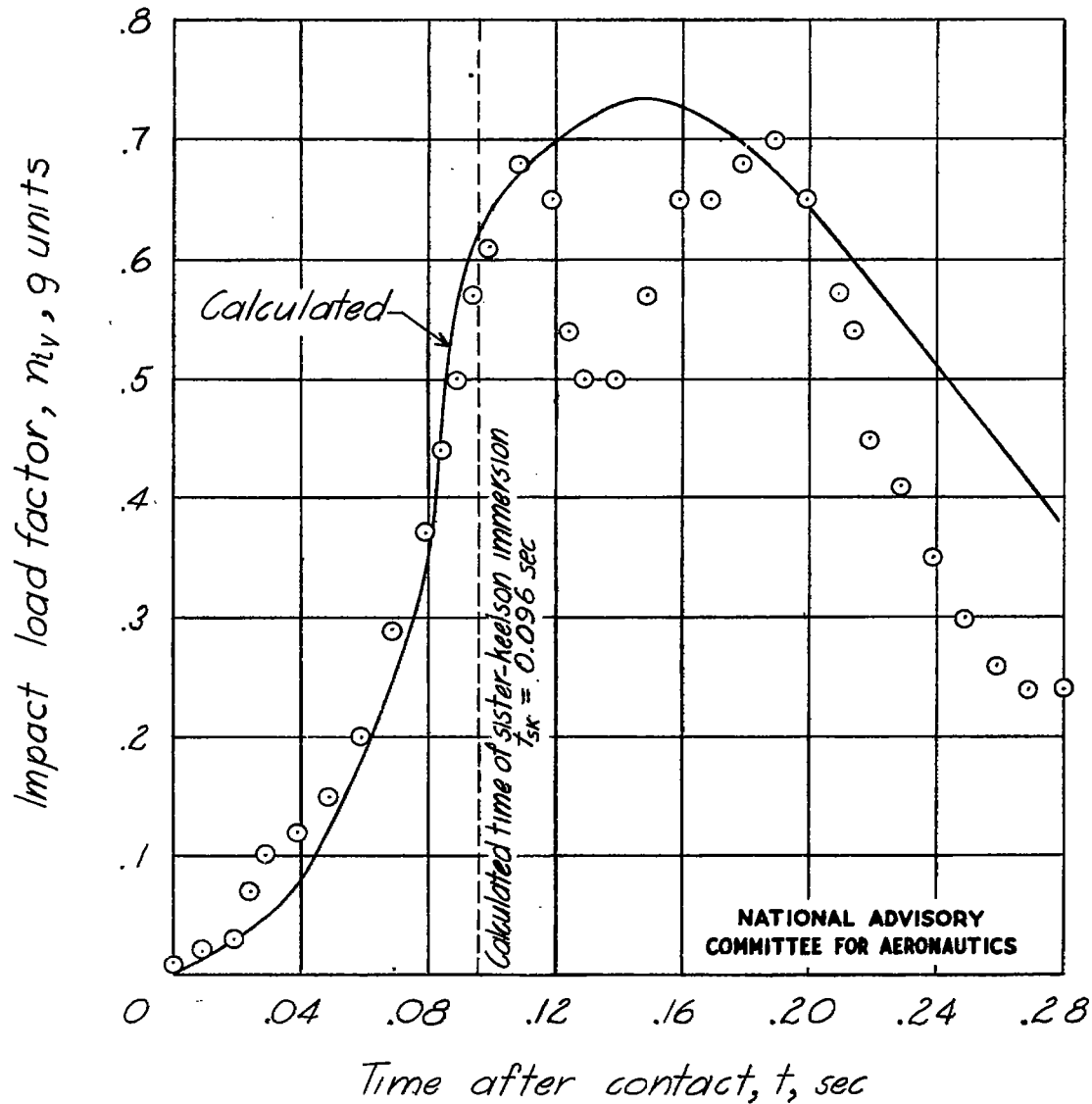
Figure 11.- Calculated and experimental time history of hydrodynamic impact load on scalloped-bottom float. Smooth water; W=1350 pounds; V_{r0}=3.04 feet per second; V_{h0}=55.2 feet per second; \tau=7^\circ .
