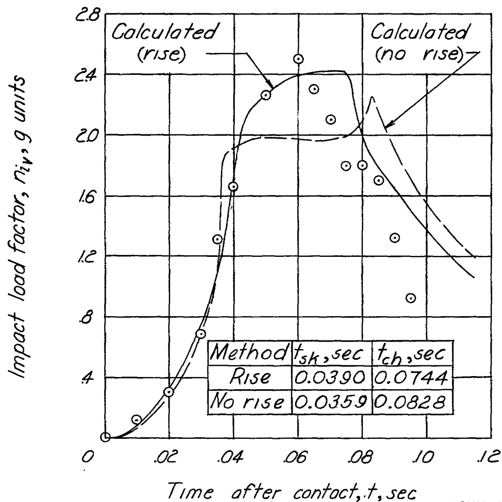
Figure 13.- Calculated and experimental time history of hydrodynamic impact load on scalloped-bottom float. Rough water; W=1350 pounds; V_{v_0}=2.91 feet per second; V_{h_0}=55.84 feet per second; \tau=7^\circ ; wave height = 2 feet; wave length = 60 feet; V_w=14.29 feet per second; \theta=4^\circ .
