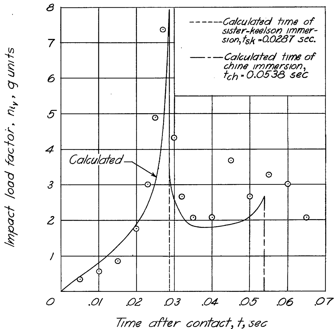
Figure 7.— Calculated and experimental time history of hydrodynamic impact load on scalloped-bottom float. Vertical impact; smooth water; W=1350 pounds; V_{r0} = 10.4 feet per second; V_{h0} = 0 feet per second; \tau = 0^\circ .
