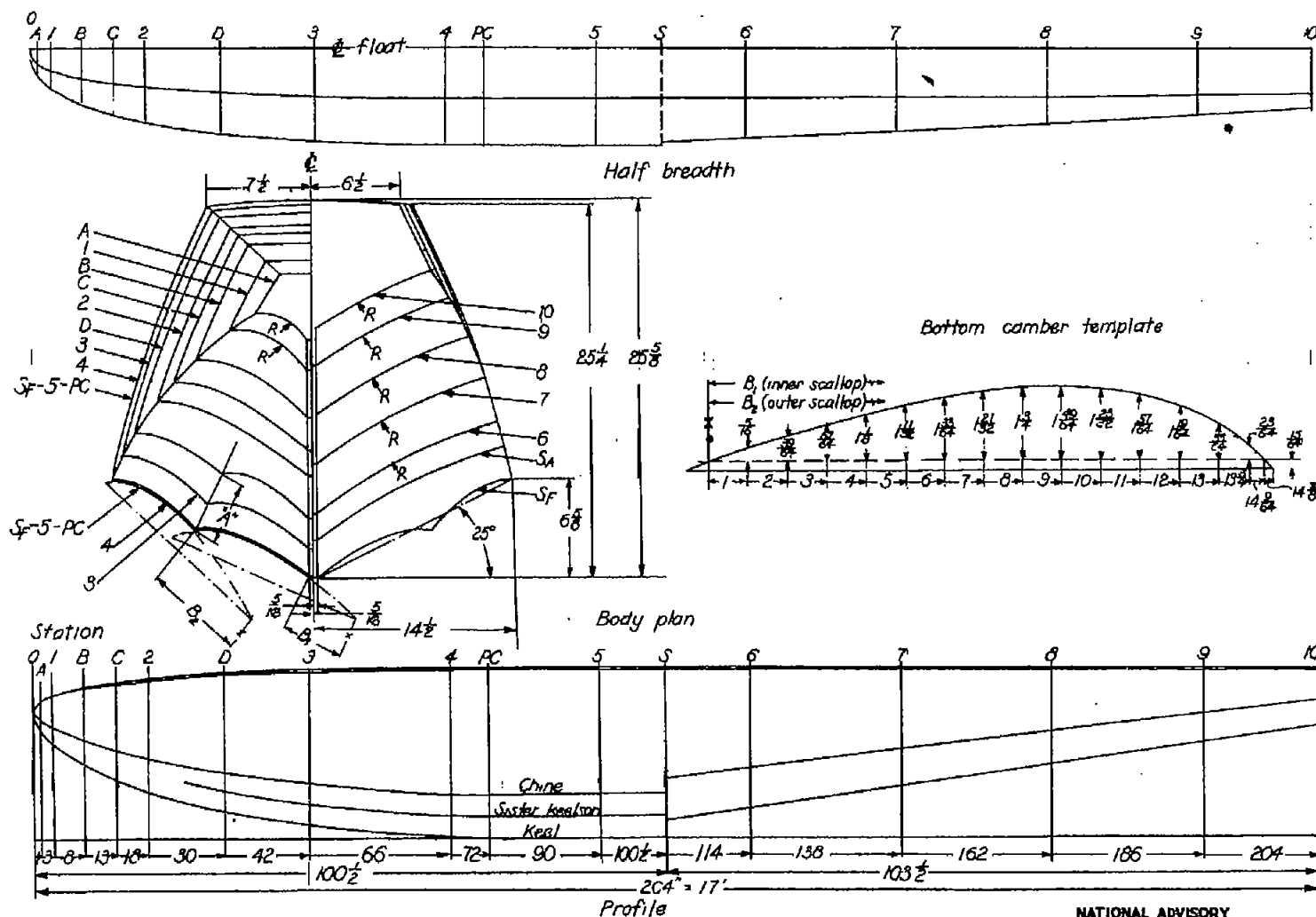
Figure 1. - Lines of scalloped-bottom seaplane float tested in Langley impact basin.
