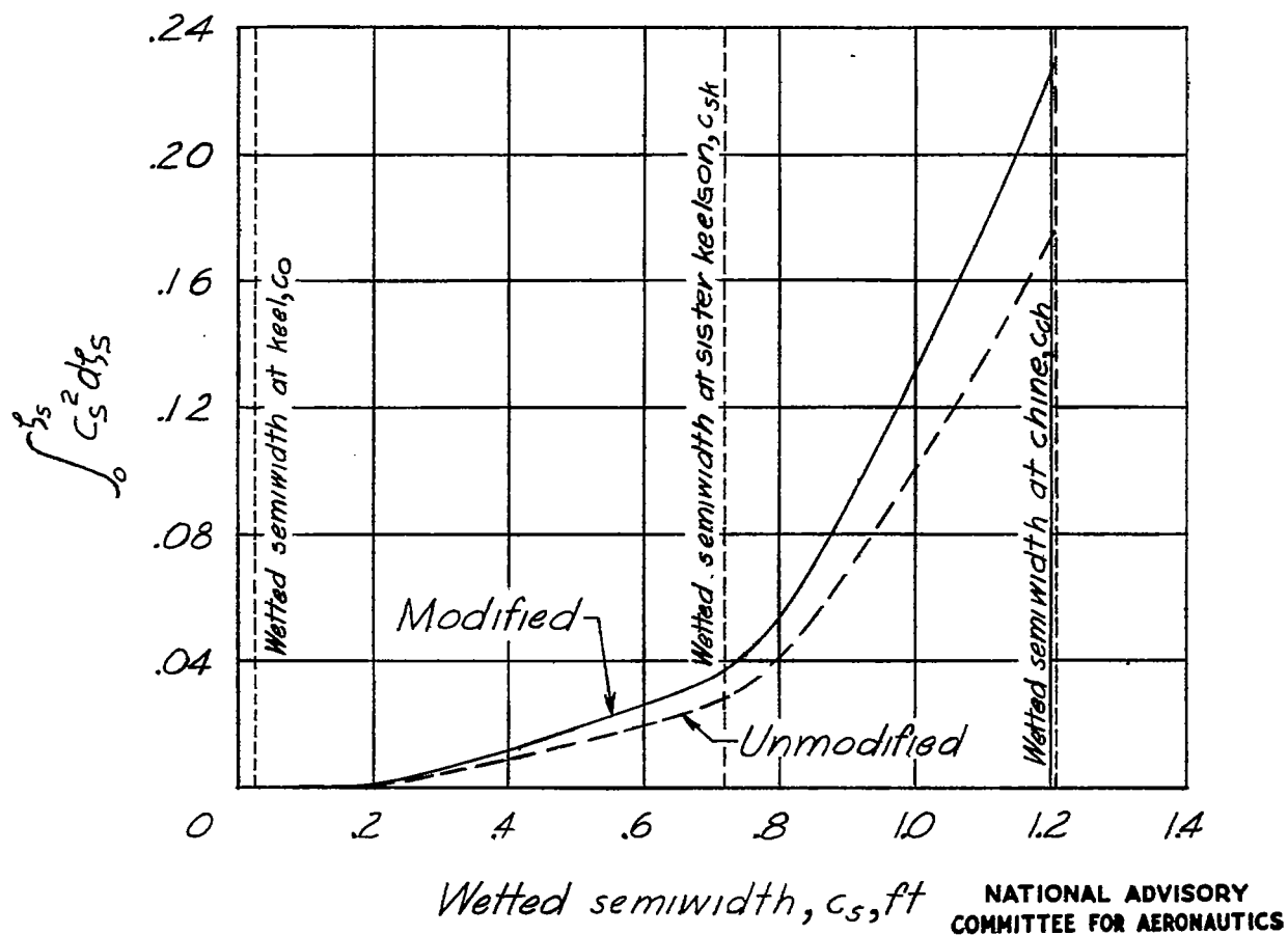
Figure 6. - Calculated variation of \int_0^{s_s} c_s^2 ds_s with wetted semiwidth for scalloped cross section.
