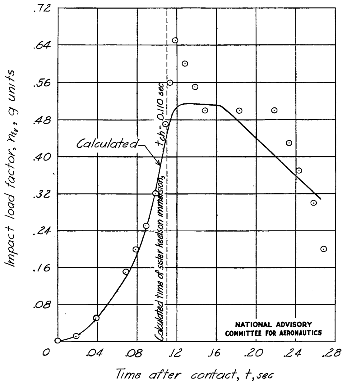
Figure 8.- Calculated and experimental time history of hydrodynamic impact load on scalloped-bottom float. Smooth water; W = 1350 pounds; V_{V_0} = 2.77 feet per second; V_{h_0} = 55.56 feet per second; \tau = 3^\circ .
