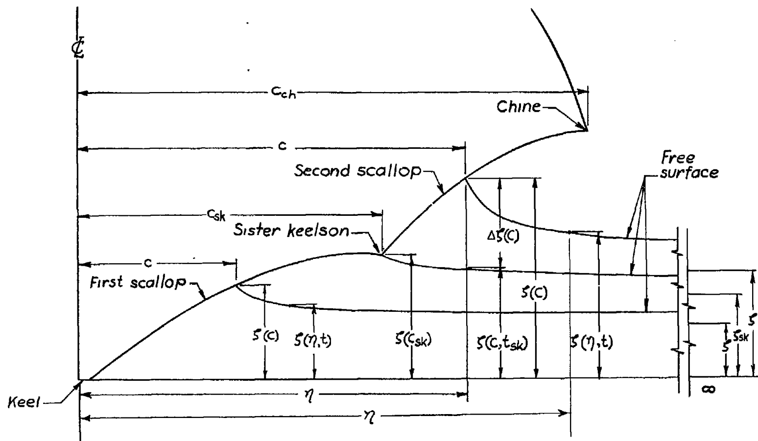
Figure 3.- Symbols and definitions for immersion of scalloped cross section.
