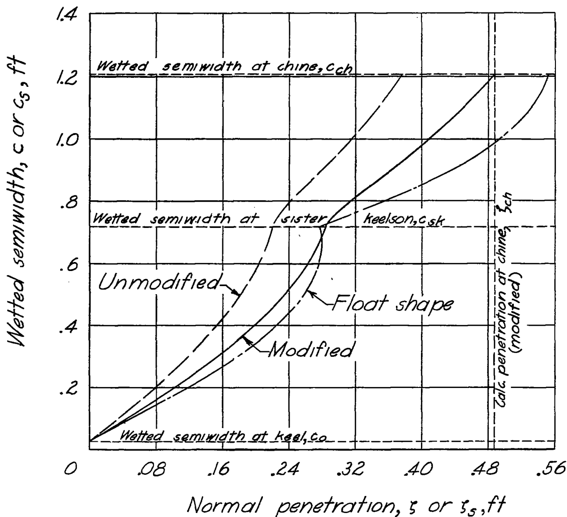
Figure 4. - Calculated section characteristics (variation of wetted semiwidth with penetration) for scalloped cross section.
