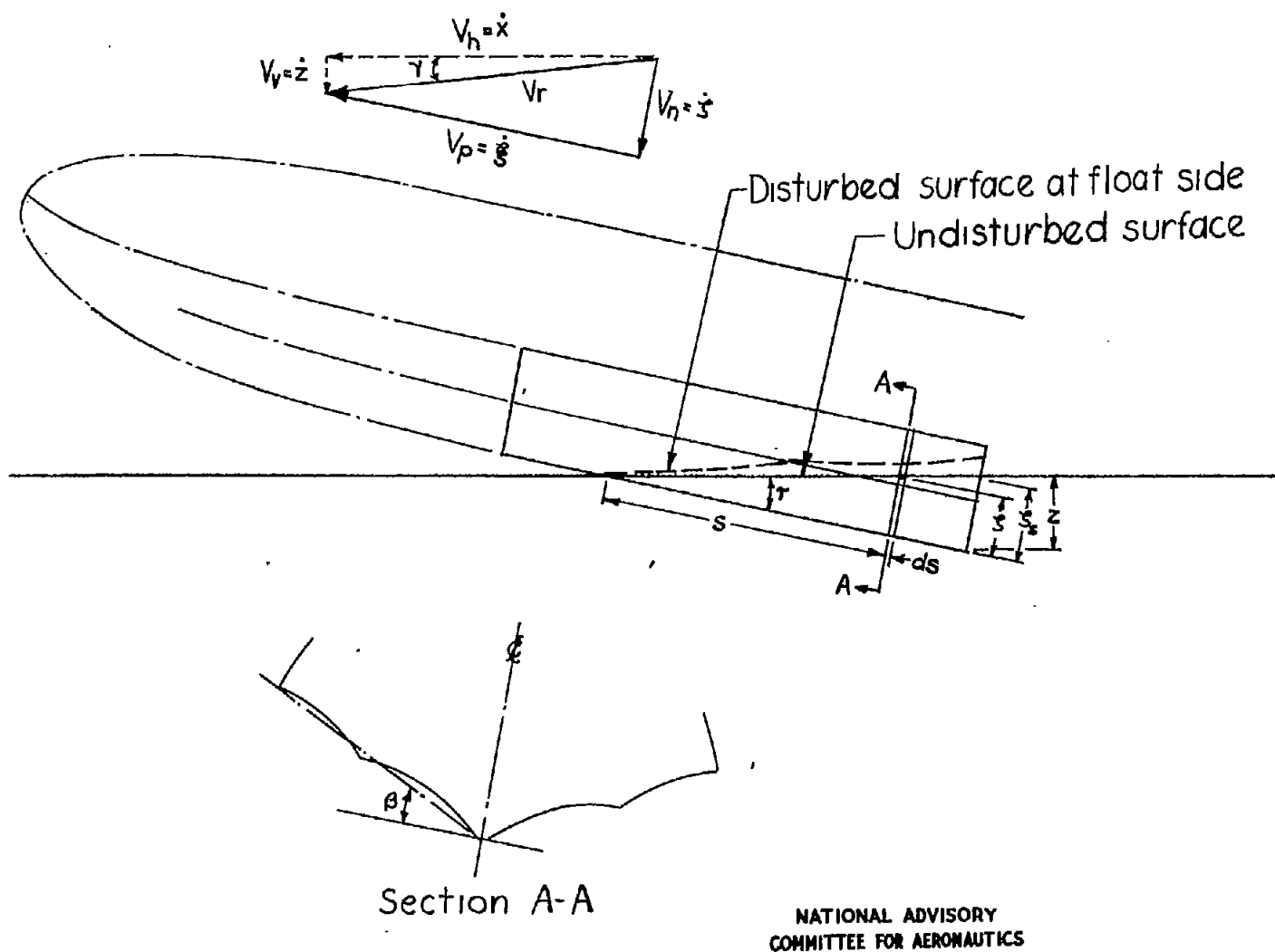
Figure 2.- Immersion of scalloped-bottom float.
