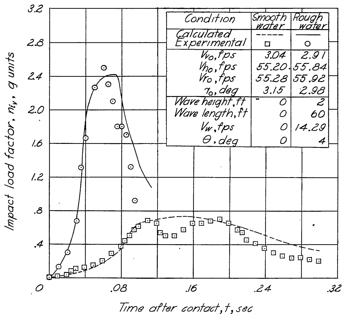
Figure 14.-Comparison of calculated and experimental time histories of hydrodynamic load on scalloped-bottom float for impacts in smooth and rough water with similar flight conditions. W=1350 pounds; \tau = 7^\circ .
