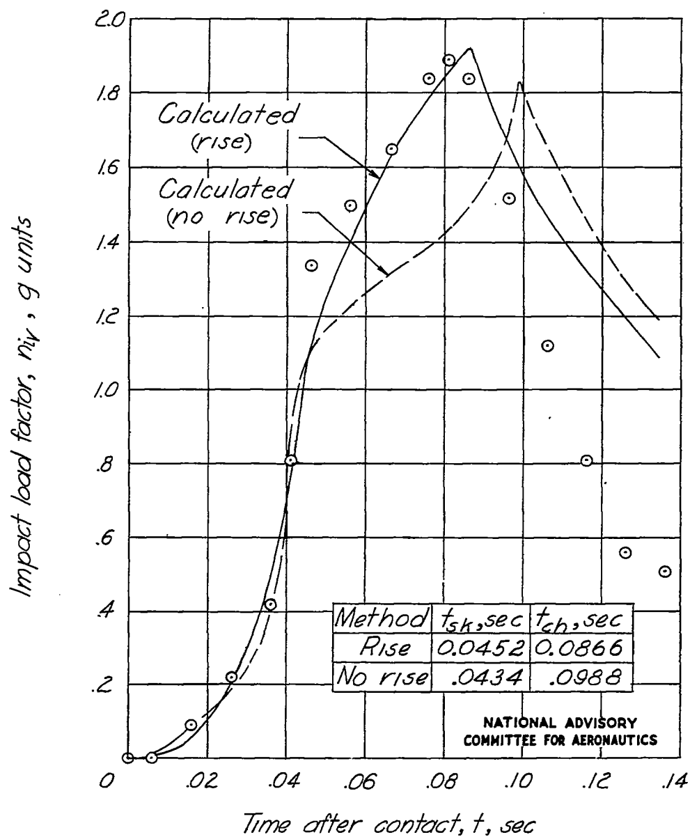
Figure 12.— Calculated and experimental time history of hydrodynamic impact load on scalloped-bottom float. Rough water; W=1350 pounds; V_0=2.77 feet per second; V_{h0}=49.3 feet per second; \tau=10^\circ ; wave height = 2 feet; wave length = 60 feet; V_w=12.27 feet per second; \theta=3.4^\circ .
