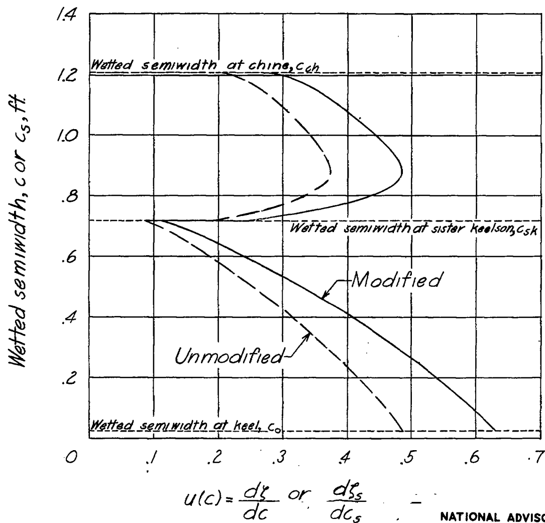
Figure 5. - Calculated variation of u(c) with wetted semiwidth for scalloped cross section.
