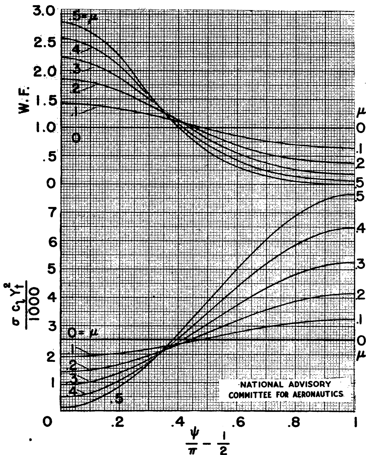
Figure 11.- Chart to be used in determining the effective blade profile-drag coefficient \delta .
