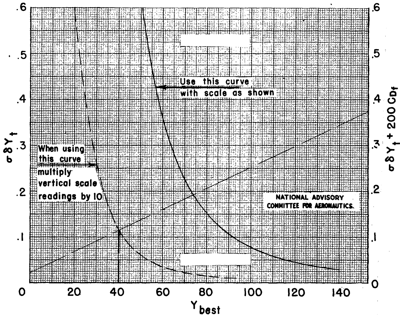
Figure 7.- Chart for finding the best-climbing-speed parameter Y_{best} .
