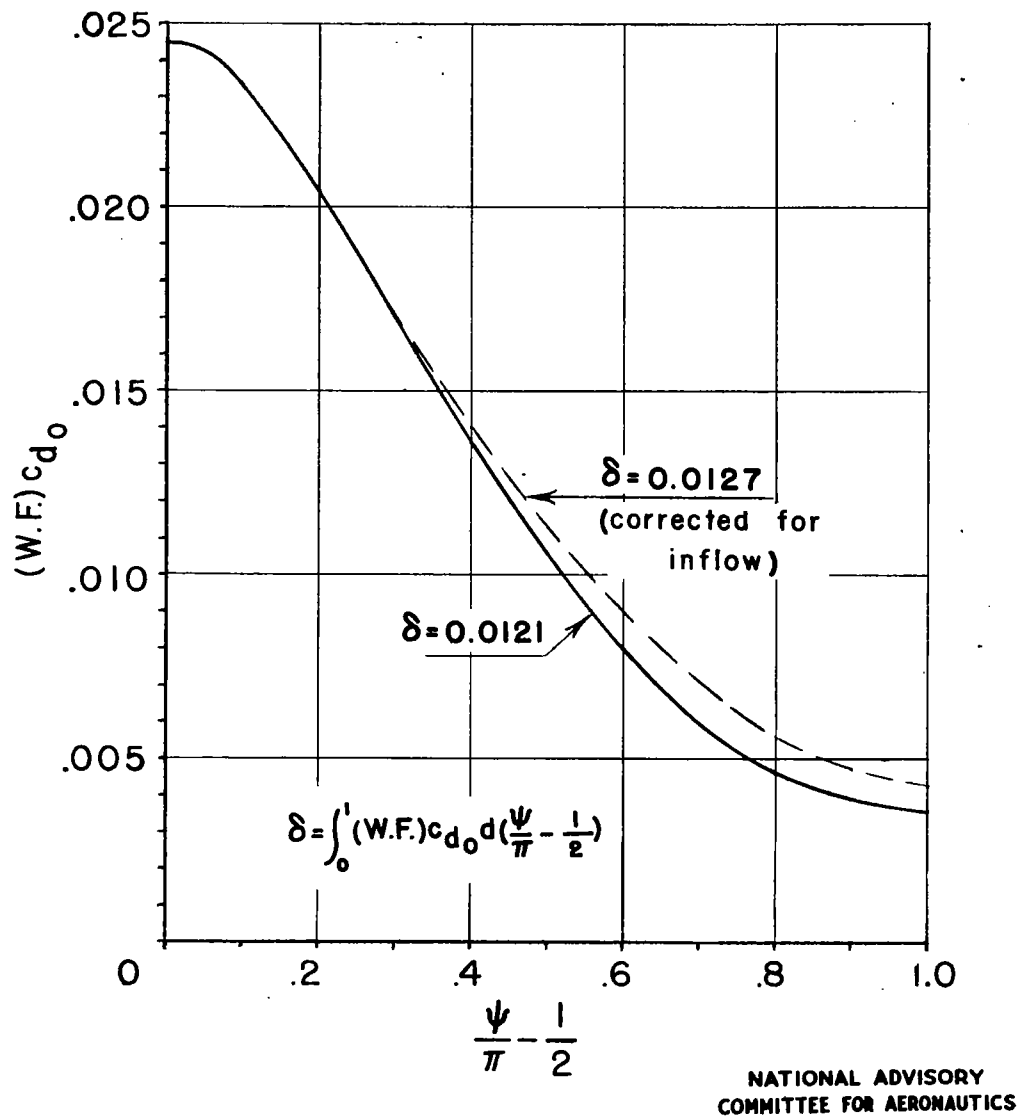
Figure 13.- Sample graph for finding \delta . \sigma Y_t^2 = 5740 ; \mu = 0.3 ; airfoil polar from figure 12.
