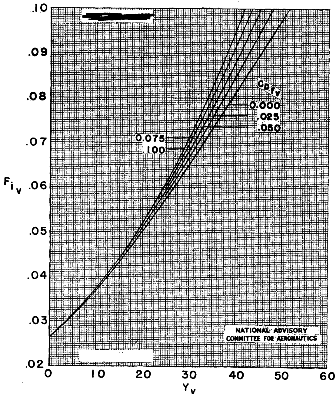
Figure 5.- Minimum induced power-loading parameter in vertical flight F_{i_v} . (For untwisted rectangular blades F_{i_v} is increased 6 percent.)
