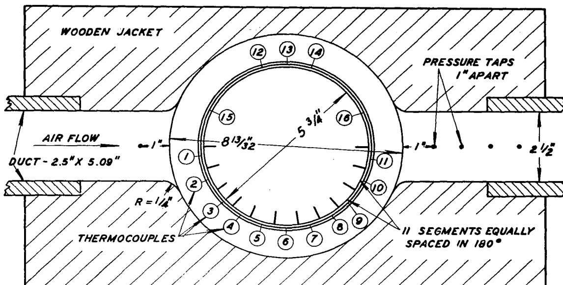
TOP VIEW OF TEST SECTION SHOWING LOCATION OF PRESSURE TAPS AND THERMOCOUPLES ALL COUPLES 2" FROM BOTTOM EXCEPT (12) - \frac{1}{2}" , (14) - 1"
