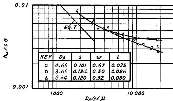
STANTON NUMBER VS REYNOLDS NUMBER SHOWING THE EFFECT OF CYLINDER DIAMETER, REFERENCE 29
