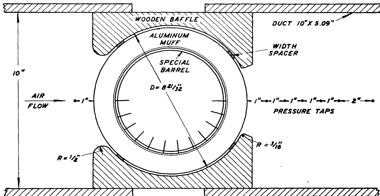
TOP VIEW OF MODEL PRATT AND WHITNEY R2800 ENGINE BAFFLES AS TESTED
