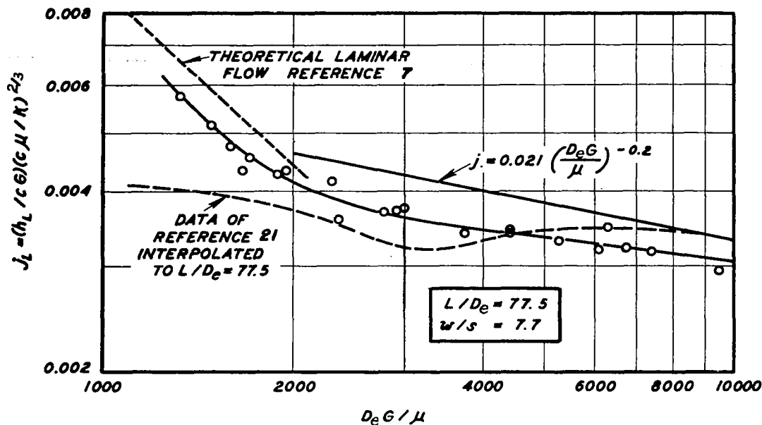
FIGURE 7 HEAT TRANSFER COEFFICIENTS FOR RECTANGULAR DUCTS j_L VS D_e G / \mu , DATA OF REFERENCE 22
