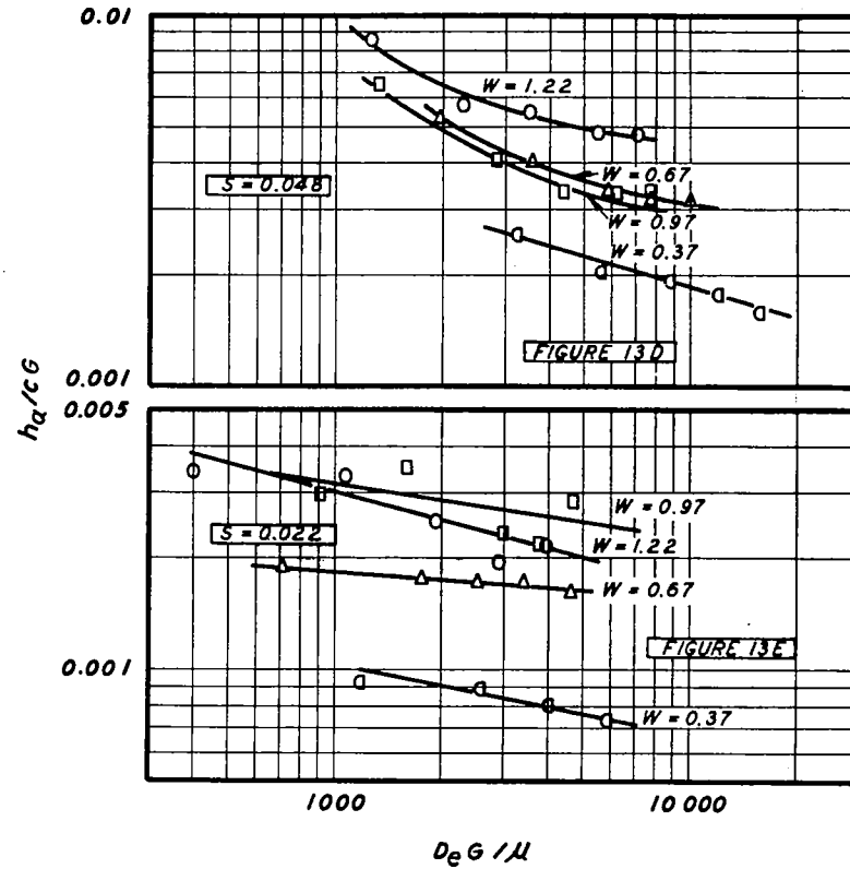
FIGURE 13 STANTON NUMBER VS REYNOLDS NUMBER FOR FINNED CYLINDERS SHOWING THE EFFECT OF FIN WIDTH REFERENCE 29
