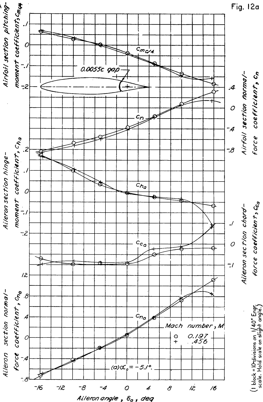
Figure 12.—Section characteristics of the NACA 66,2-216 airfoil with a 0.20c aileron having a blunt-nose balance of 0.35c a and 0.02c balance-nose radii.
