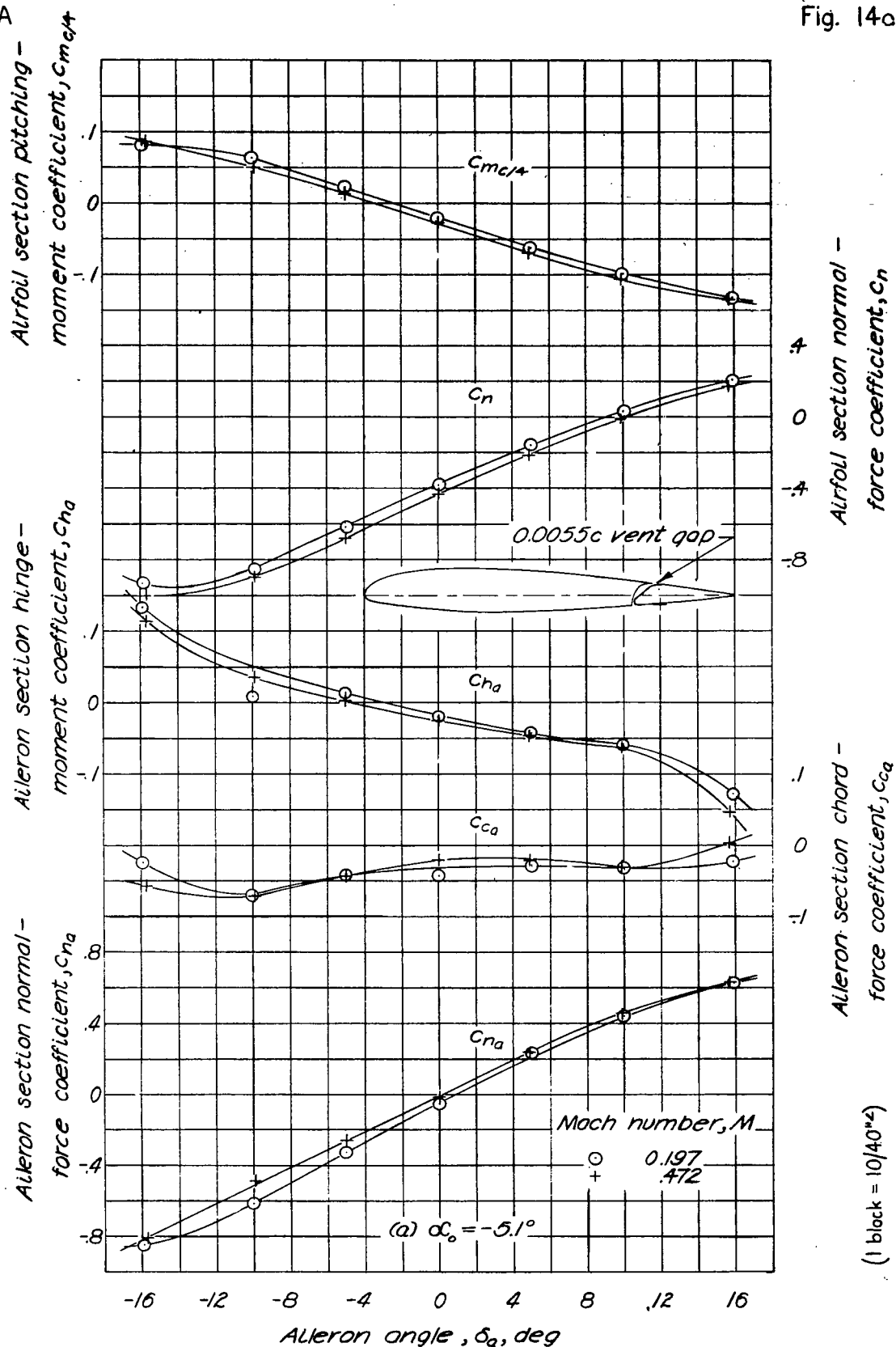
Figure 14. — Section characteristics of the NACA 23012 airfoil with a 0.20c aileron having a Frise type balance of 0.35c and a 0.008c nose radius.
