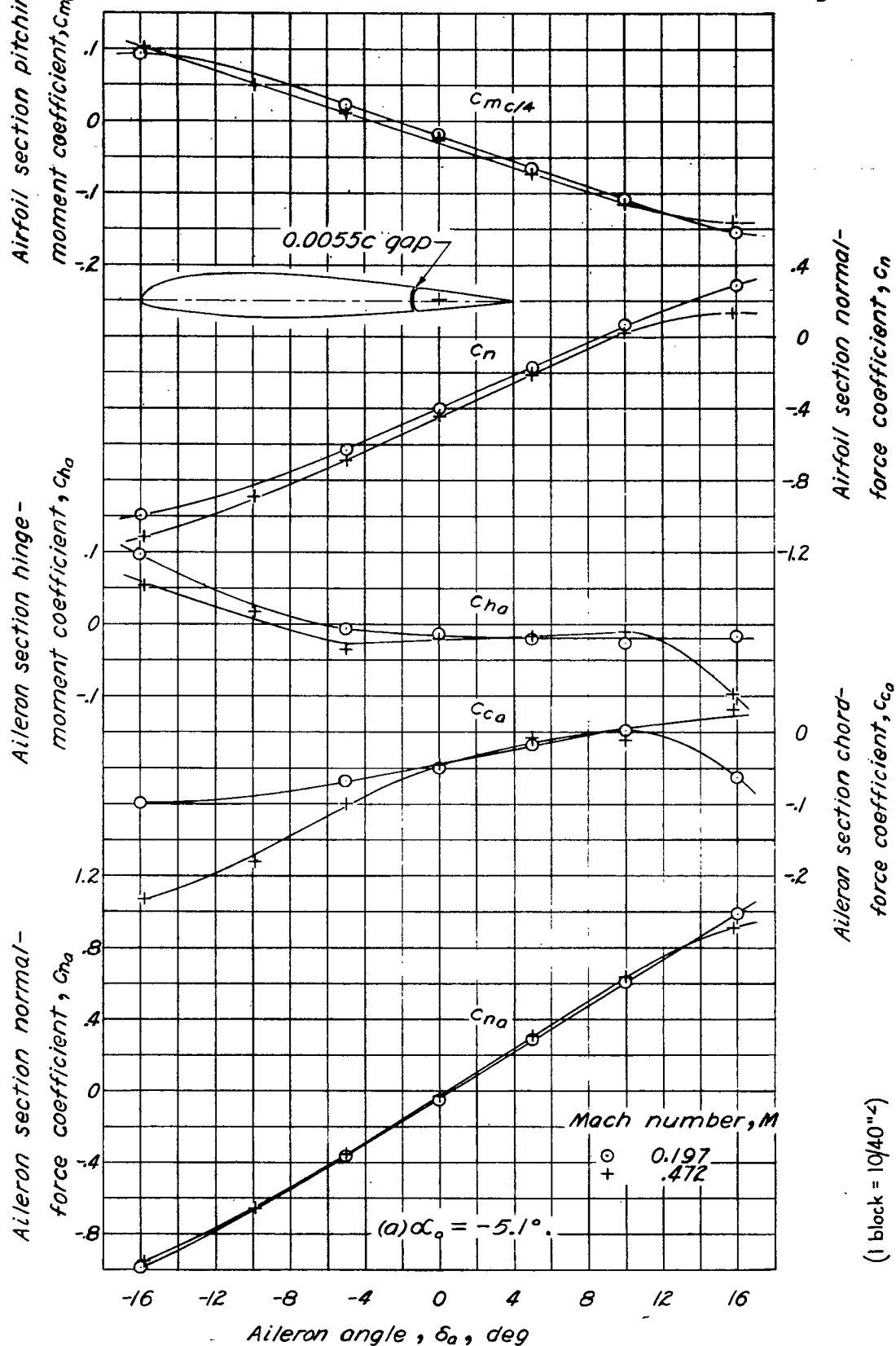
Figure 15.—Section characteristics of the NACA 23012 airfoil with a 0.20c aileron having a blunt nose balance of 0.35c o and 0.02c balance-nose radii.
