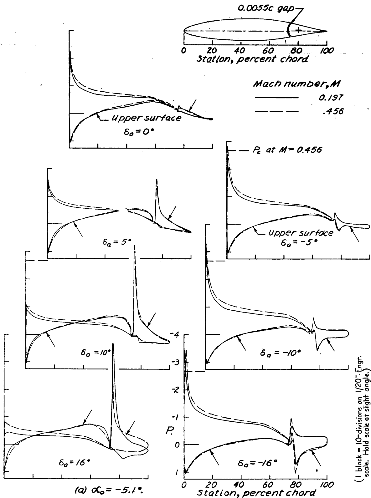
Figure 4. — Pressure distribution of the NACA 66, 2-216 airfoil with a 0.20c gileron having a blunt-nose balance of 0.35c a and 0.02c balance-nose radii.
