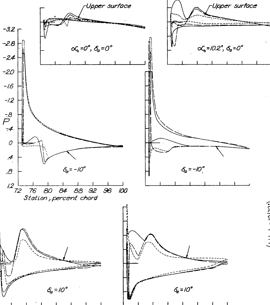
(b) Effect of vent gap and lower-surface radius. Balance-nose radius = 0.008 c. Figure 11. — Concluded.
