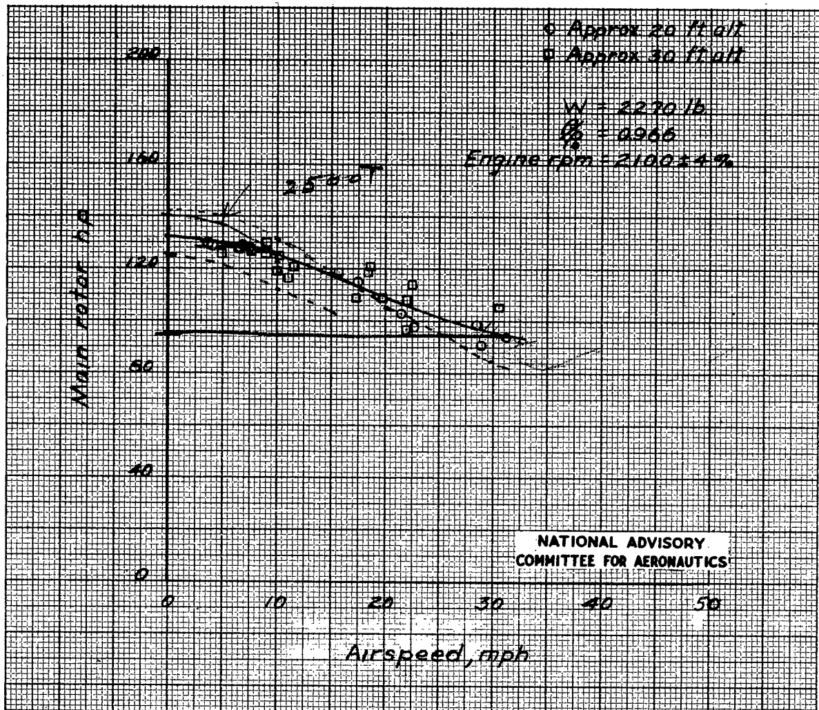
Figure 3.- Preliminary data indicating the effect of airspeed on the main rotor shaft power required by the HNS-1 helicopter in the near hovering condition.
