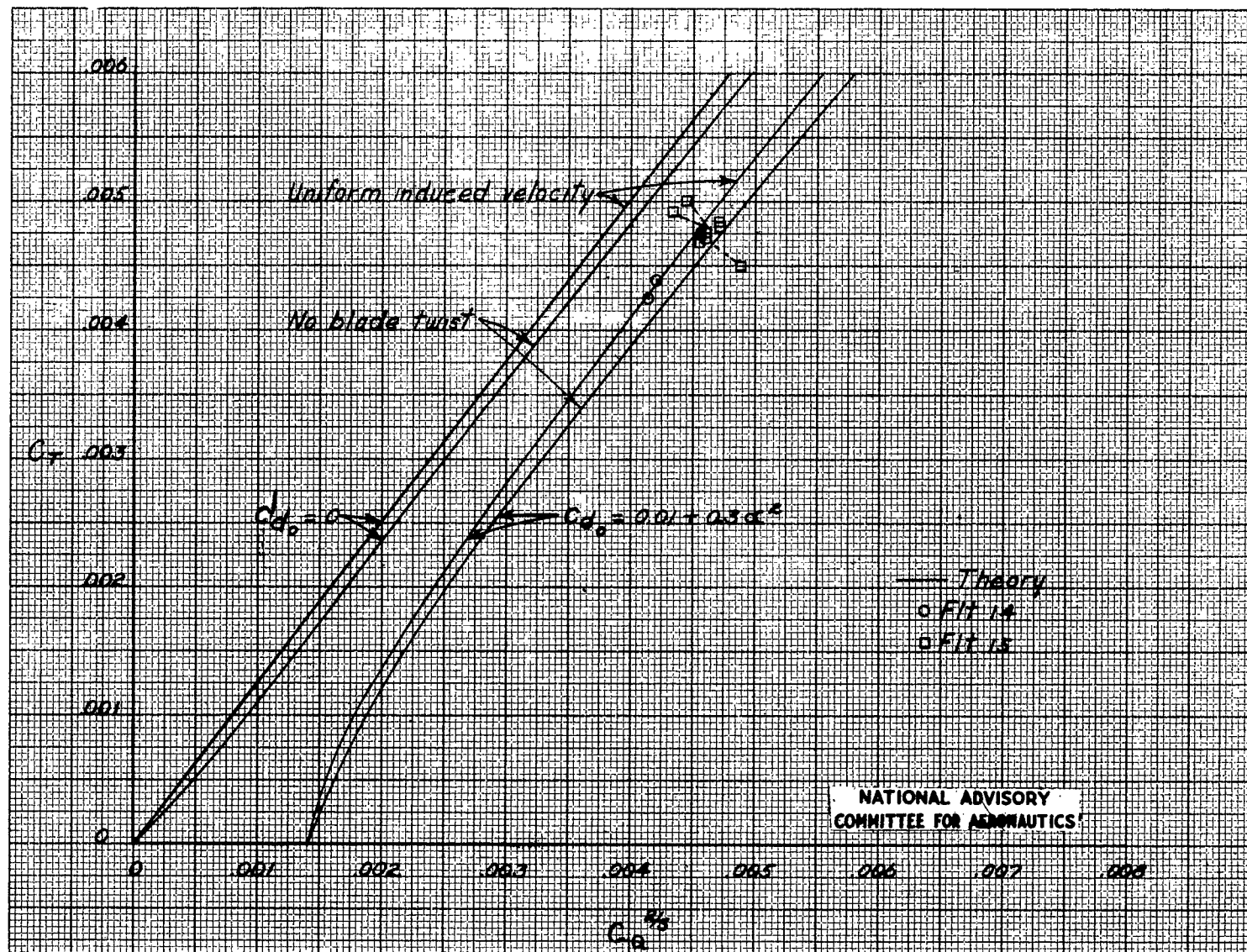
Figure 5.- Comparison of hovering performance of alternate main-rotor blades with theory. Theory from NACA 626 (reference 1): \sigma = 0.042 , constant chord; HNS-1 helicopter.
