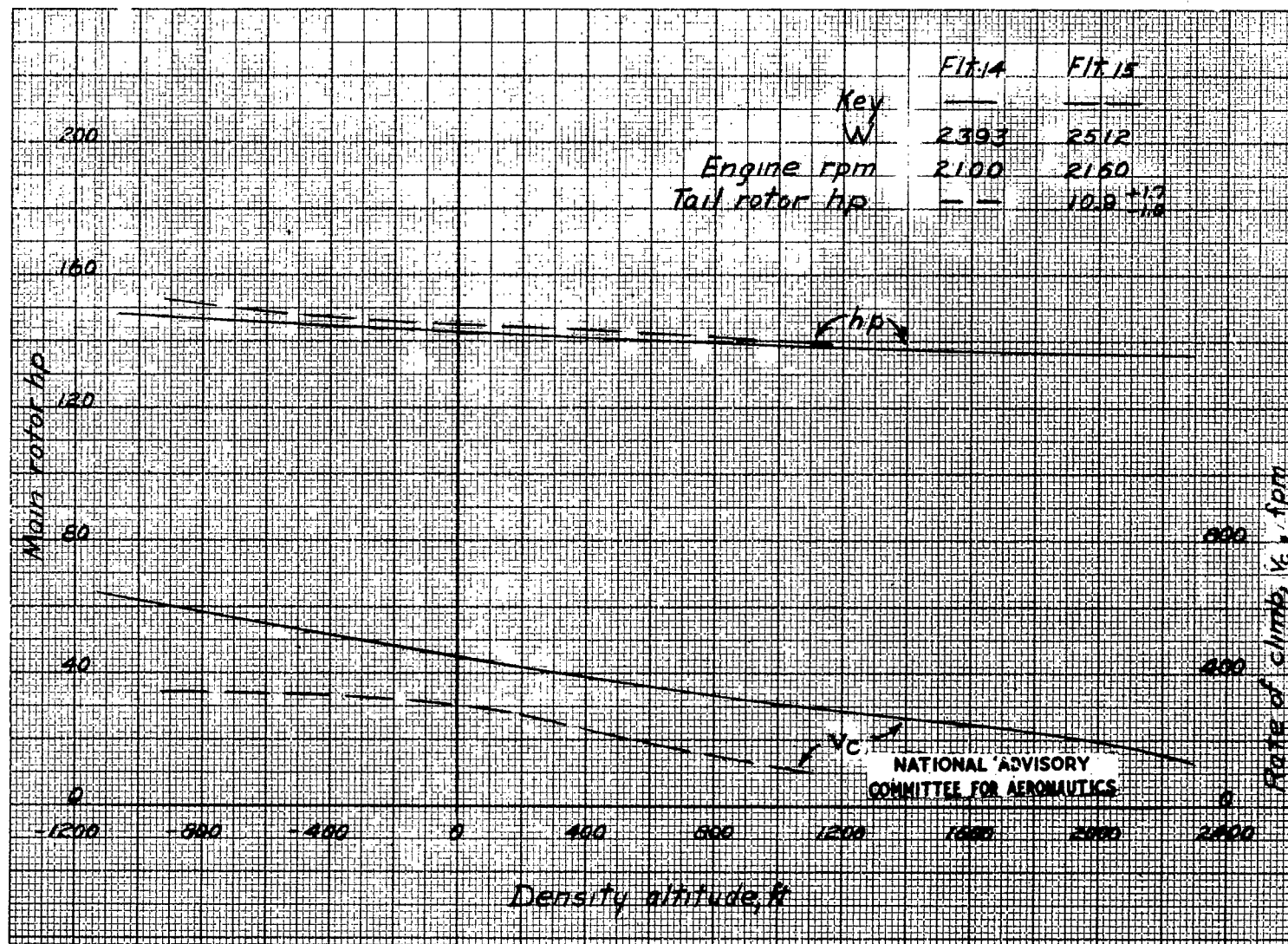
Figure 7.- Continuous climb records obtained with alternate main-rotor blades; HNS-1 helicopter.
