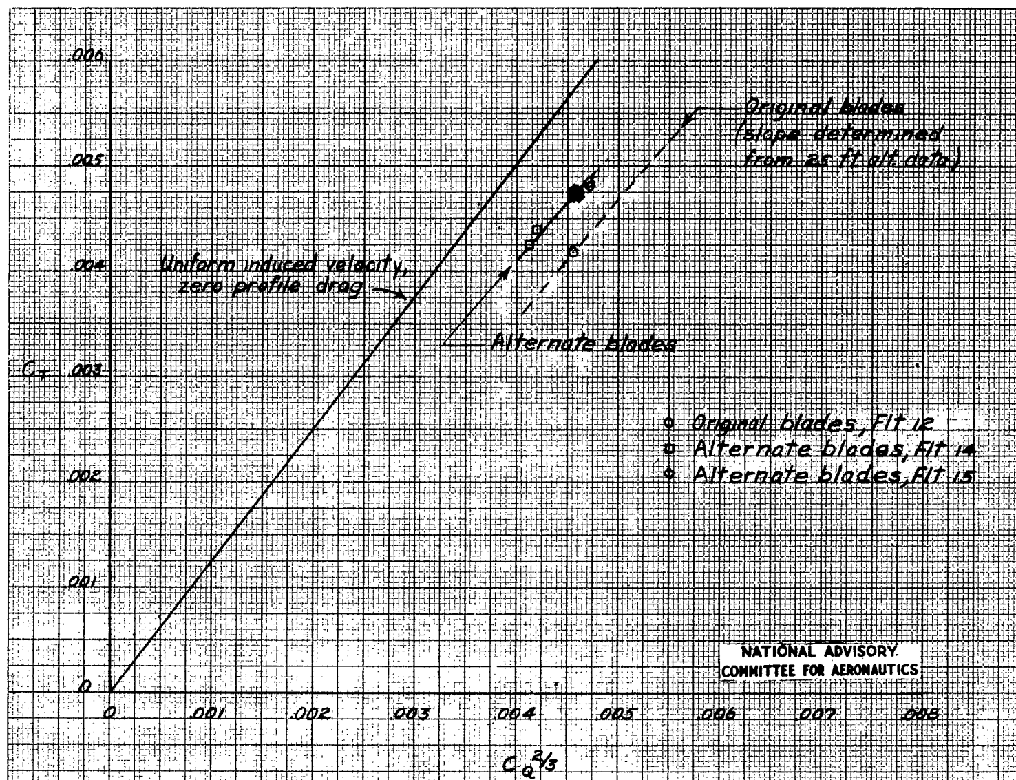
Figure 6.- Comparison of hovering performance of original main-rotor blades and alternate main-rotor blades; HNS-1 helicopter.
