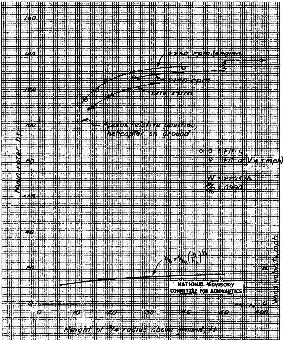
(a) Main rotor shaft power vs. height
