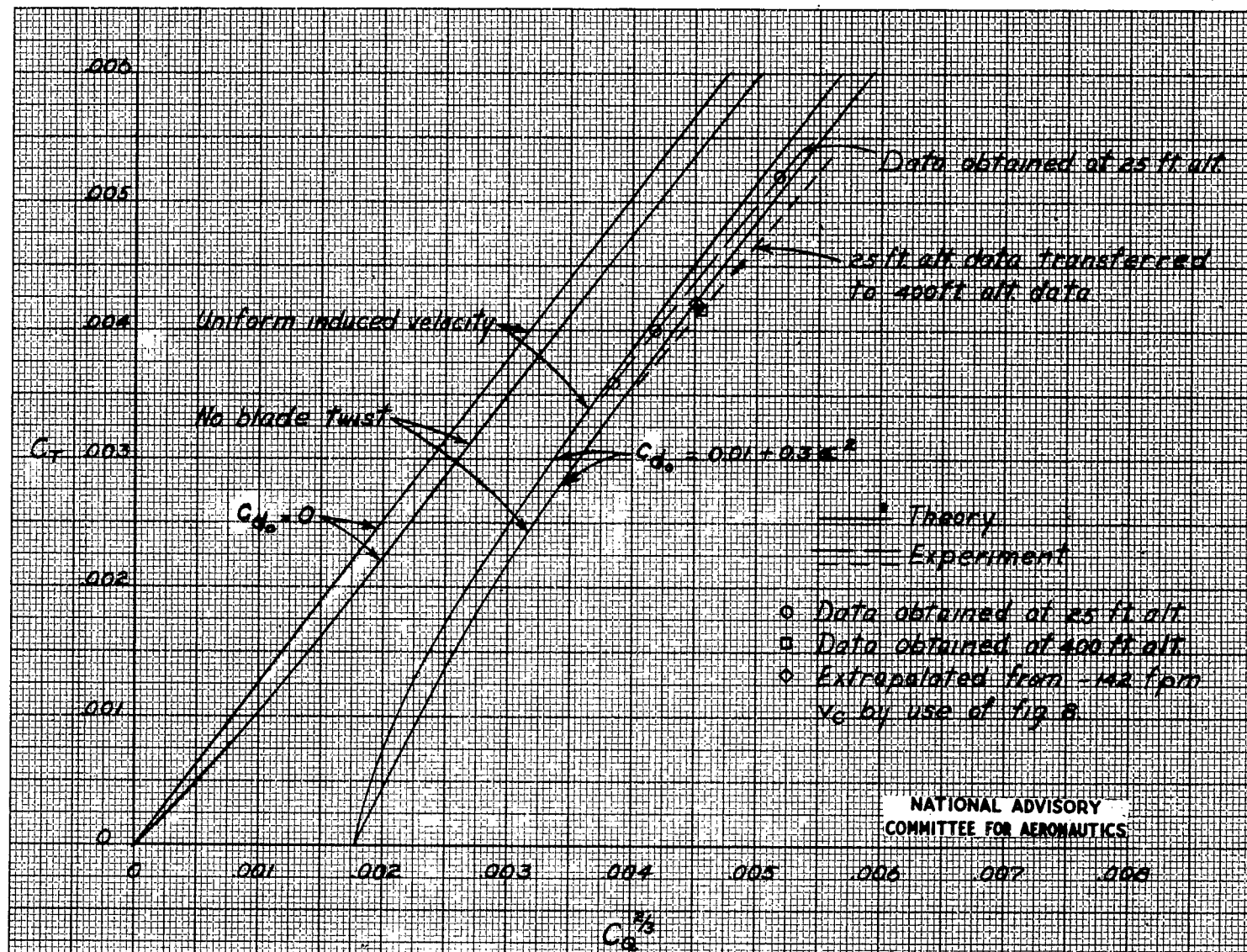
Figure 4.- Comparison of hovering performance of original main rotor blades with theory. Theory from NACA TN 626 (reference 1): \sigma = 0.060 , constant chord; HNS-1 helicopter.
