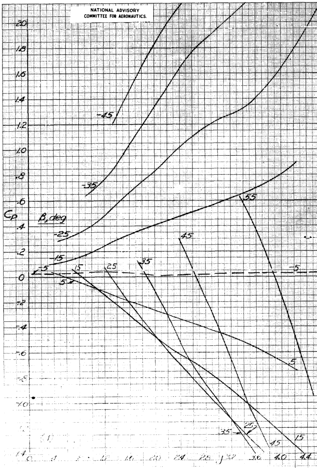
Figure 10. Variation of power coefficient with advance ratio, slight narrow blades. Best rotation.
