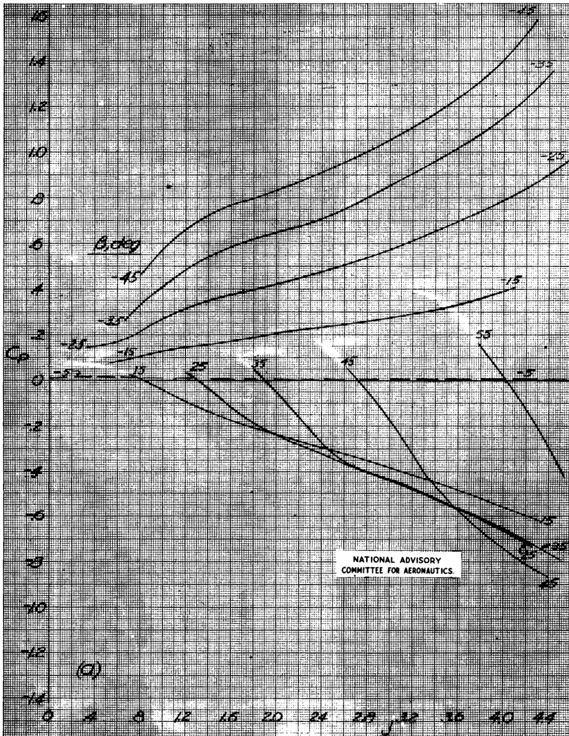
Figure 8.- Variation of power coefficient with advance ratio, four narrow blades, single rotation.
