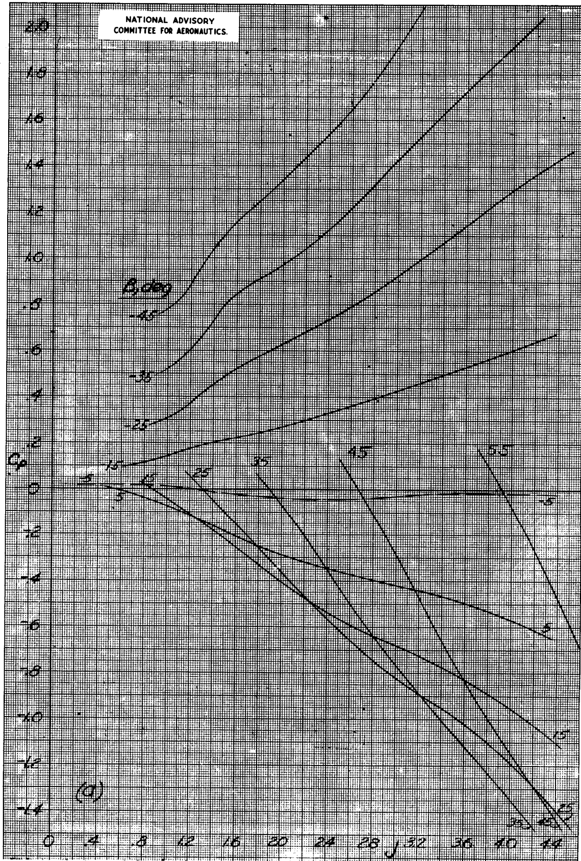
Figure 20.- Variation of power coefficient with advance ratio, four wide blades, dual rotation.
