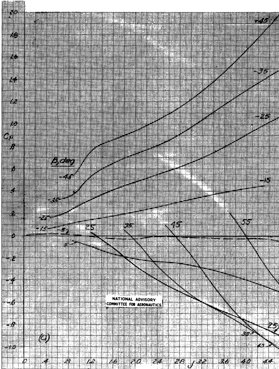
Figure 16.- Variation of power coefficient with advance ratio, three wide blades.
