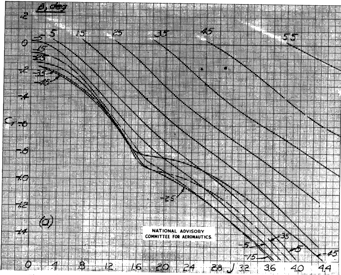
Figure 17.- Variation of thrust coefficient with advance ratio, four wide blades, single rotation.
