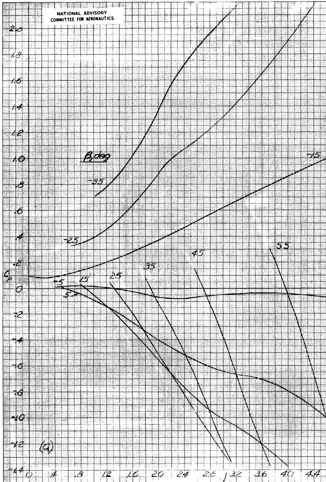
Figure 22.- Variation of power coefficient with advance ratio, six wide blades, dual rotation.
