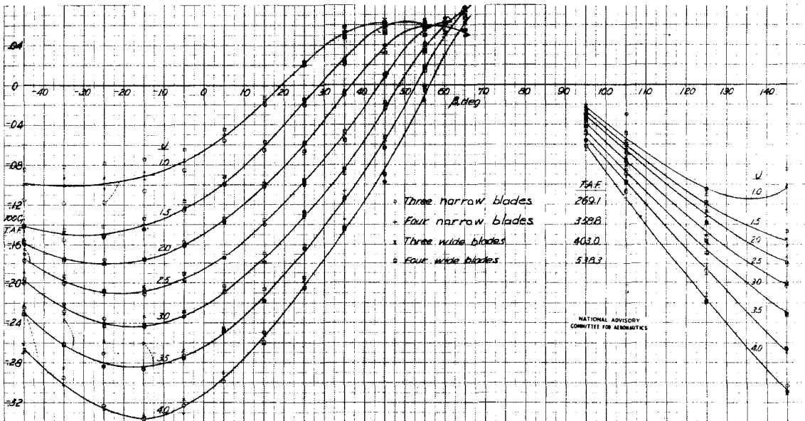
(a) Single rotation, thrust coefficient. Figure 25 - General propeller chart based on common activity factor.
