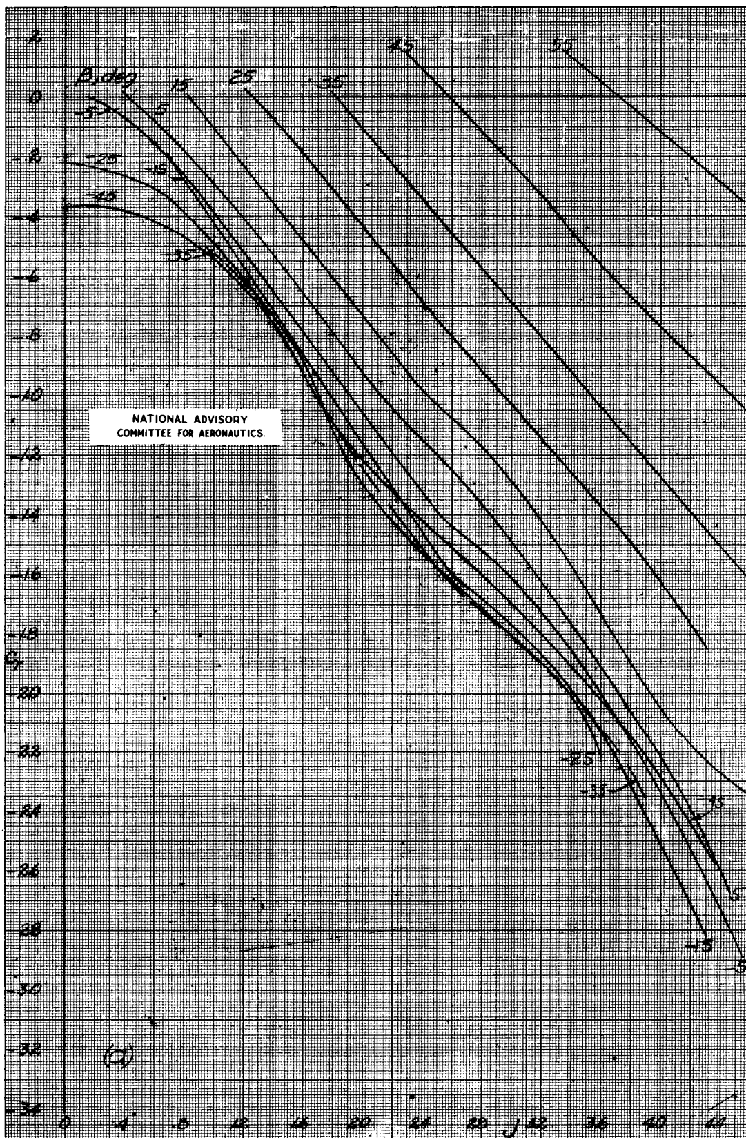
Figure 13.- Variation of thrust coefficient with advance ratio, eight narrow blades, dual rotation.
