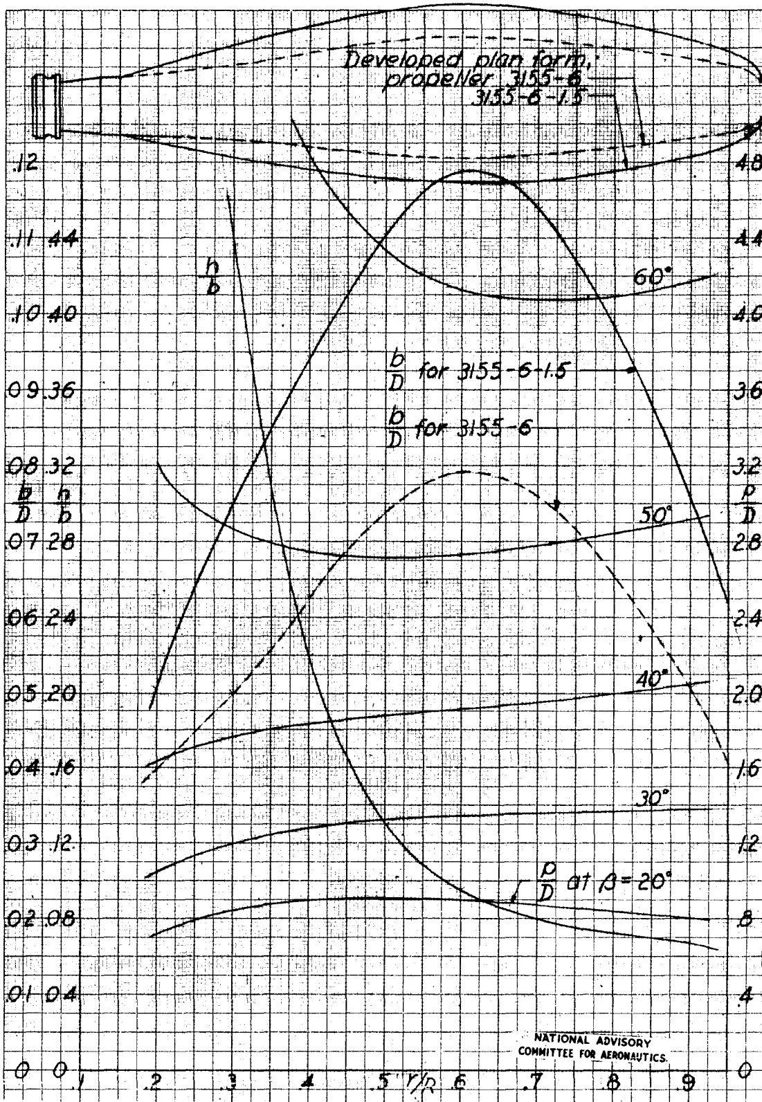
Figure 3.- Plan form and blade-form curves for propellers 3155-6 and 3155-6-1.5. Blade-form curves, except b/D , are identical for the two propellers. D, diameter; R, radius; r, station radius; b, section chord; h, section thickness; p, geometric pitch.
