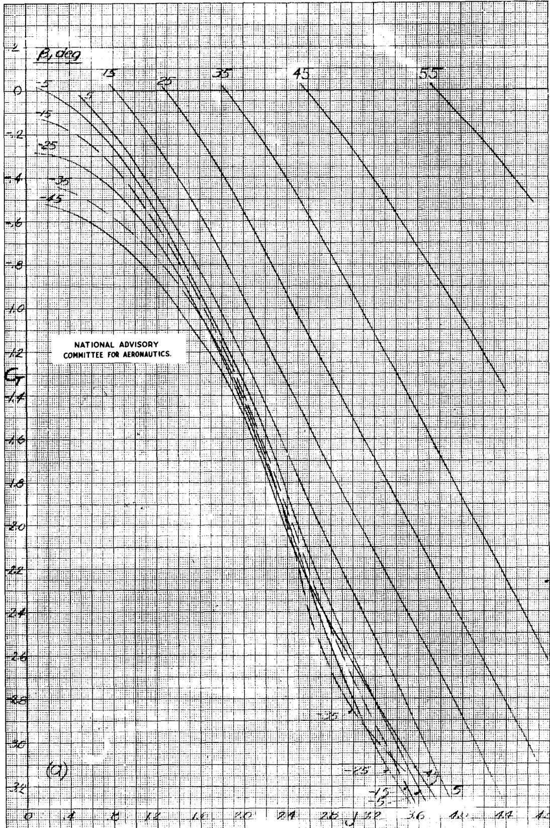
Figure 23.- Variation of thrust coefficient with advance ratio, eight wide blades, dual rotation.
