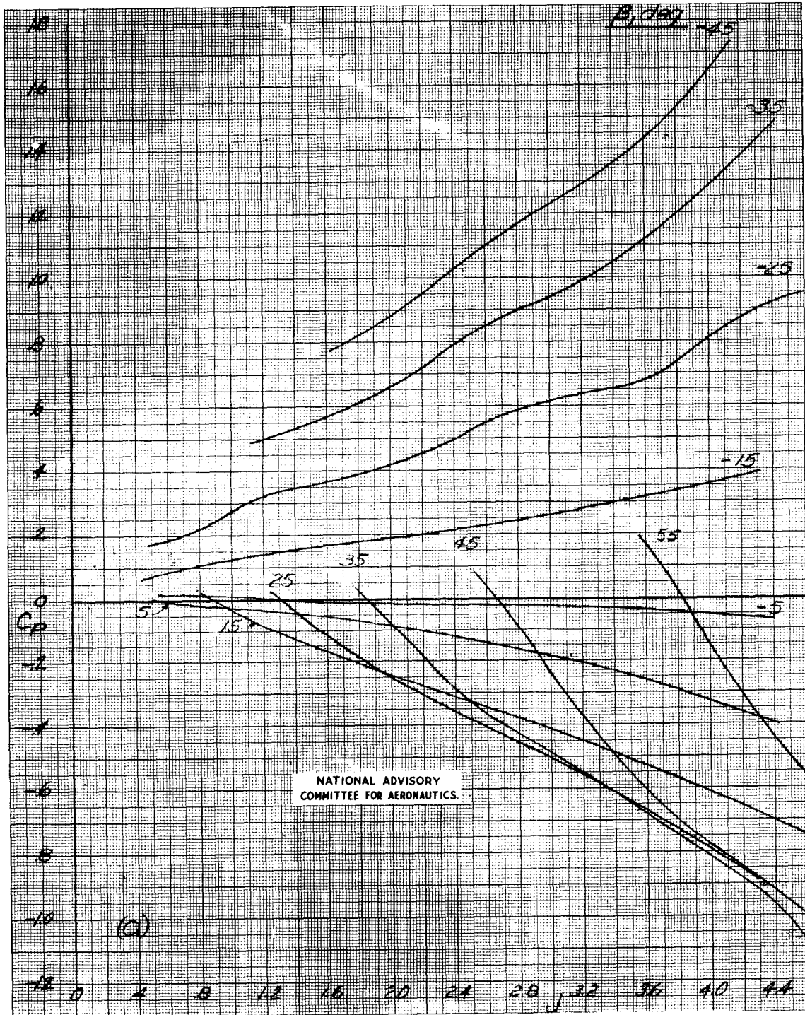
Figure 10.- Variation of power coefficient with advance ratio, four narrow blades, dual rotation.
