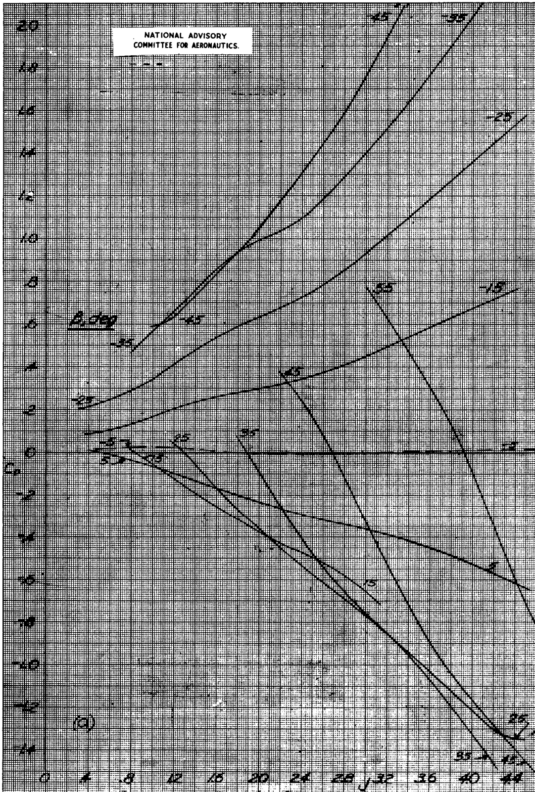
Figure 12.- Variation of power coefficient with advance ratio, six narrow blades, dual rotation.
