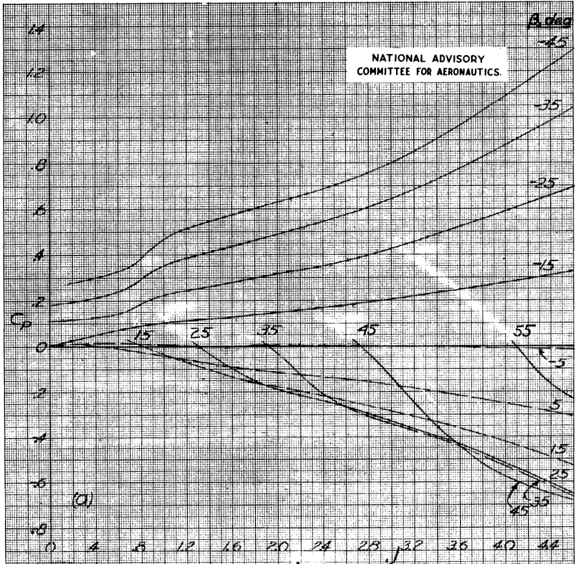
Figure 6.- Variation of power coefficient with advance ratio, three narrow blades.
