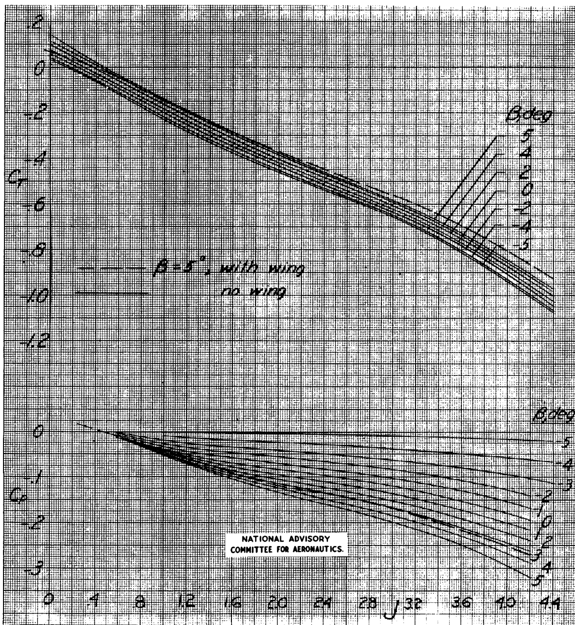
Figure 26.- Variation of thrust and power coefficients with advance ratio for small increments of \beta , three narrow blades.
