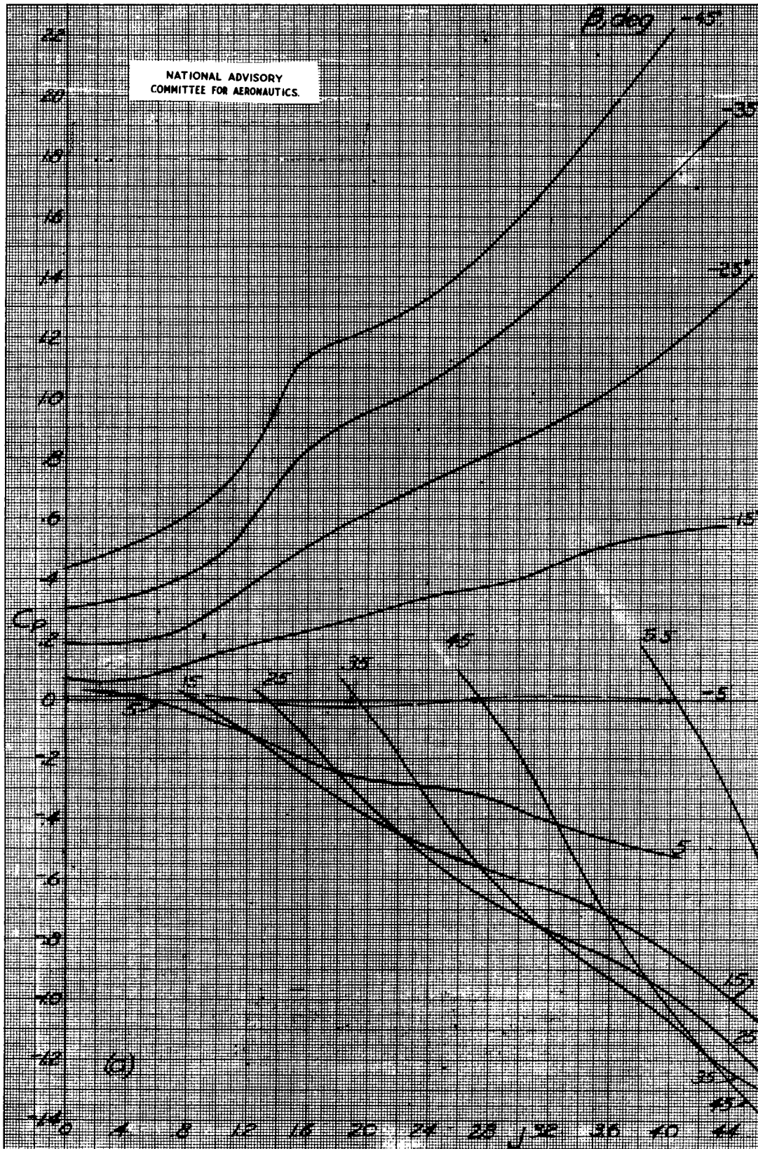
Figure 15.- Variation of power coefficient with advance ratio, four wide blades, single rotation.
