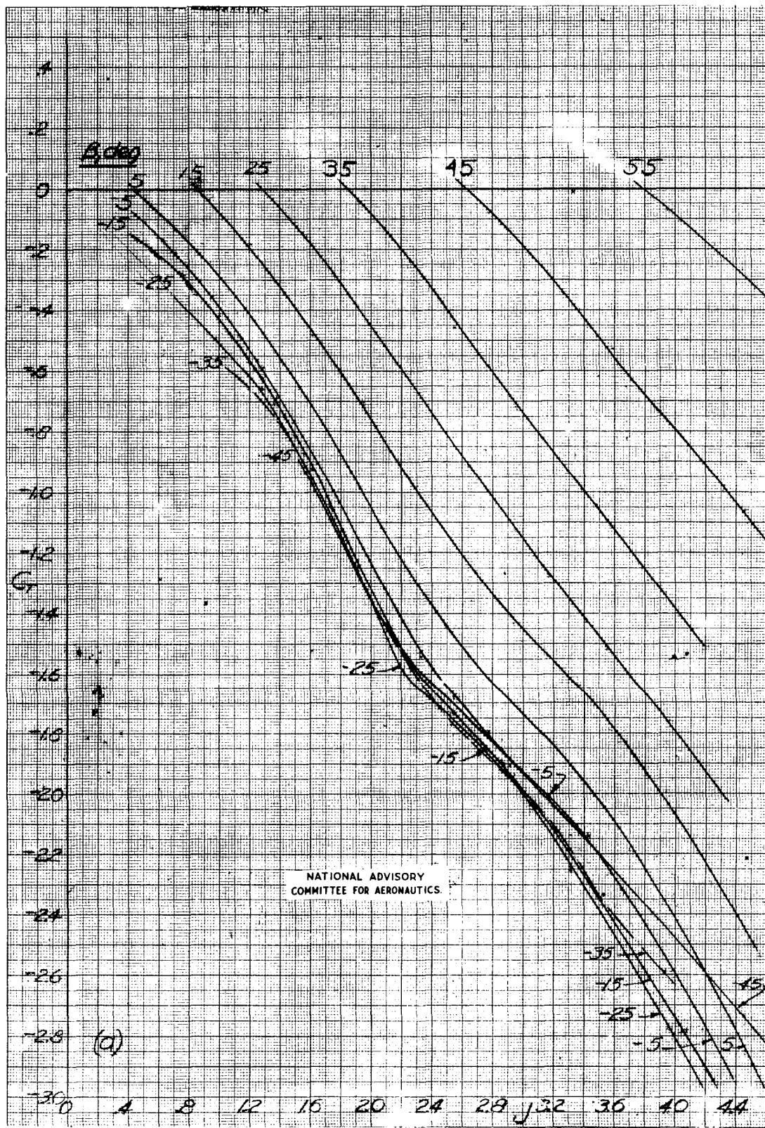
Figure 21.- Variation of thrust coefficient with advance ratio, six wide blades, dual rotation.
