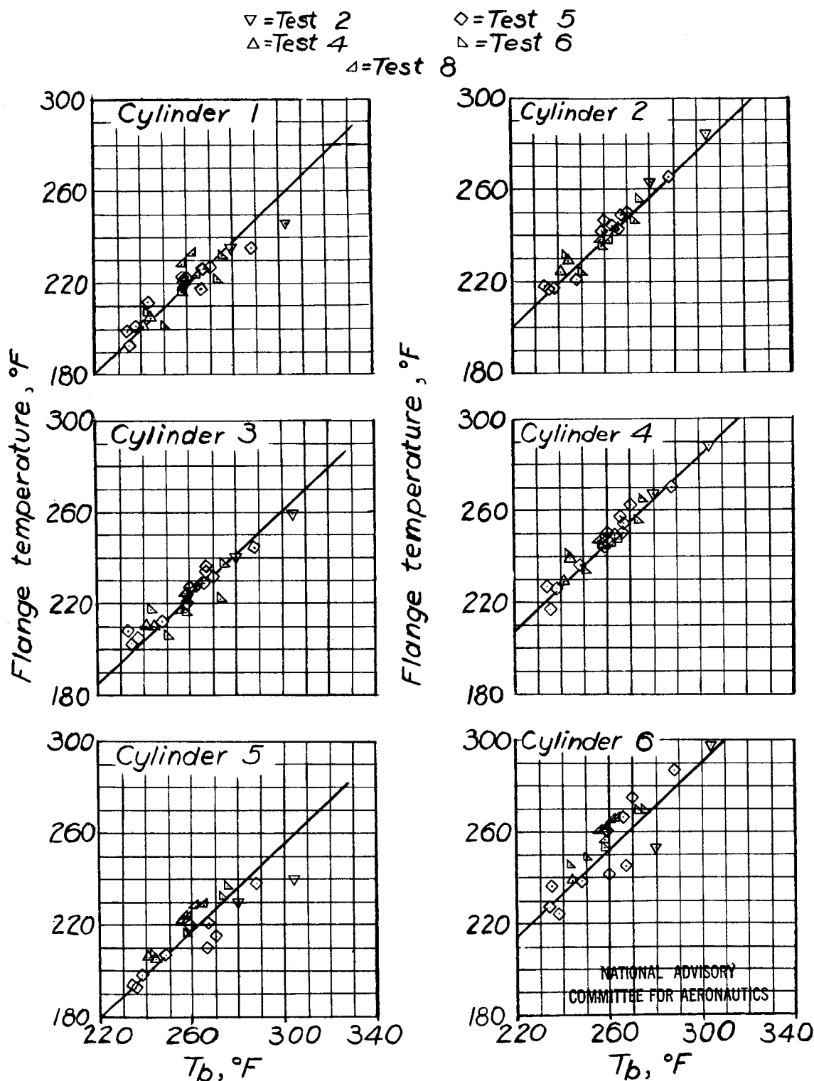
Figure 20. - Variation of cylinder-flange temperatures with average barrel temperatures.
