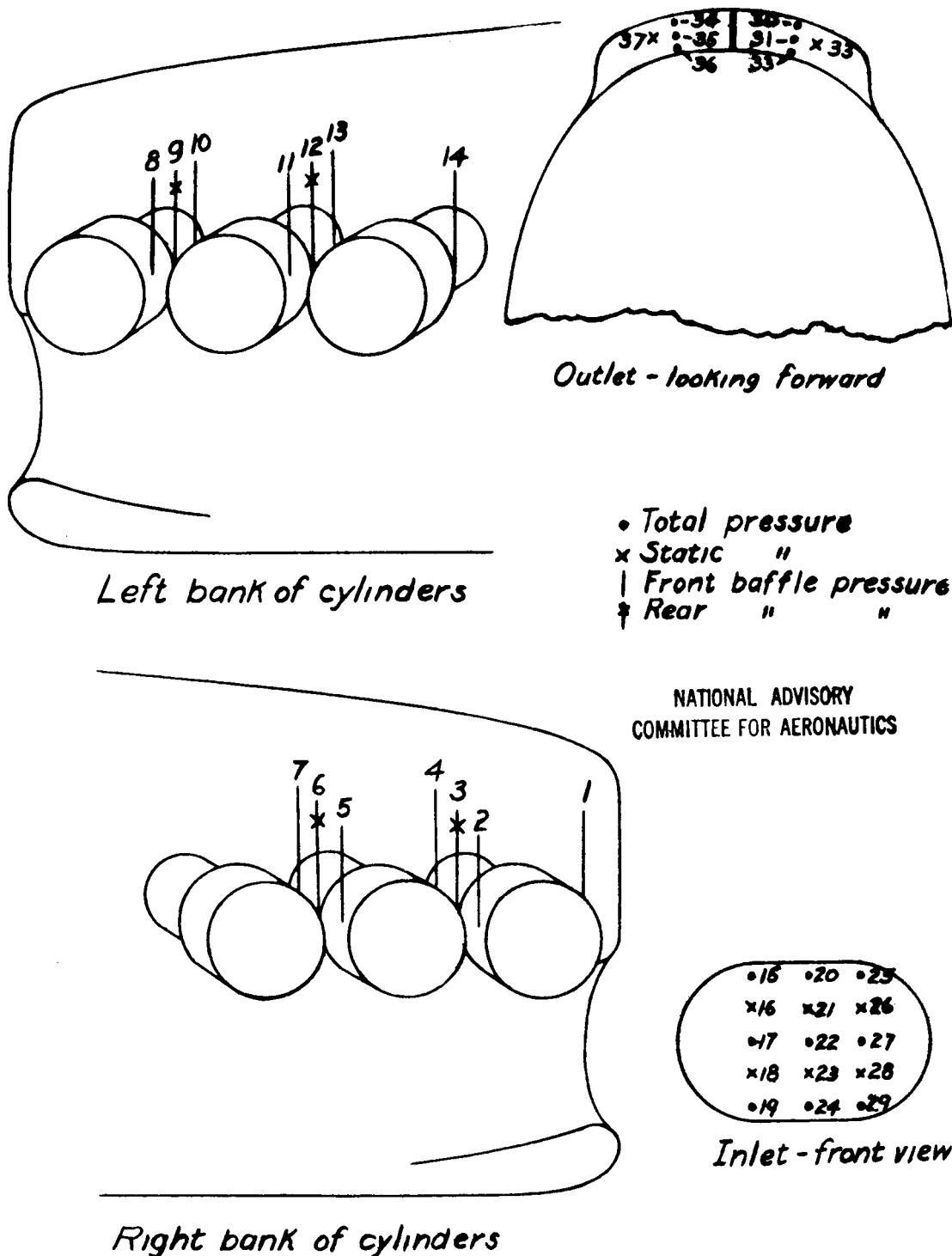
Figure 13.- Sketch showing location of static and total pressure tubes in modified cowling.
