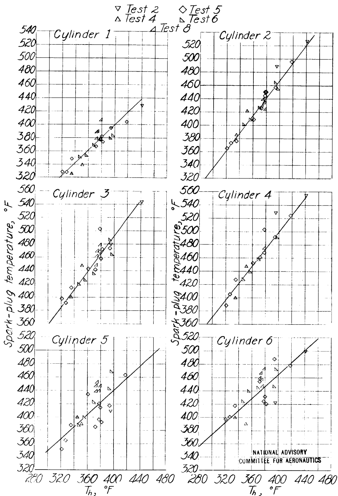
Figure 19.- Variation of rear-spark-plug temperatures with average head temperature.
