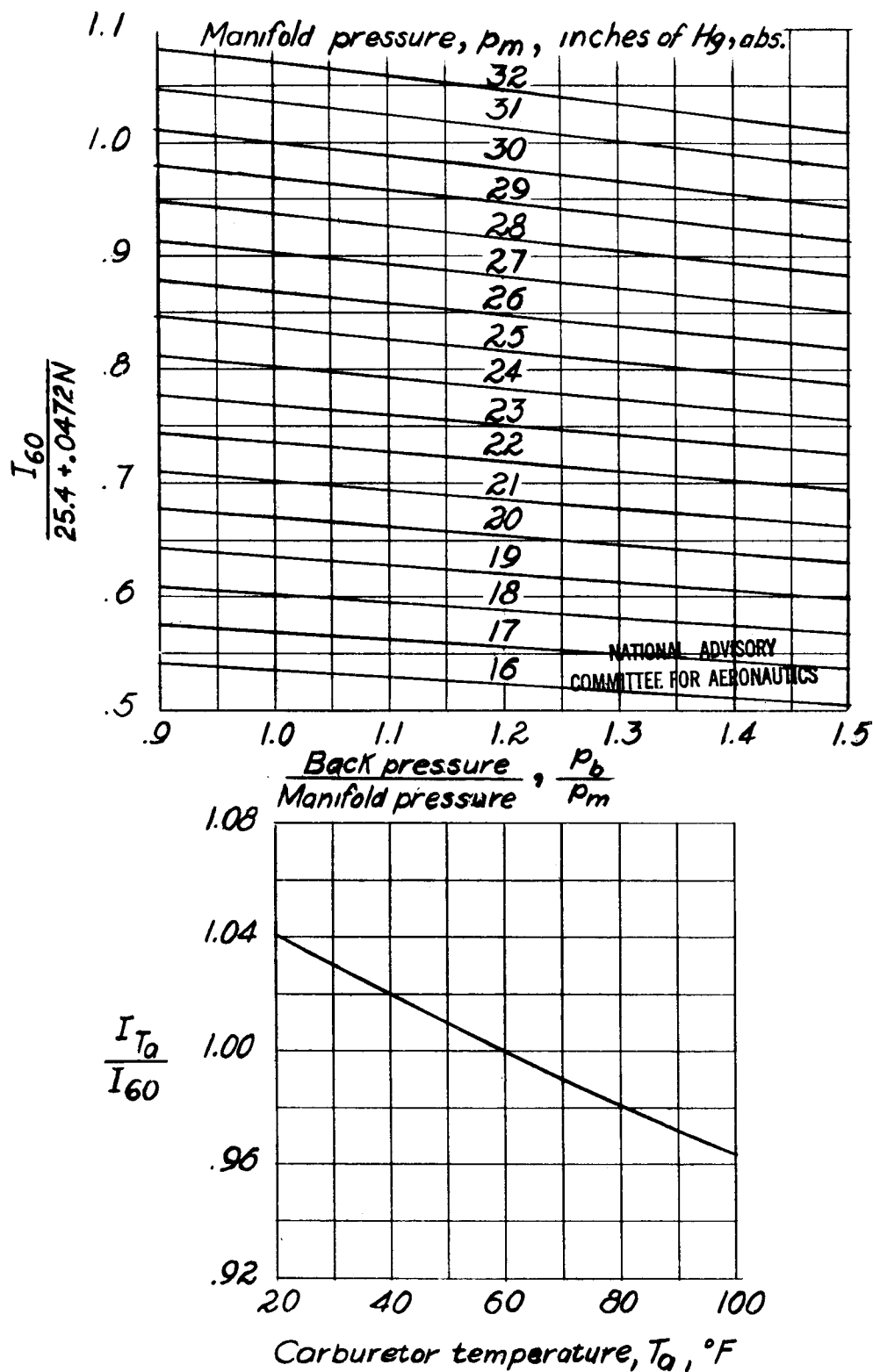
Figure 14.- Estimated indicated horsepower chart for Franklin 6-AC-298 engine.
