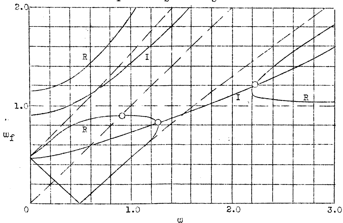
Figure 8.- Plot of real and imaginary equations for case of s = \infty ; \Lambda_1 = .07 ; \Lambda_2 = .22 ; \Lambda_3 = .198 .
