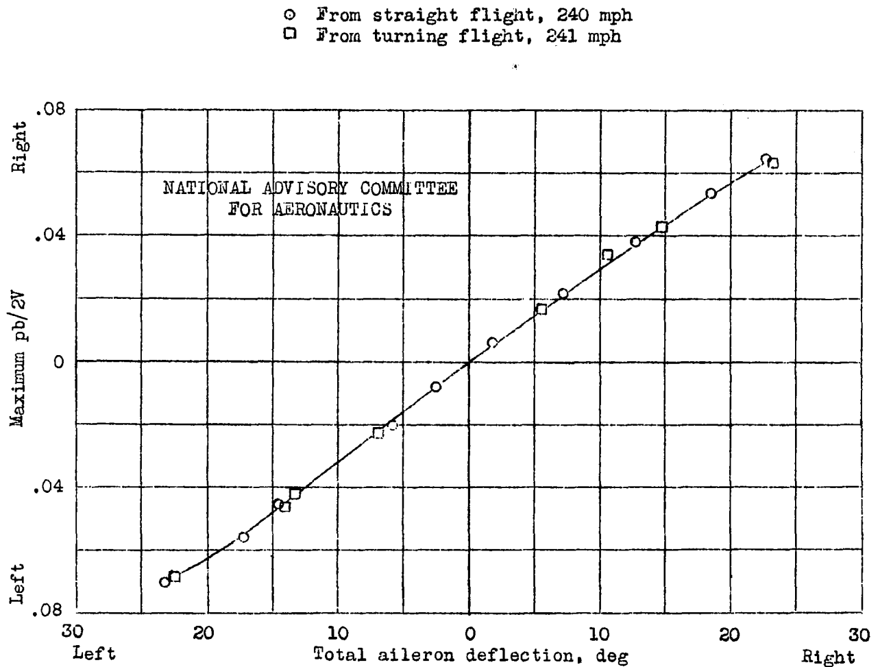
(b) Rolls at moderate airspeed, normal rated power
