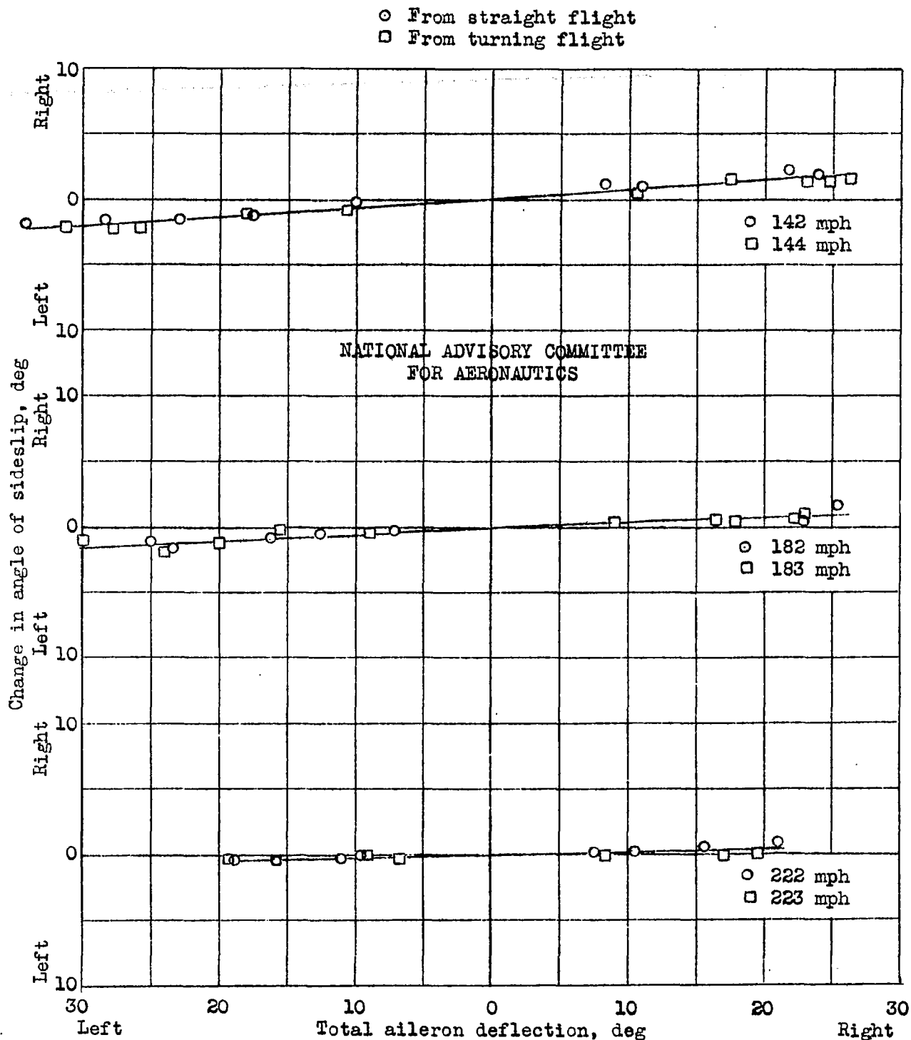
Figure 7.- Comparison between flight determinations of change in sideslip angle corresponding to maximum rolling velocity in rudder-fixed aileron rolls from straight, unbanked flight and from steady, turning flight. Clean condition, normal rated power. Lockheed PV-1 airplane.
