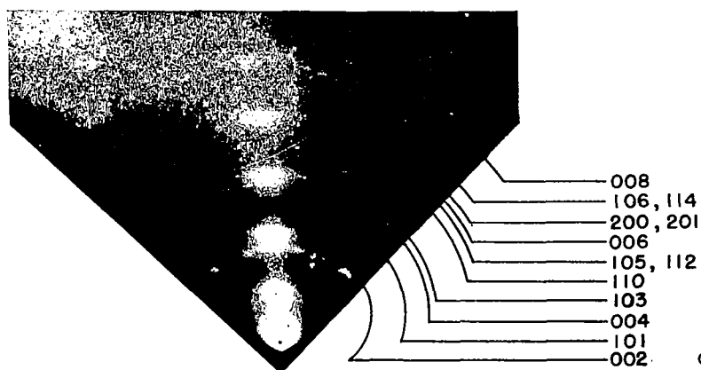
Figure 2.—Electron-diffraction pattern of graphite showing preferred orientation (cleavage planes parallel to the surface). The heavy short arcs are the (002), (004), (006), and (008) planes. Camera constant, 14.0. \times 2 .
