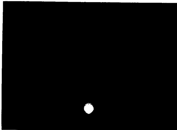
Figure 7.—Representative electron-diffraction pattern of highly oriented graphite from cast-iron ring. Test 5; camera constant, 14.0. \times 2 .
