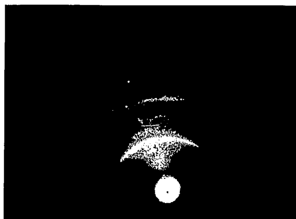
Figure 4.—Electron-diffraction pattern of \alpha -iron plus graphite from a new cast-iron ring abraded with No. 600 emery paper. Camera constant, 14.0. \times 2 .
