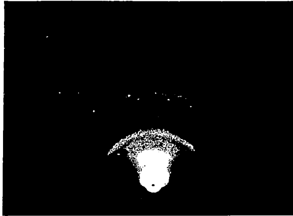
Figure 5.—Electron-diffraction pattern of graphite from a new cast-iron ring abraded then etched with 2-percent nital. Camera constant, 14.0. \times 2 .
