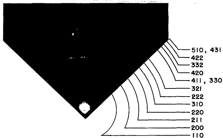
Figure 1.—Electron-diffraction pattern of \alpha -iron. Camera constant, 14.0. \times 2 .
