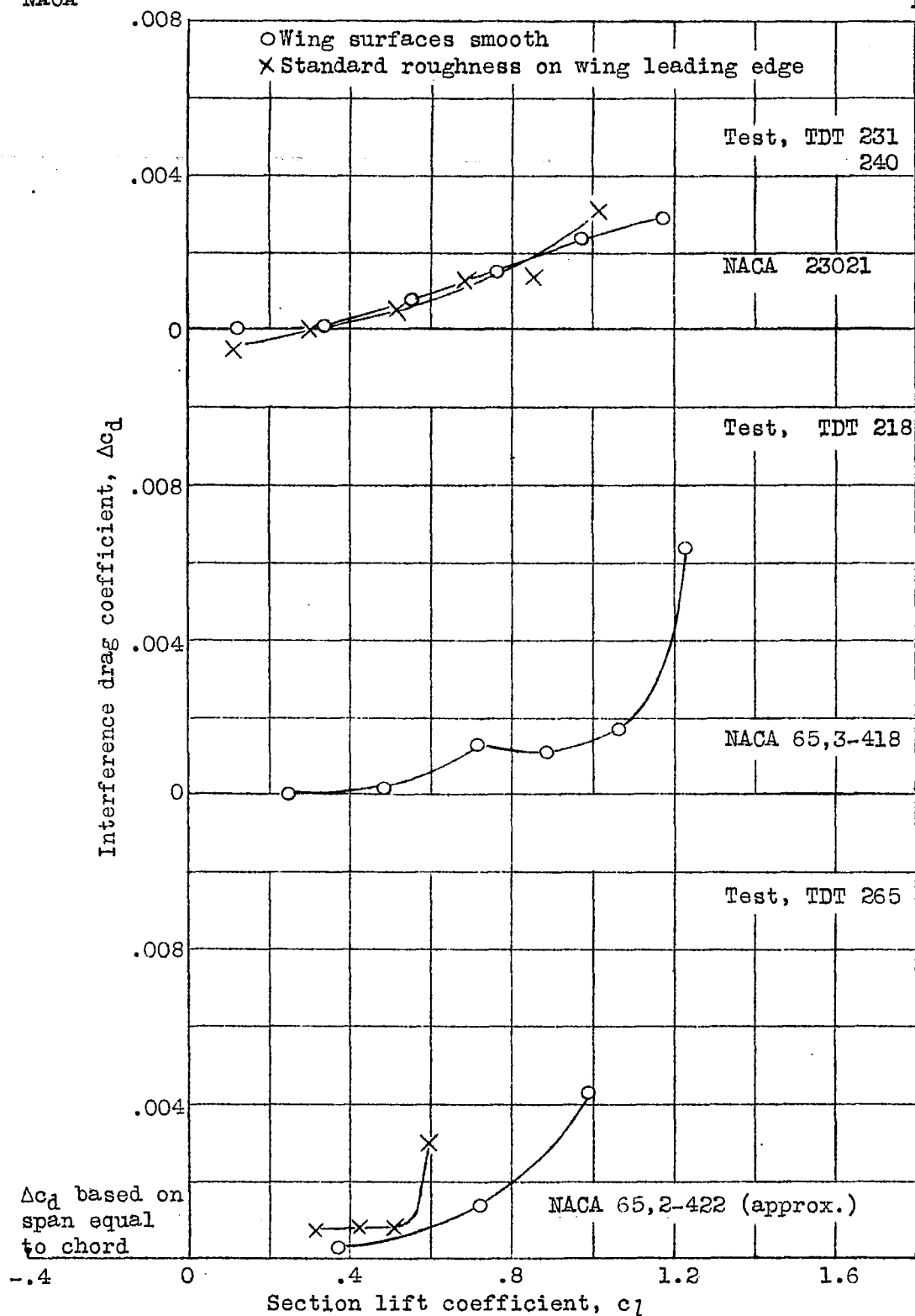
Figure 4.- Interference drag coefficients for three airfoils with intersecting flat plates. R=6 \times 10^6
