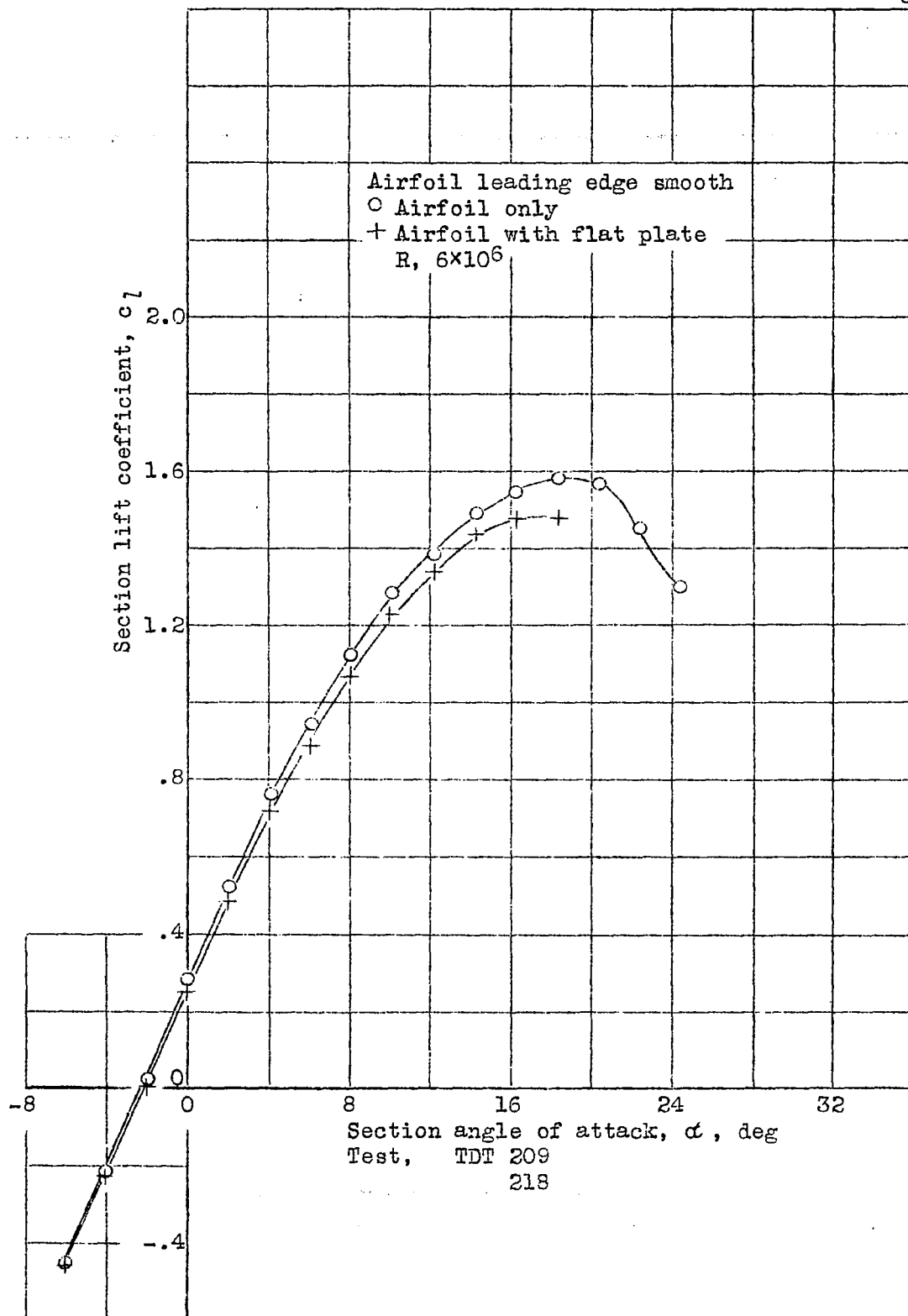
Figure 6.-- Lift characteristics of NACA 65,3-418 airfoil with and without intersecting flat plate.
