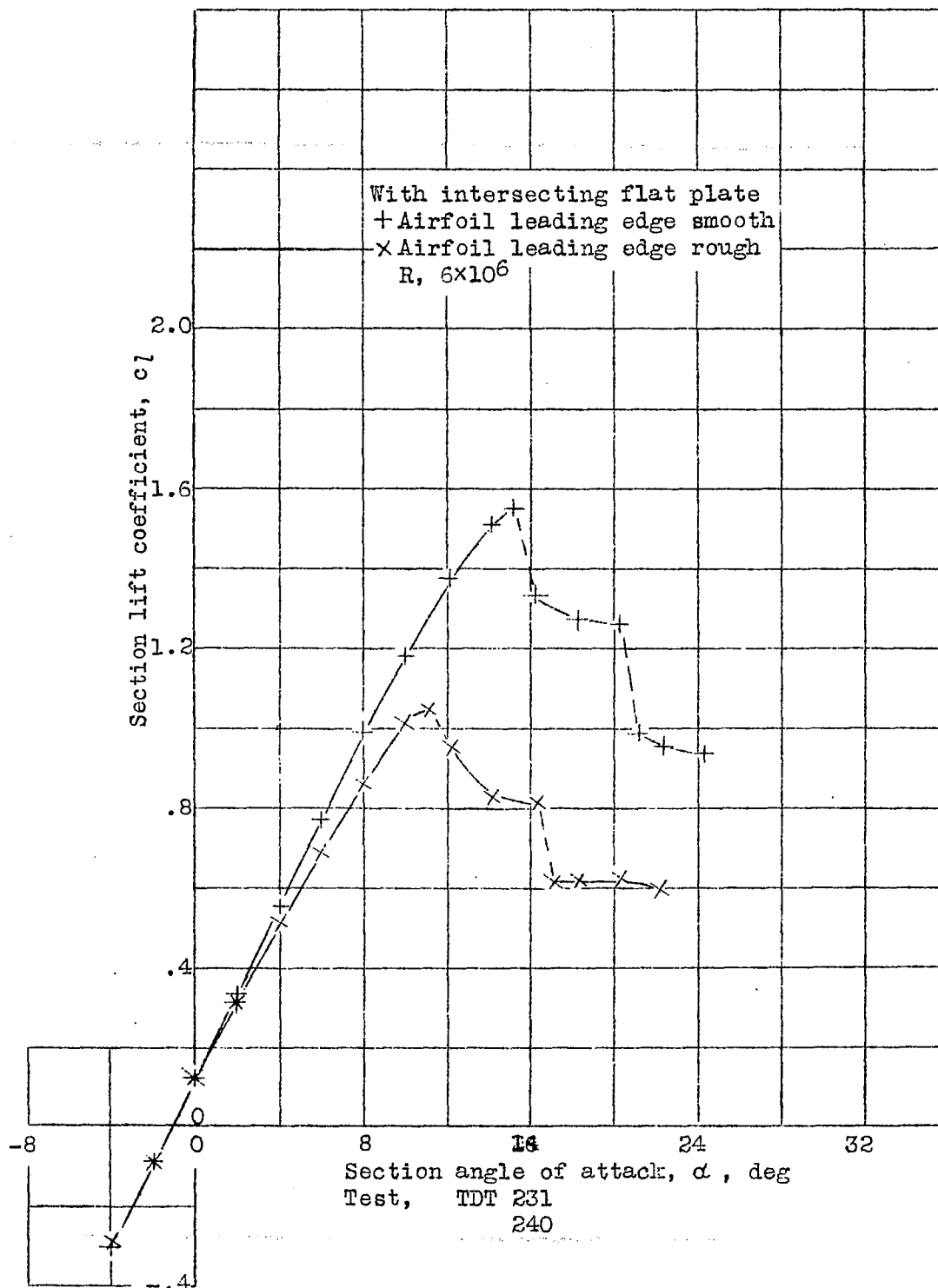
Figure 5.- Lift characteristics of NACA 23021 airfoil with intersecting flat plate.
