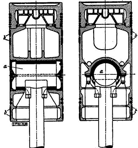
Figures 35 and 36.- Cooled piston of an opposed piston engine. Type M.A.N.
