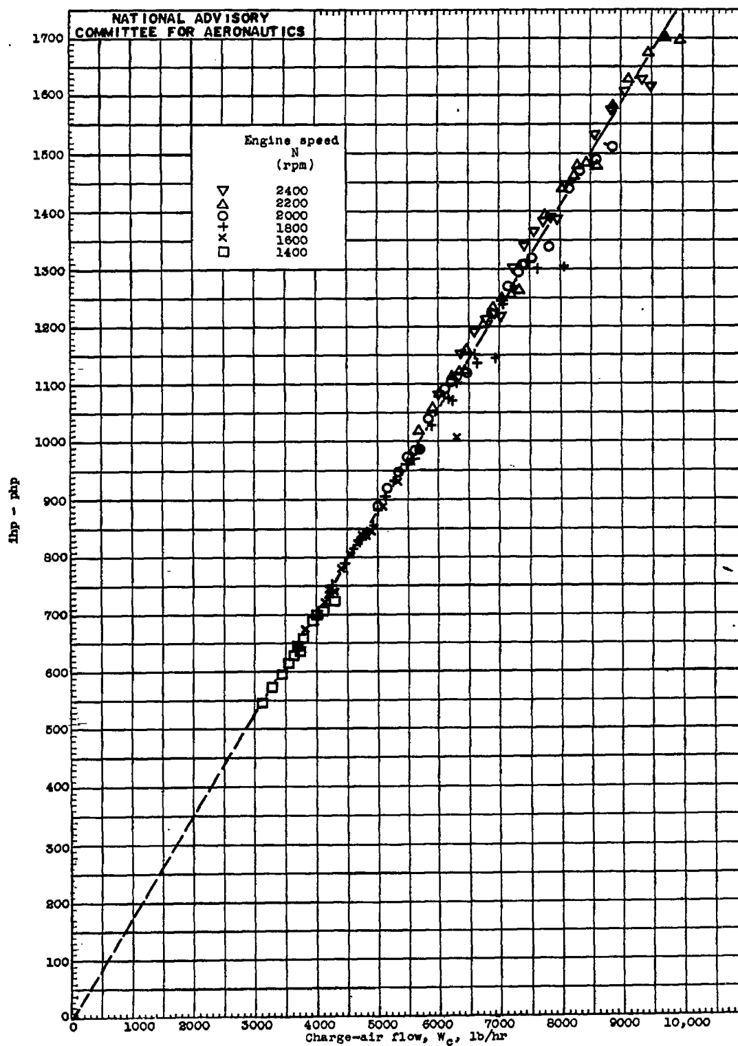
Figure 15. - Continued. Variation of ihp - php with charge-air flow for various engine speeds and values of p_e/p_m . Charge-air flow W_c and ihp - php corrected to a constant inlet-manifold mixture temperature T_m of 560^\circ R ; supercharger in low gear ratio (7.6 : 1).
