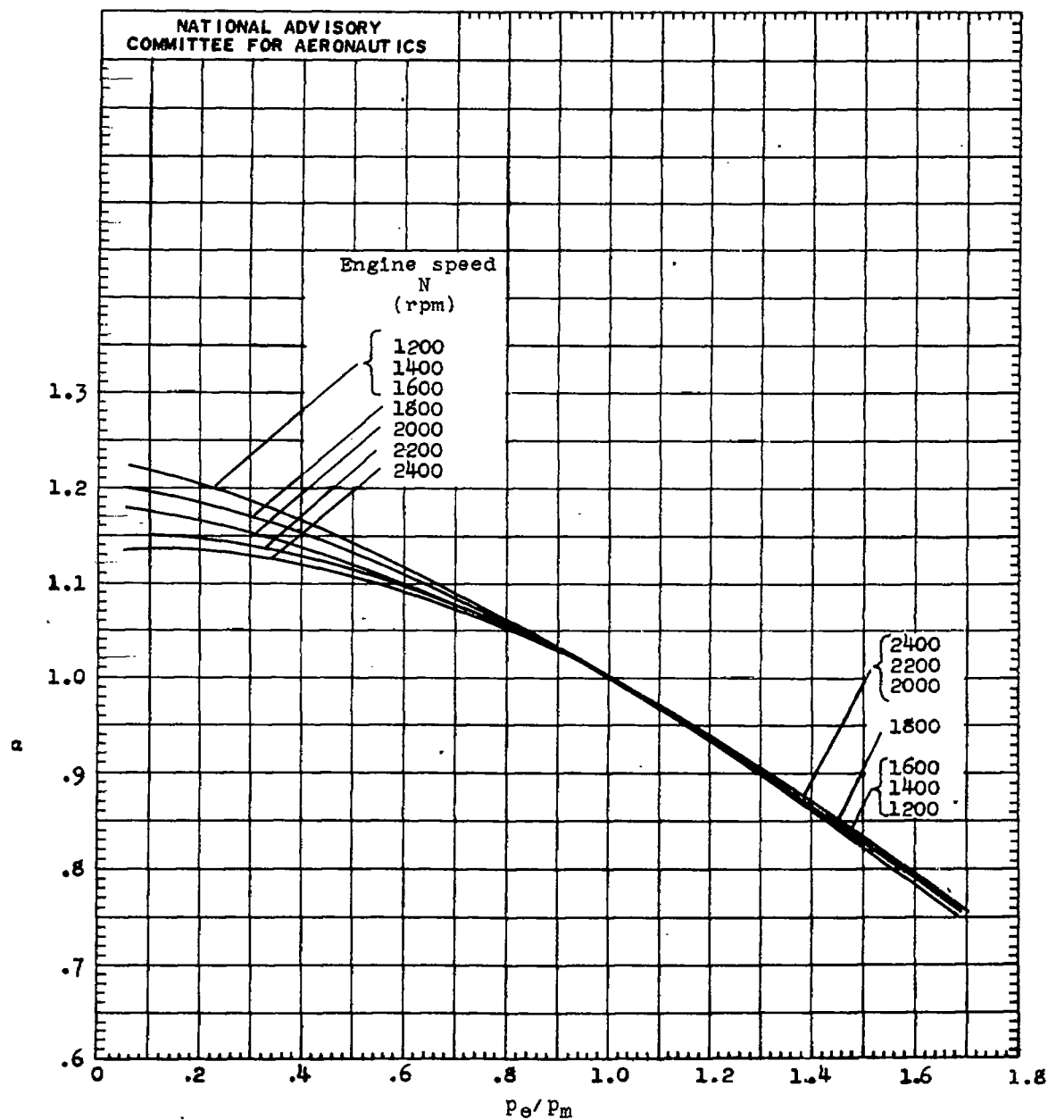
Figure 9. - Variation of \alpha with p_e/p_m for various engine speeds, fuel-air ratios, inlet-manifold pressures, and for high and low gear ratio.
