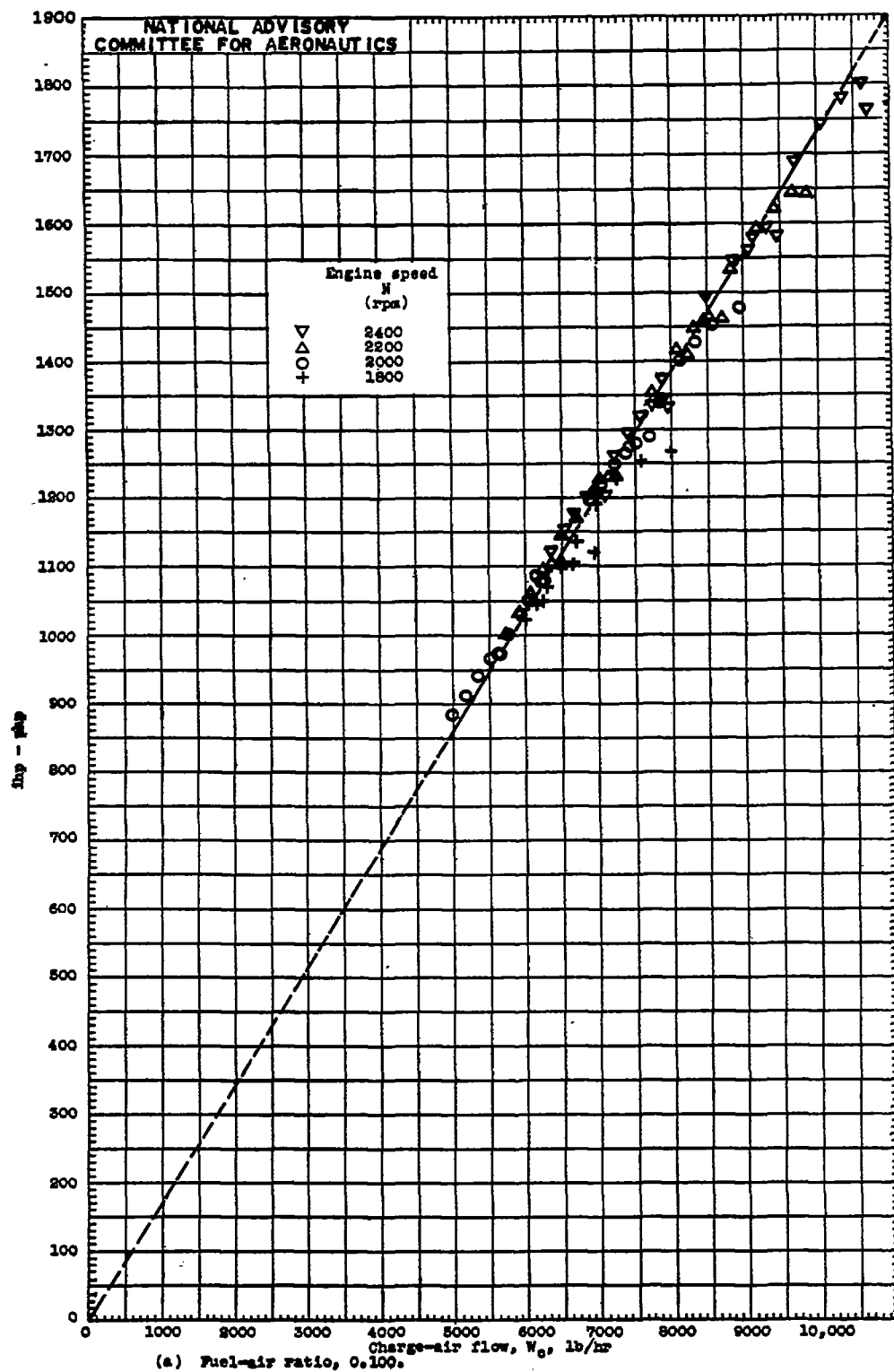
Figure 15. - Variation of ihp - php with charge-air flow for various engine speeds and values of p_e/p_m . Charge-air flow W_0 and ihp - php corrected to a constant inlet-manifold mixture temperature T_m of 660^\circ R ; supercharger in low gear ratio (7.6 : 1).
