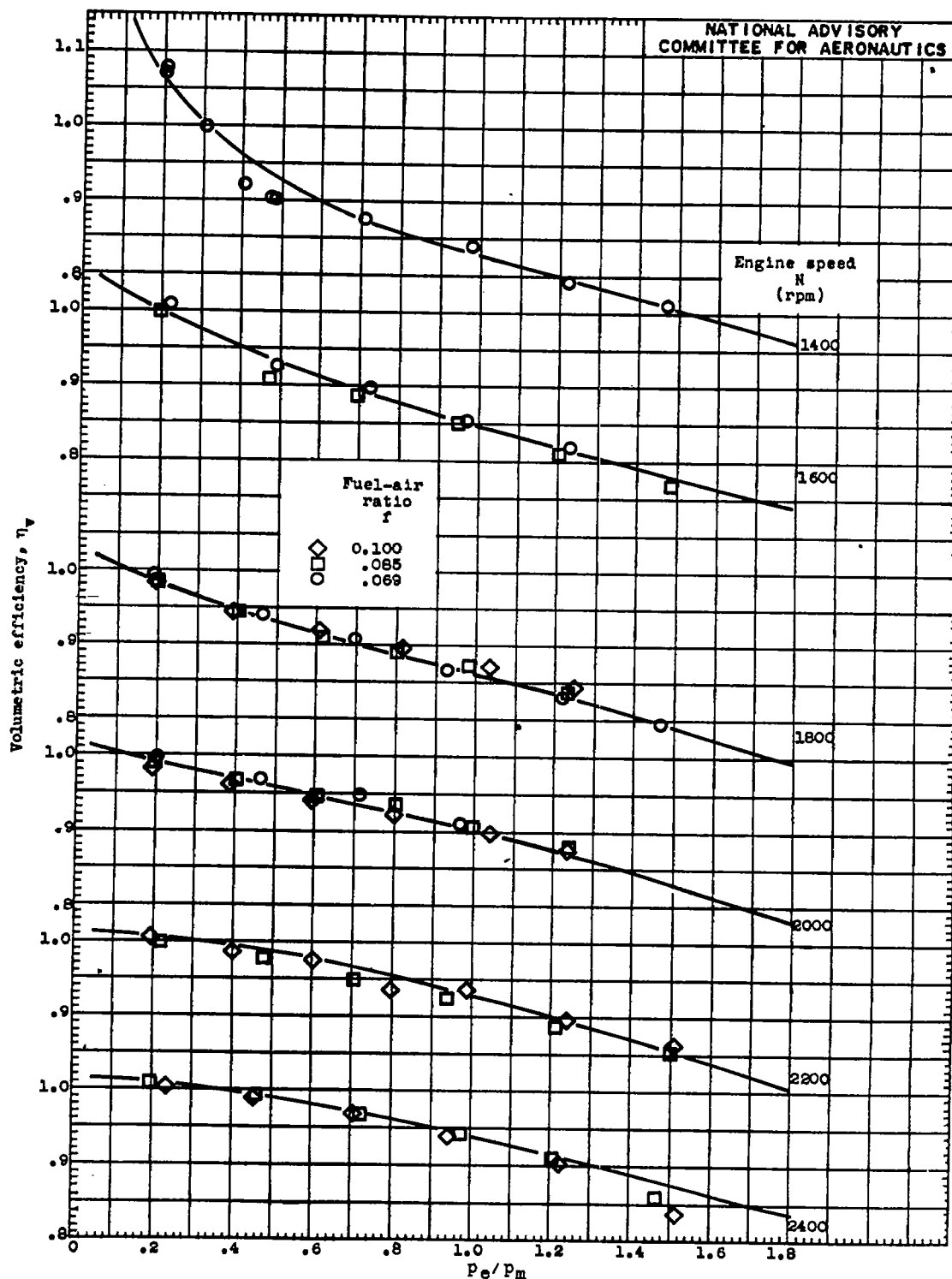
Figure 13. - Continued. Variation of volumetric efficiency \eta_v with P_e/P_m . Supercharger in low gear ratio (7.6 : 1) except where otherwise noted.
