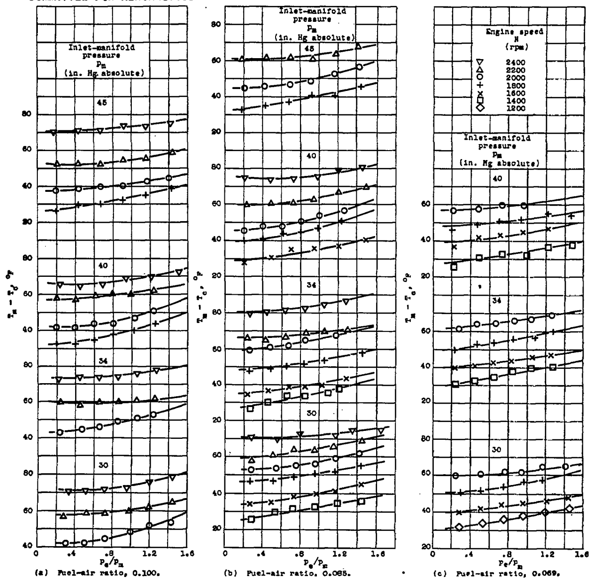
Figure 4.-- Variation of T_m - T_c with P_e/P_m with supercharger in low gear ratio (7.8 : 1).
