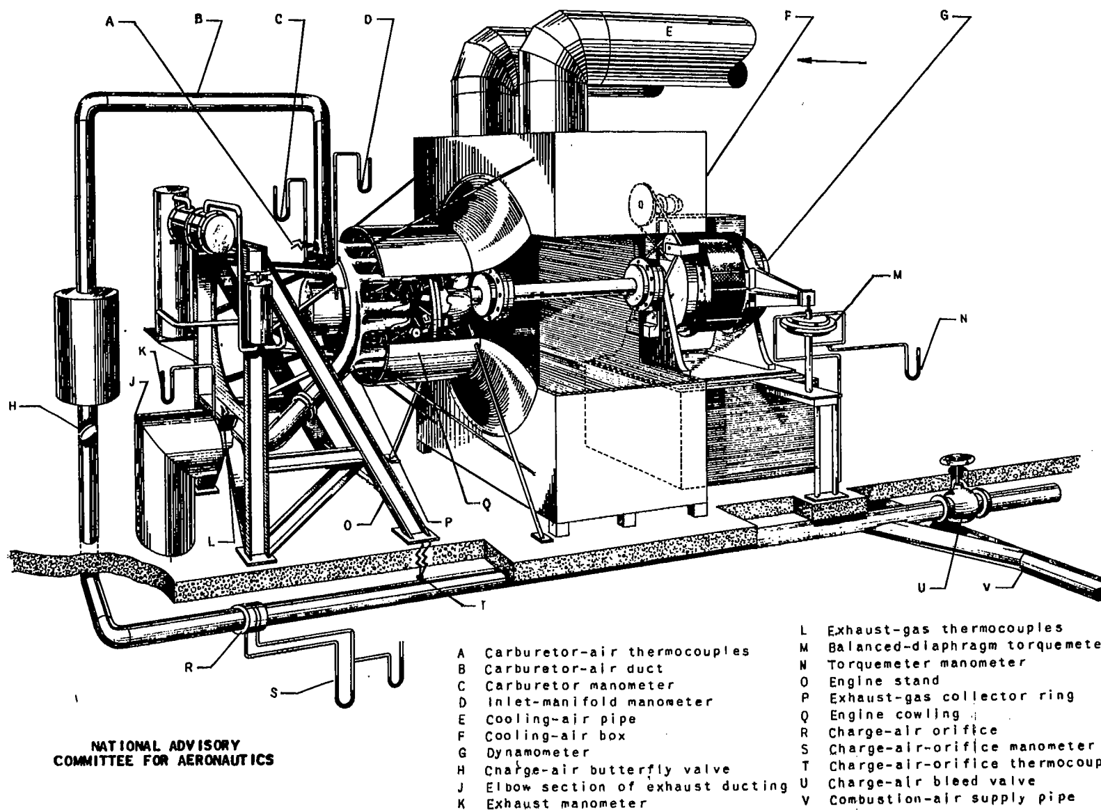
Figure 2. - Sketch of setup.
