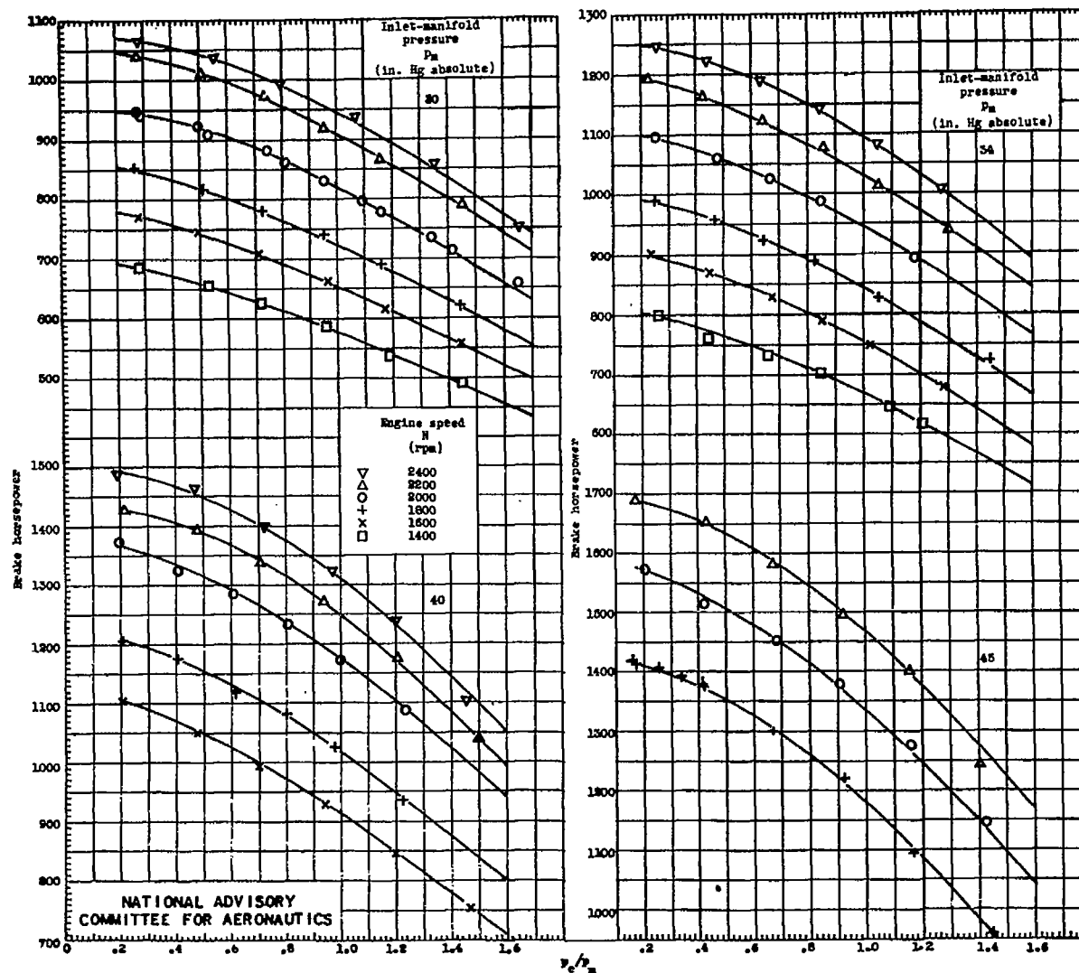
Figure 5. - Continued. Variation of brake horsepower with p_0/p_m . Brake horsepower corrected to constant carburetor-air temperature of 560° R; supercharger in low gear ratio (7.6 : 1).
