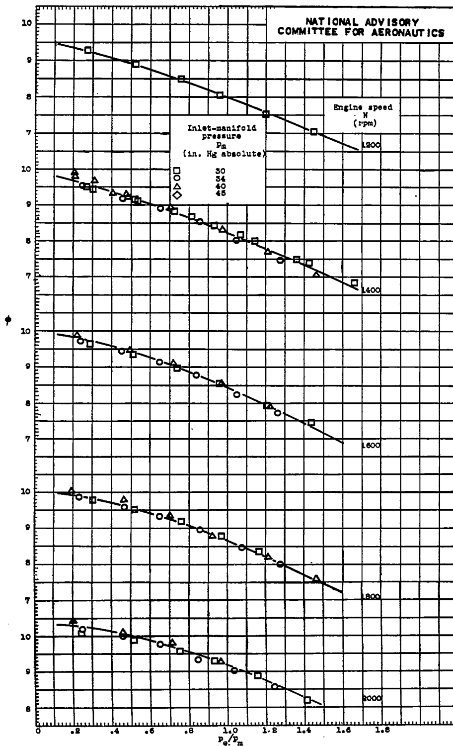
Figure 3. - Concluded. Variation of \phi with p_0/p_m . Values of \phi corrected to constant inlet-manifold mixture temperature T_m of 560° R; supercharger in low gear ratio (7.6 : 1) except where otherwise noted.
