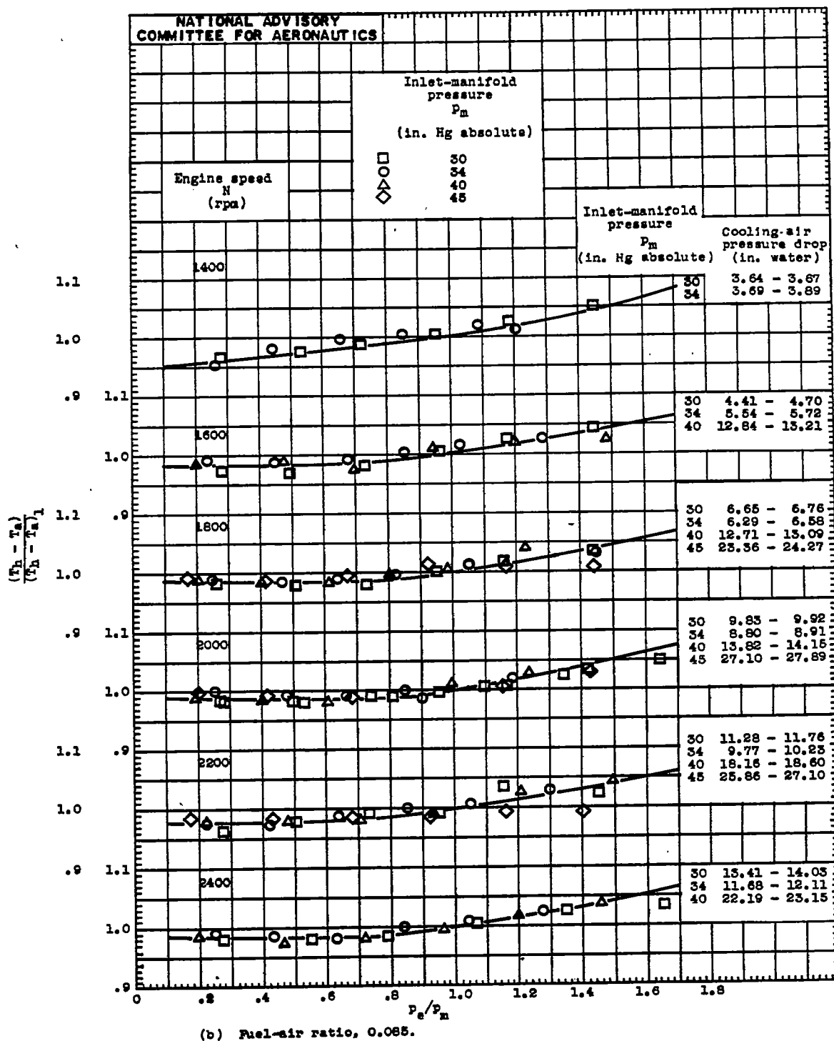
Figure 16. - Continued. Variation of \frac{(T_h - T_a)}{(T_h - T_a)_1} with P_e/P_m for constant engine speeds, fuel-air ratios, inlet-manifold pressures, and cooling-air pressure drops. Supercharger in low gear ratio (7.6 : 1).
