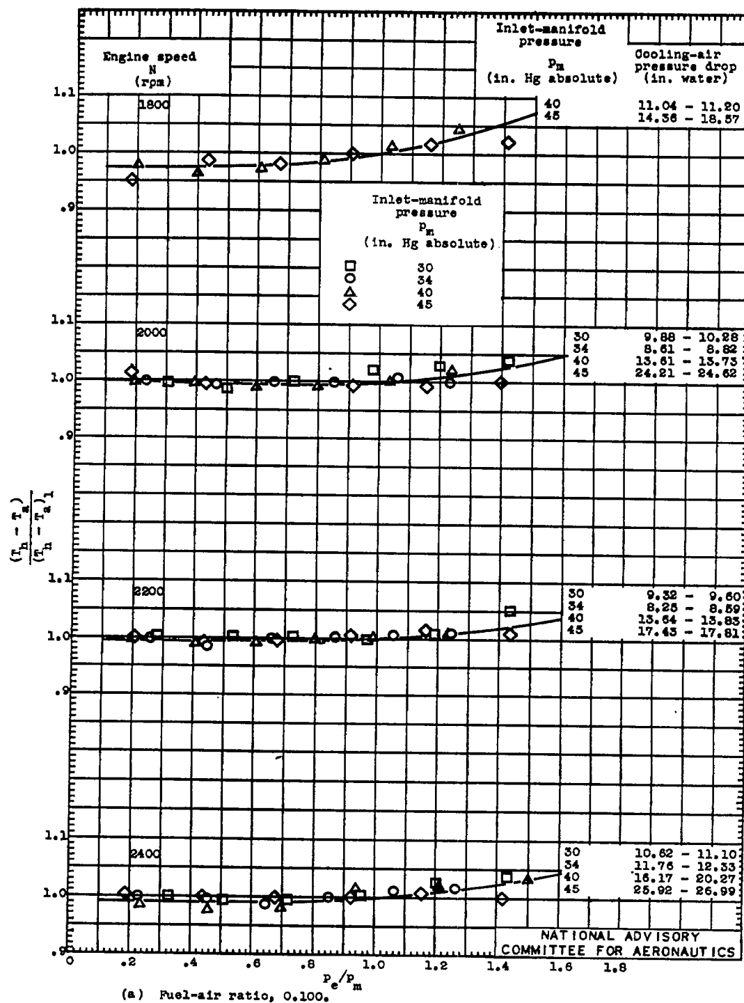
Figure 16. - Variation of \frac{(T_h - T_a)}{(T_h - T_a)_1} with p_e/p_m for constant engine speeds, fuel-air ratios, inlet-manifold pressures, and cooling-air pressure drops. Supercharger in low gear ratio (7.6 : 1).
