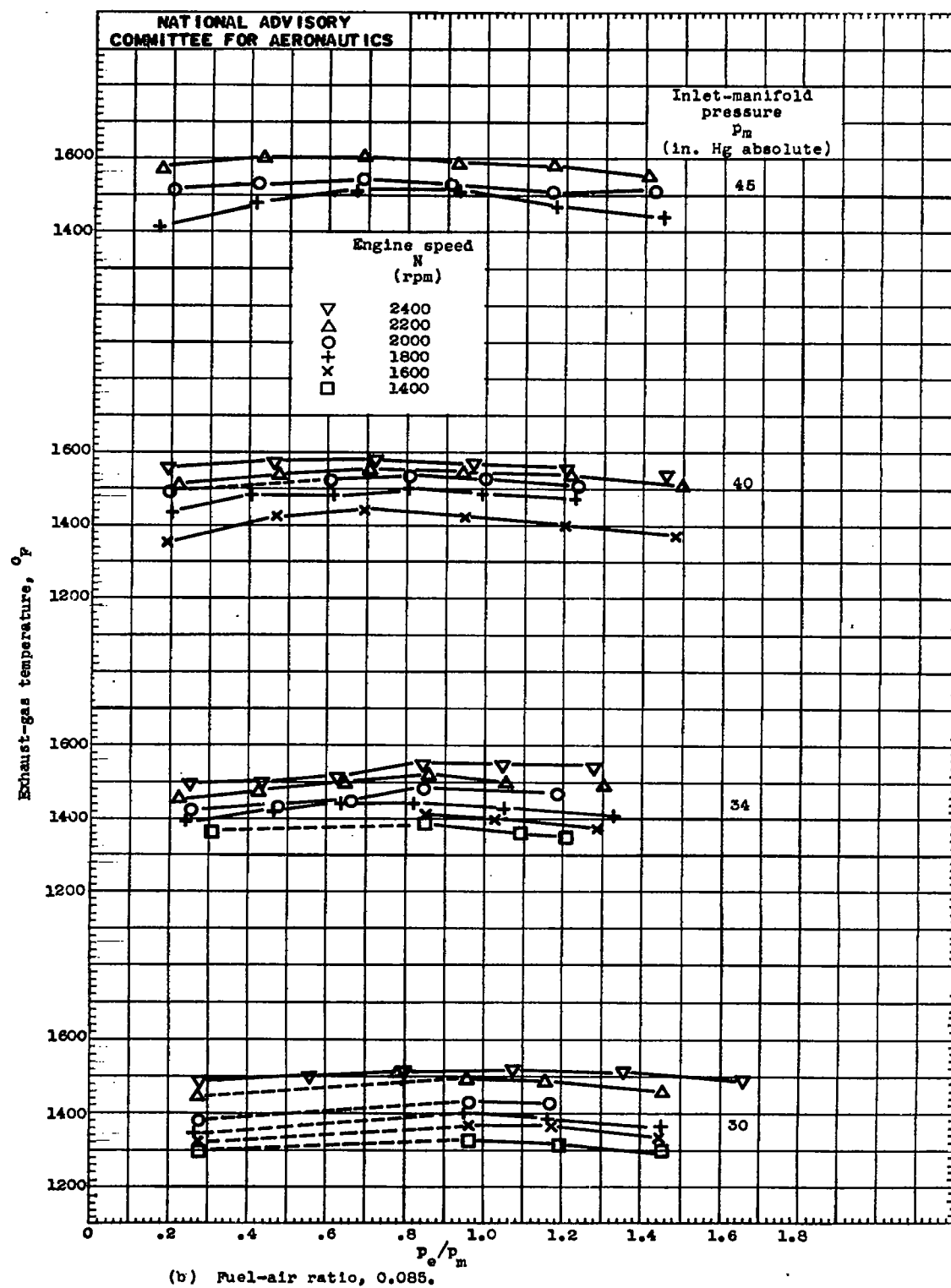
Figure 17. - Continued. Variation of exhaust-gas temperature with P_e/P_m for constant engine speeds, inlet-manifold pressures, and fuel-air ratios. Supercharger in low gear ratio (7.6 : 1).
