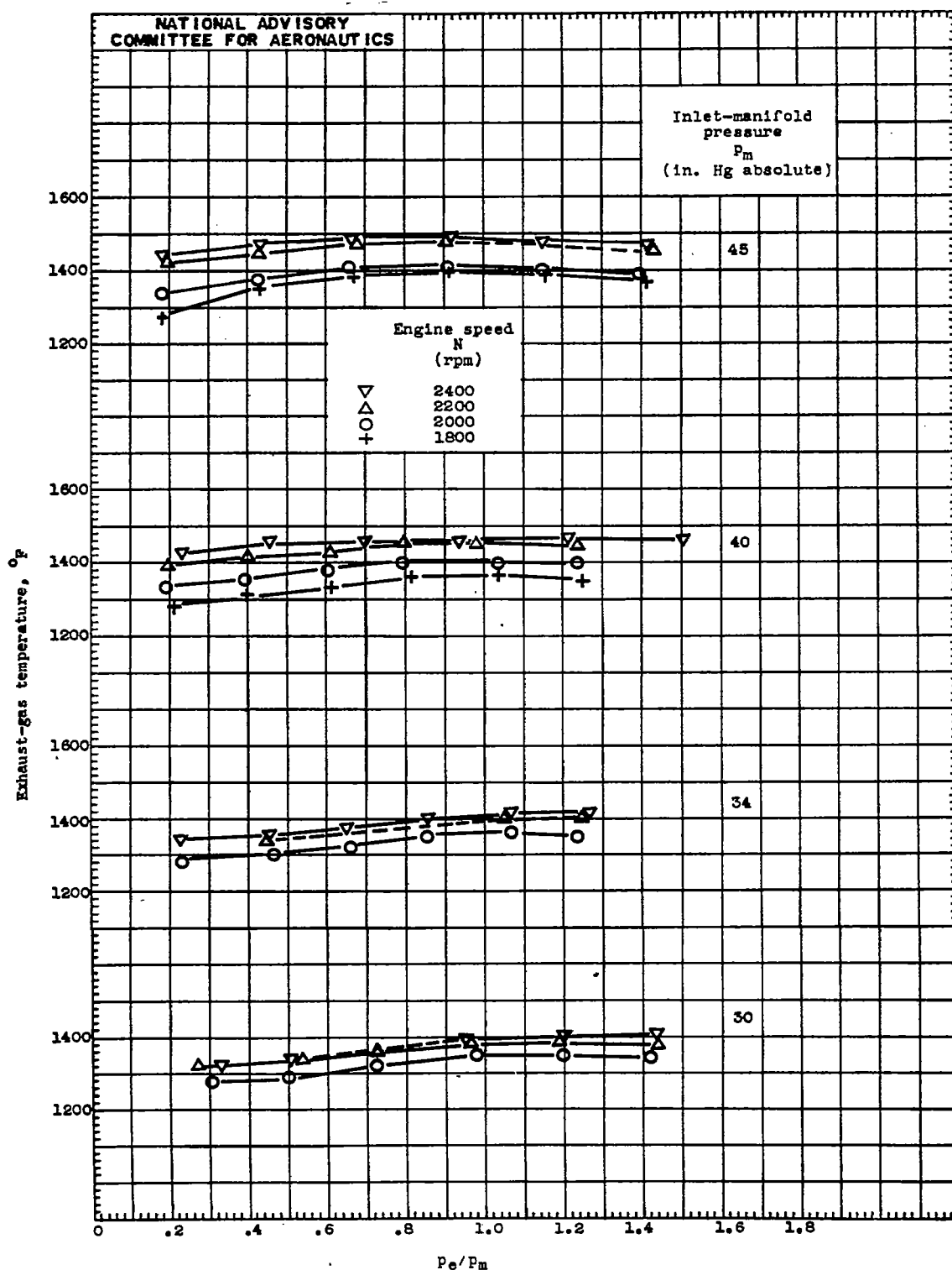
Figure 17. - Variation of exhaust-gas temperature with P_e/P_m for constant engine speeds, inlet-manifold pressures, and fuel-air ratios. Supercharger in low gear ratio (7.6 : 1).
