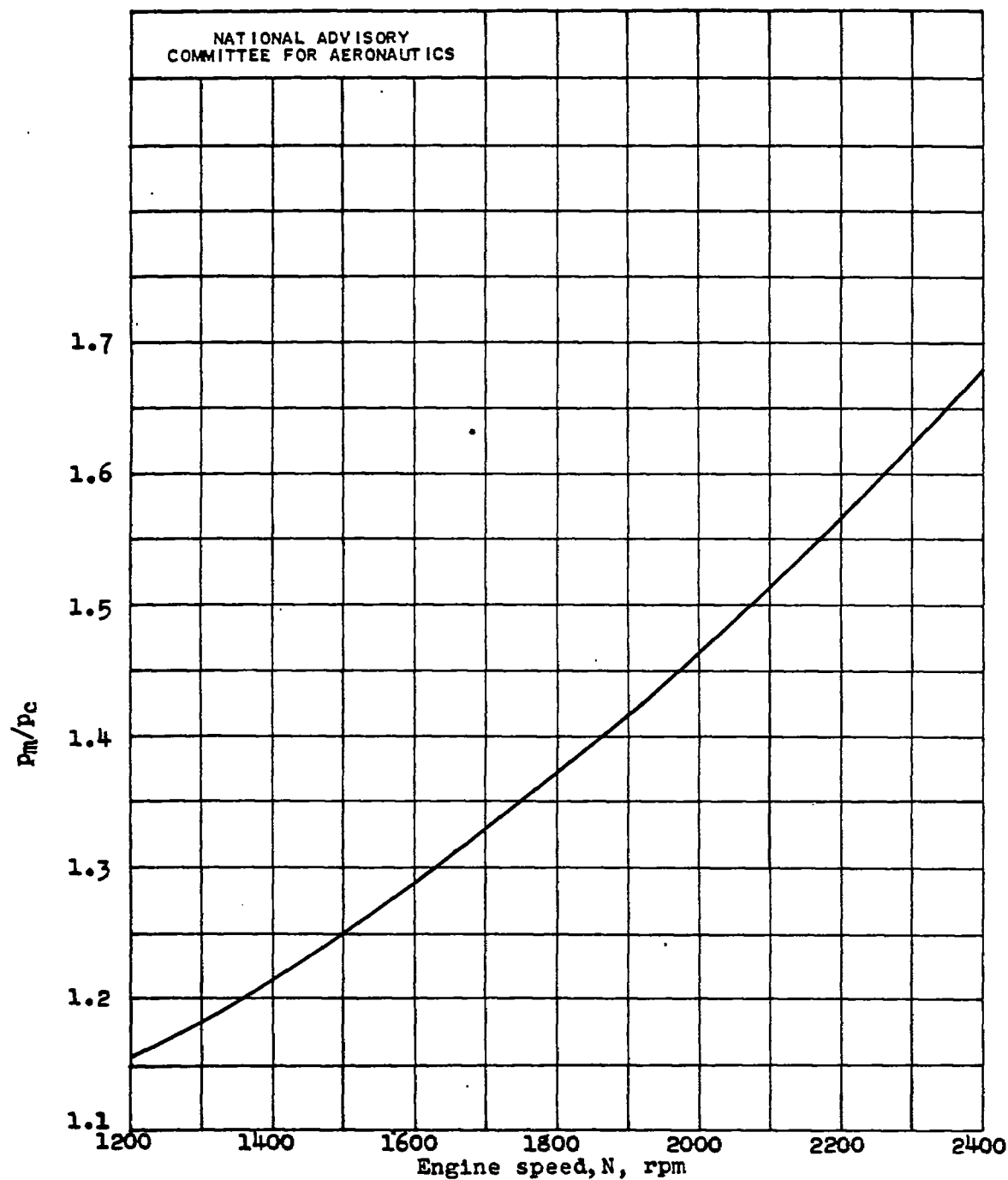
Figure 10. - Variation of ratio of inlet-manifold pressure to carburetor-inlet pressure P_m/P_c at full-open throttle with engine speed N . Carburetor-air temperature, 550^{\circ} R.
