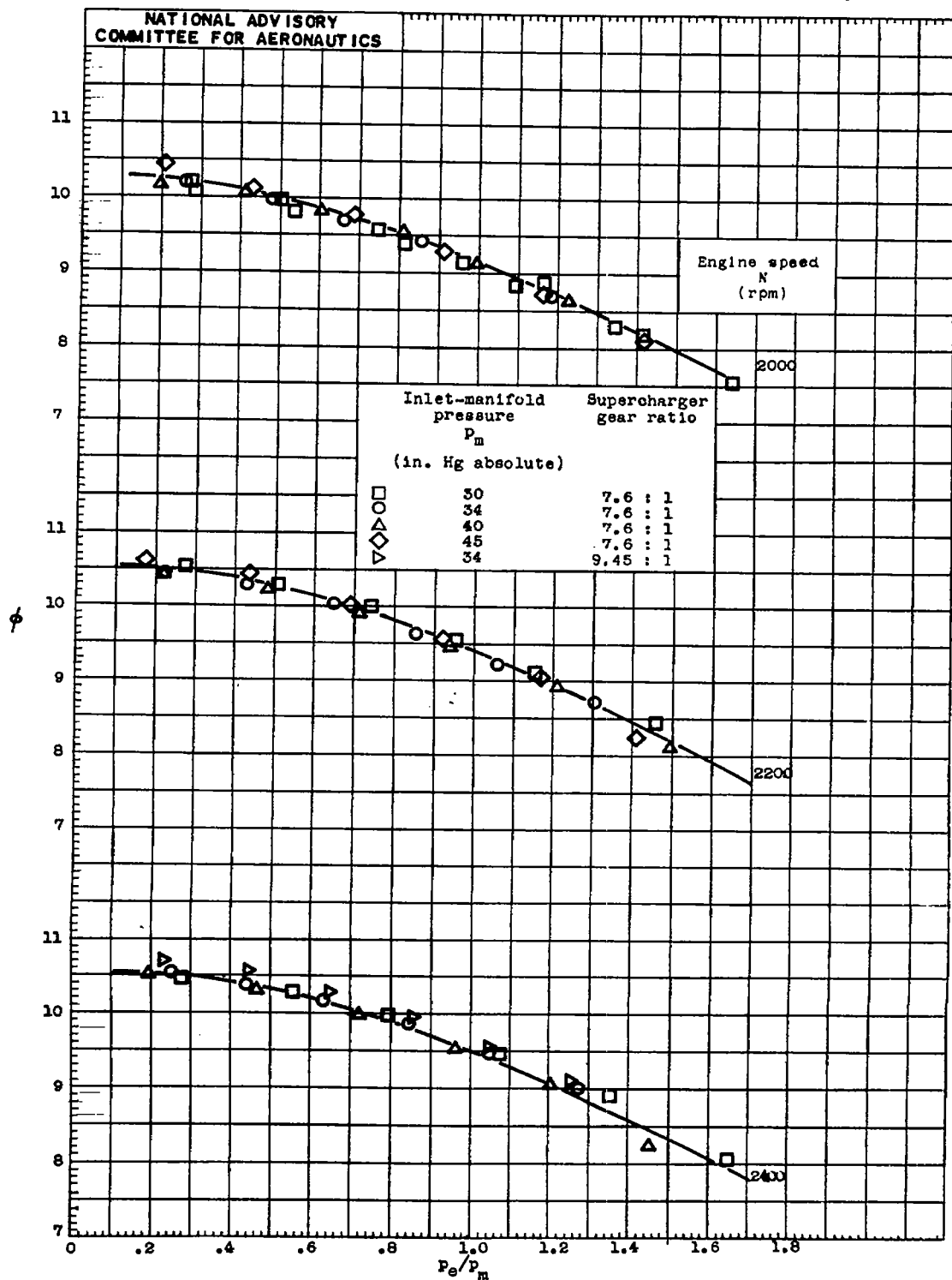
Figure 3. - Continued. Variation of \phi with P_e/P_m . Values of \phi corrected to constant inlet-manifold mixture temperature T_m of 560^\circ\text{R} ; supercharger in low gear ratio (7.6 : 1) except where otherwise noted.
