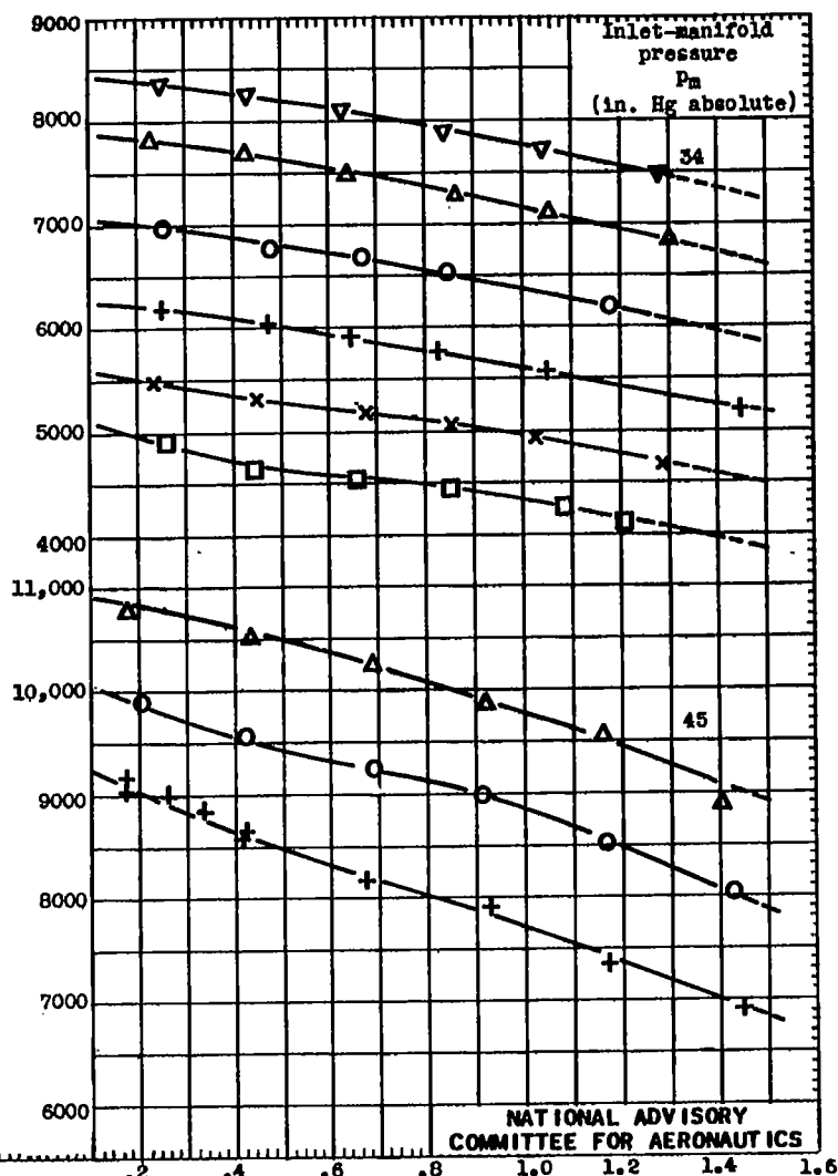
Figure 11. - Continued. Variation of charge-air flow W_o with P_o/P_m . Charge-air flow corrected to constant carburetor-air temperature of 550° R; supercharger in low gear ratio (7.6 : 1).
