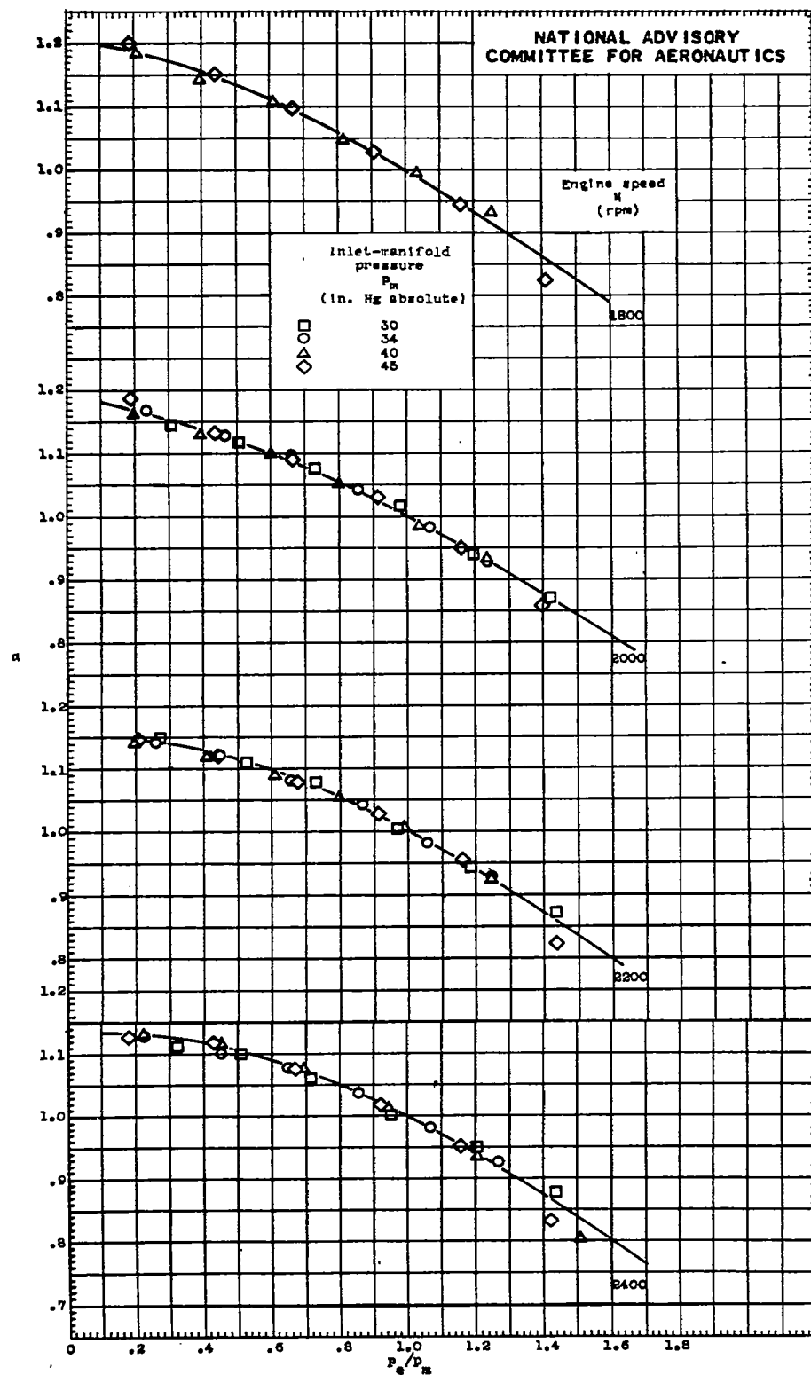
Figure 7. - Variation of a with p_e/p_m . Supercharger in low gear ratio (7.6 : 1).
