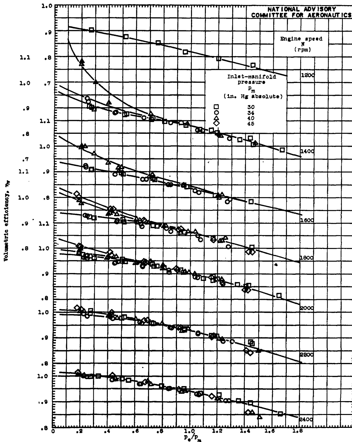
Figure 14. - Variation of volumetric efficiency \eta_v with P_e/P_m for constant engine speeds, inlet-manifold pressures, and three fuel-air ratios. Supercharger in low gear ratio (7.6 : 1).
