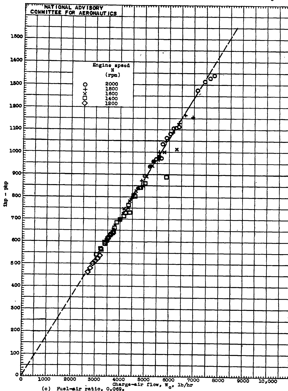
Figure 15. - Concluded. Variation of ihp - php with charge-air flow for various engine speeds and values of P_0/P_m . Charge-air flow W_c and ihp - php corrected to a constant inlet-manifold mixture temperature T_m of 660^\circ R ; supercharger in low gear ratio (7.6 : 1).
