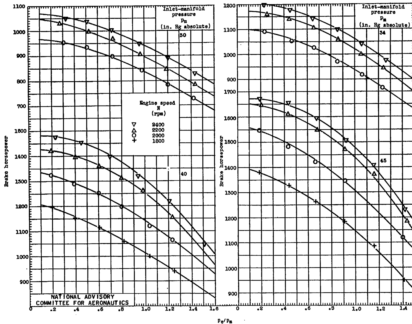
Figure 5. - Variation of brake horsepower with p_0/p_m . Brake horsepower corrected to constant carburetor-air temperature of 550° R; supercharger in low gear ratio (7.8 : 1).
