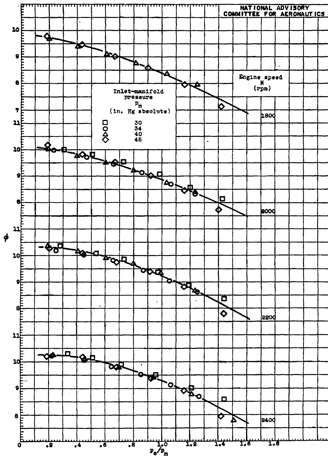
Figure 3. - Variation of \phi with P_e/P_m . Values of \phi corrected to constant inlet-manifold mixture temperature T_m of 560° R; supercharger in low gear ratio (7.6 : 1) except where otherwise noted.
