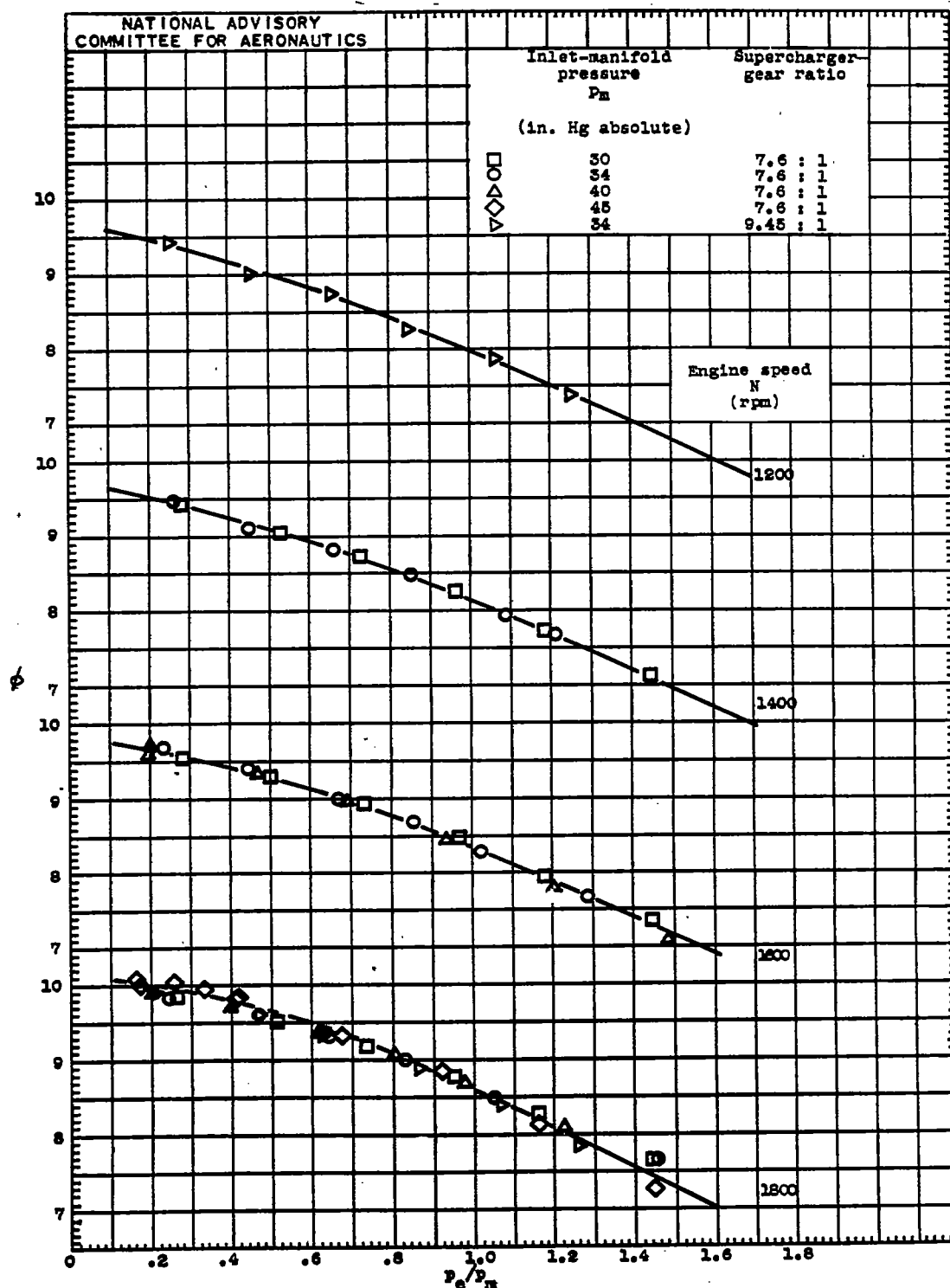
Figure 3. - Continued. Variation of \phi with P_e/P_m . Values of \phi corrected to constant inlet-manifold mixture temperature T_m of 660^\circ R ; supercharger in low gear ratio (7.6 : 1) except where otherwise noted.
