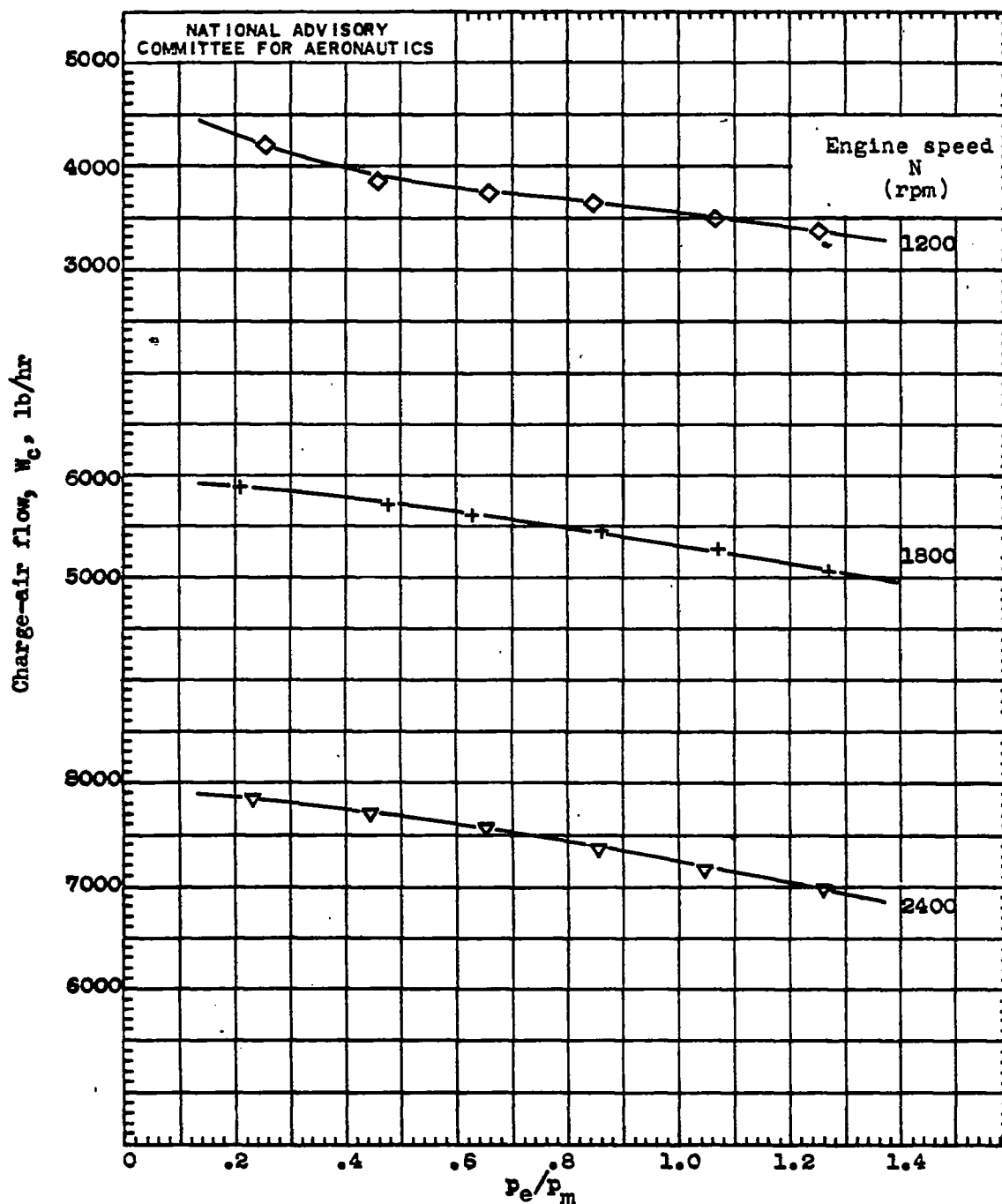
Figure 12. - Variation of charge-air flow W_c with p_e/p_m at constant inlet-manifold pressure of 34 inches mercury absolute and with supercharger in high gear ratio (9.45 : 1). Charge-air flow corrected to constant carburetor-air temperature of 550° R; fuel-air ratio, 0.085.
