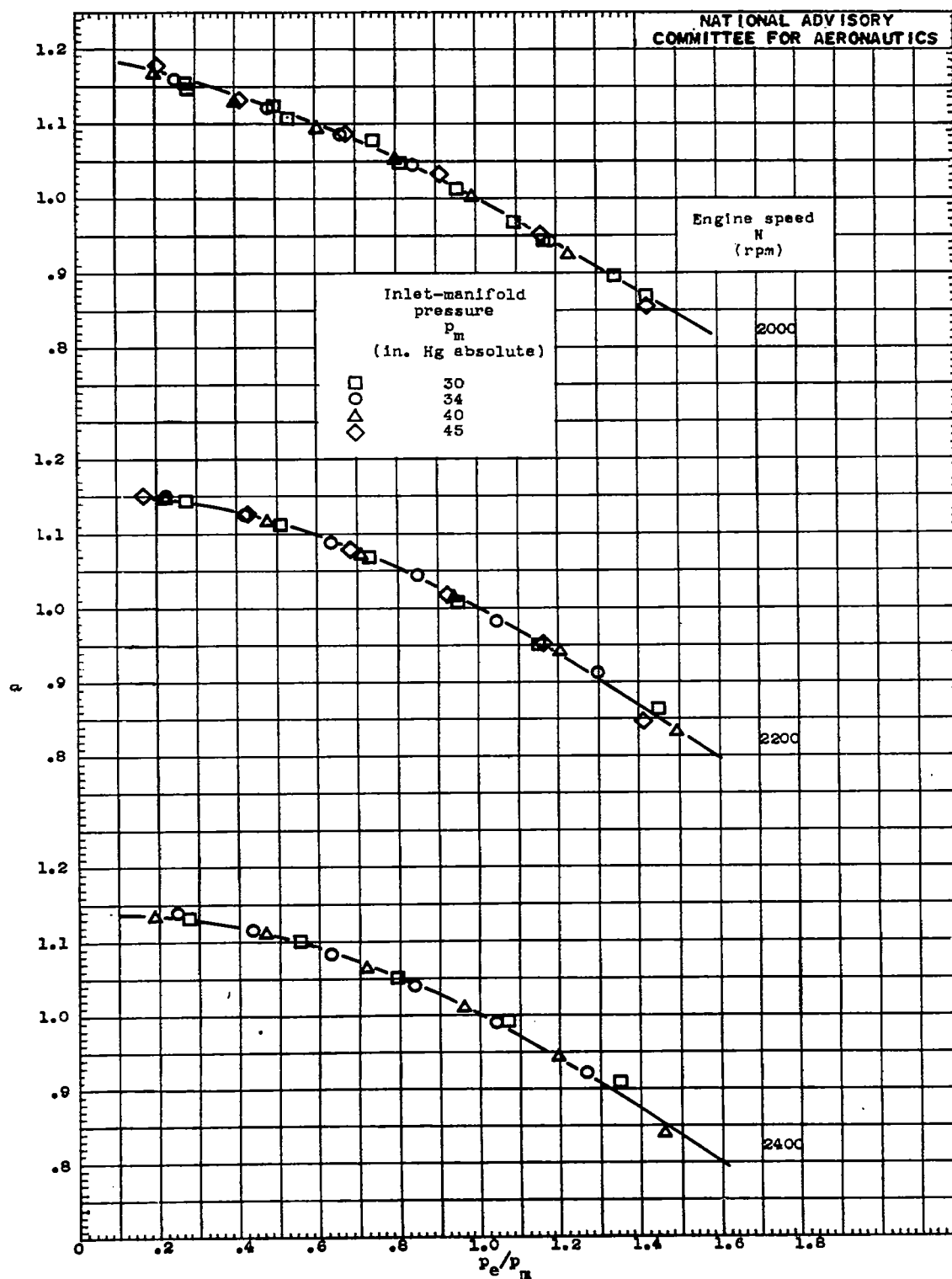
Figure 7. - Continued. Variation of \alpha with P_e/P_m . Supercharger in low gear ratio (7.6 : 1).
