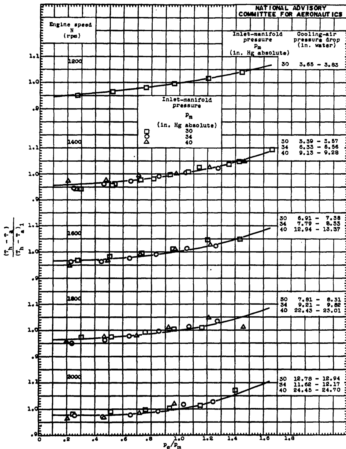
Figure 16. - Concluded. Variation of \frac{(T_h - T_a)}{(T_h - T_a)_1} with p_e/p_m for constant engine speeds, fuel-air ratios, inlet-manifold pressures, and cooling-air pressure drops. Supercharger in low gear ratio (7.6 : 1).
