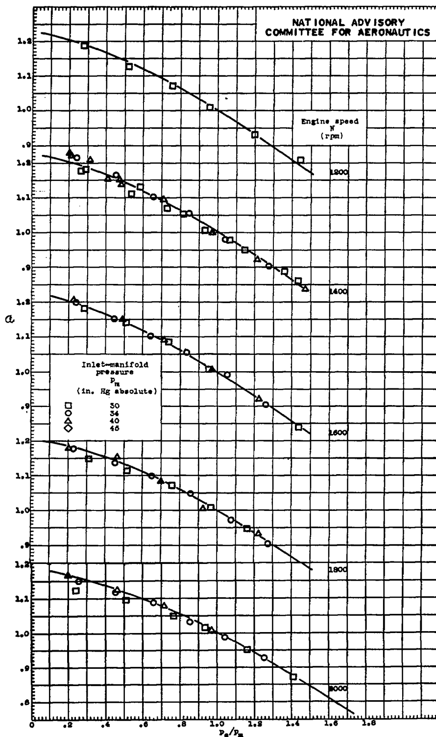
Figure 7. - Concluded. Variation of a with p_0/p_m . Supercharger in low gear ratio (7.6 : 1).
