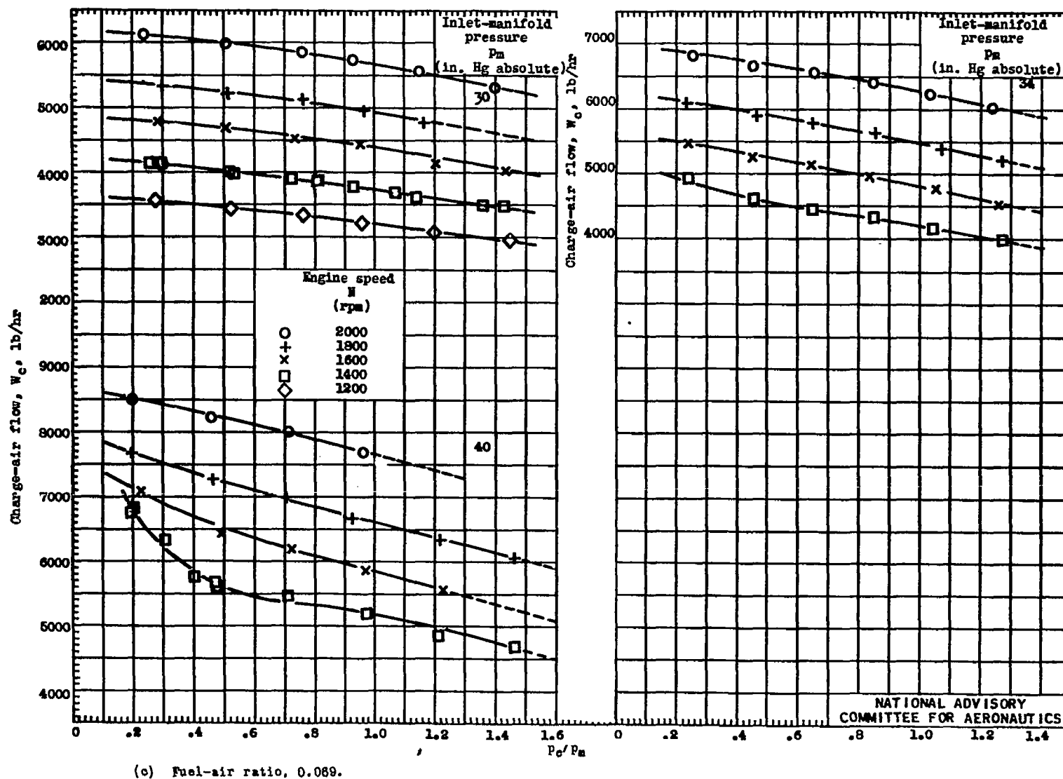
Figure 11. - Concluded. Variation of charge-air flow W_c with p_c/p_m . Charge-air flow corrected to constant carburetor-air temperature of 550° R; supercharger in low gear ratio (7.6 : 1).
