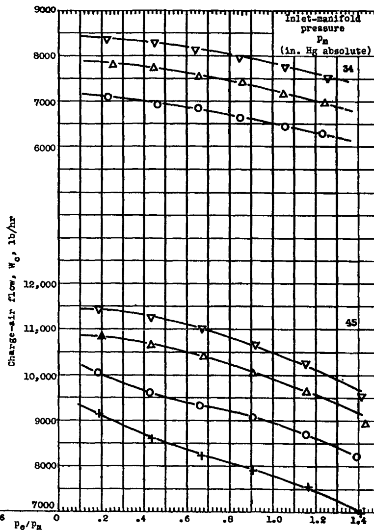
Figure 11. - Variation of charge-air flow W_c with P_0/P_m . Charge-air flow corrected to constant carburetor-air temperature of 550° R; supercharger in low gear ratio (7.6 : 1).
