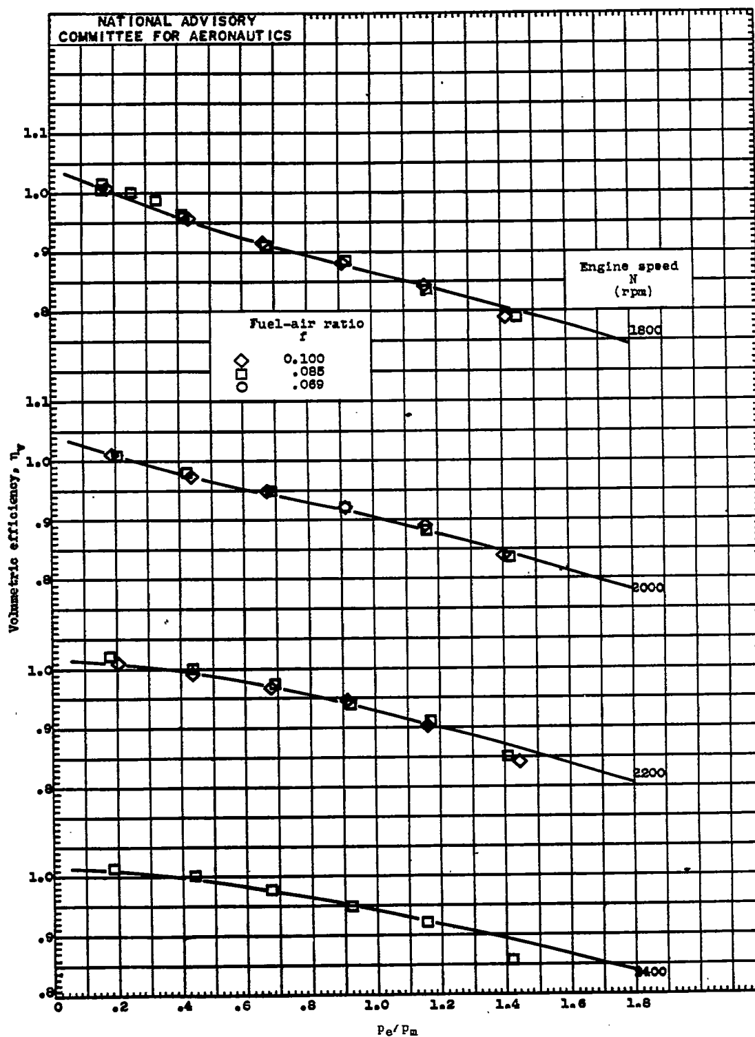
Figure 13. - Concluded. Variation of volumetric efficiency \eta_v with P_e/P_m . Supercharger in low gear ratio (7.8 : 1) except where otherwise noted.
