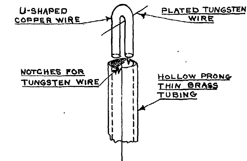
(d) EXPLODED MAGNIFIED VIEW OF CONNECTION TO PRONG
