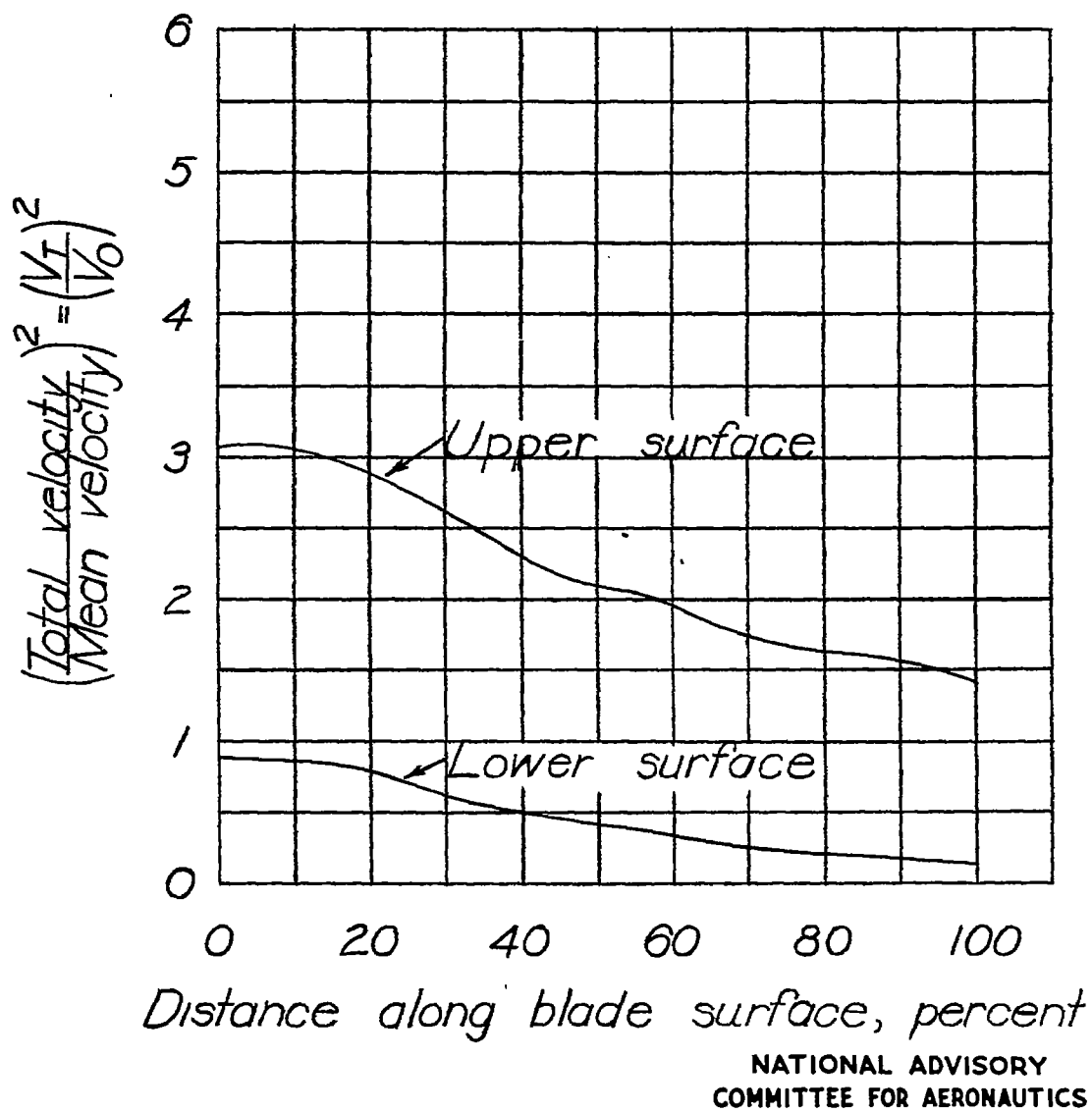
Figure 5.- Pressure distribution on airfoil derived in example I.
