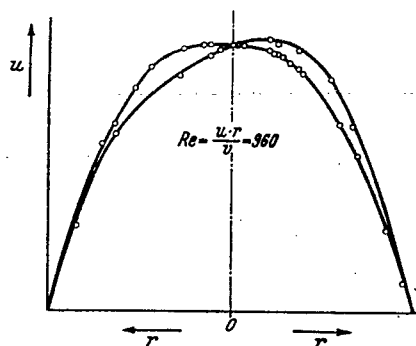
Figure 9.- Scatter of the velocity profile at the inlet. Laminar velocity profiles photographically obtained under equal test conditions.
