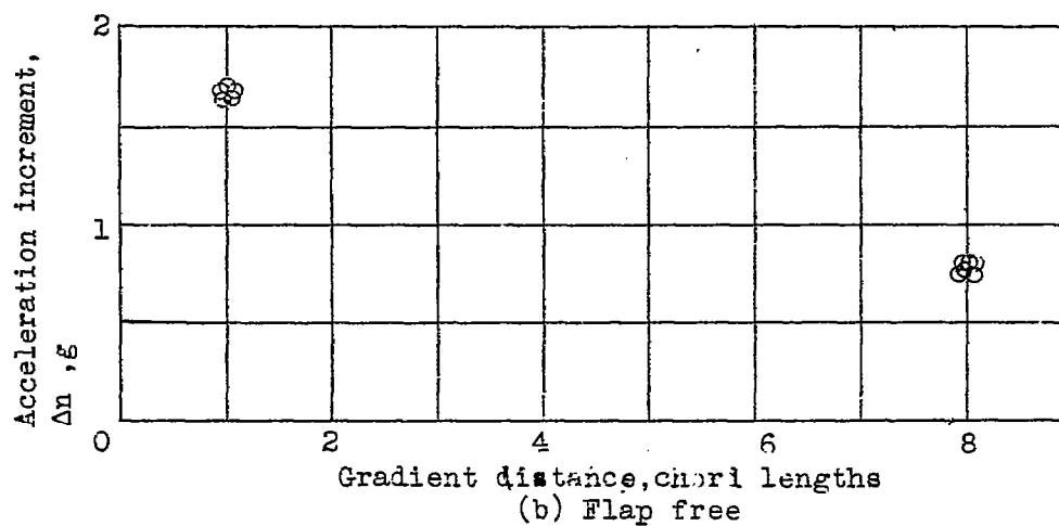
Figure 7.- Variation of acceleration increment with gradient distance.
