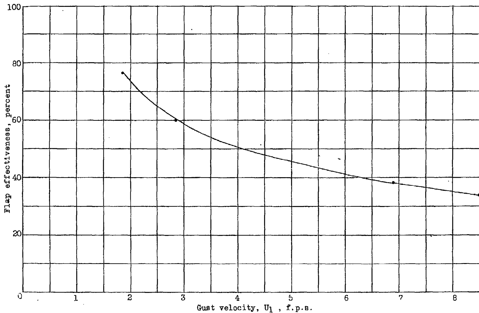
Figure 11.- Variation of flap effectiveness with gust velocity for an 8-chord-length gust.
