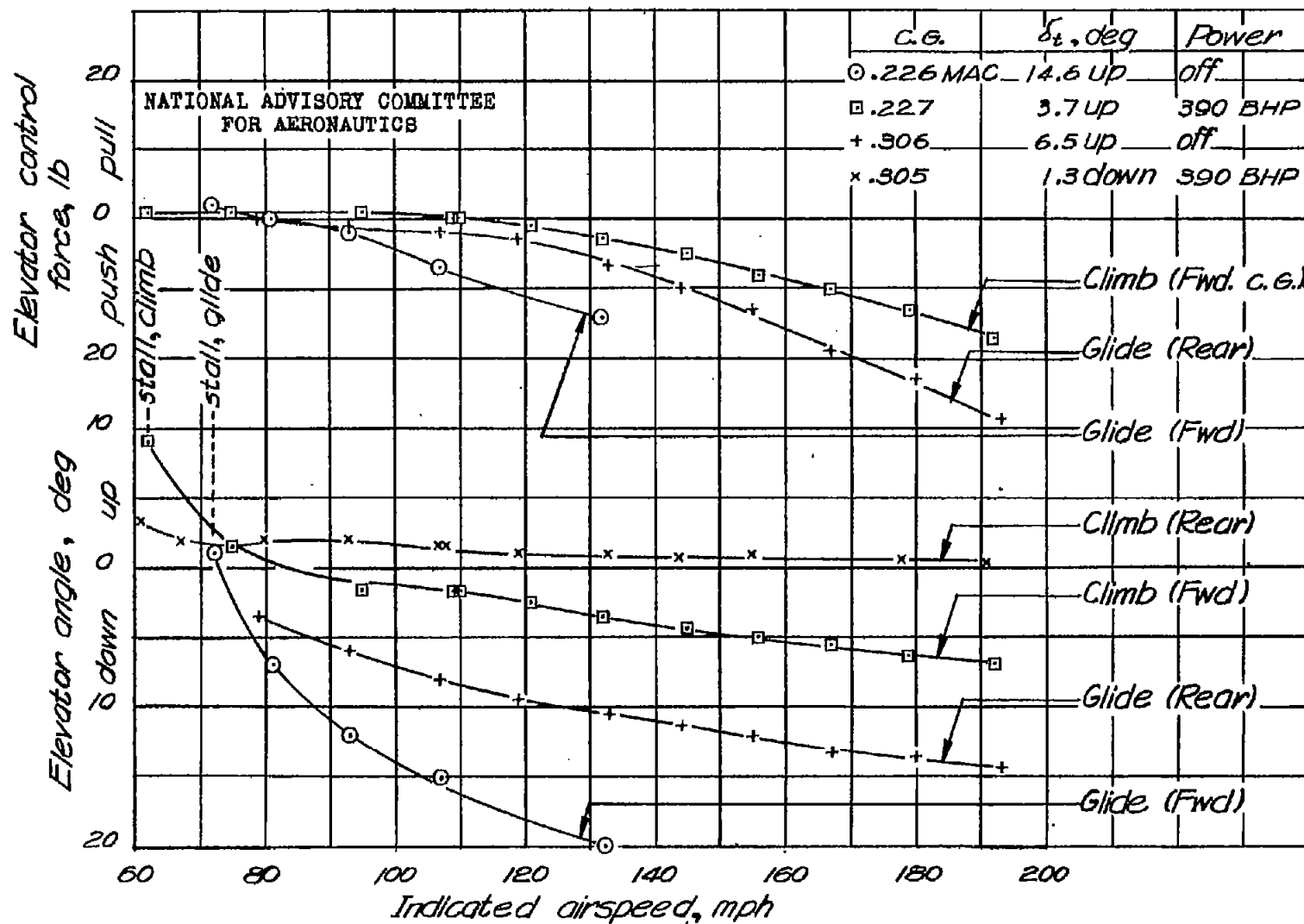
Figure 8.-Static longitudinal-stability characteristics. Flaps up.
