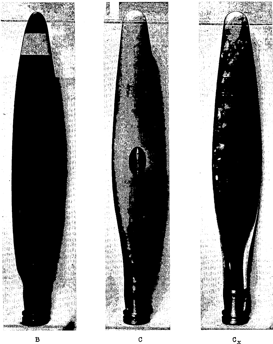
Figure 8.- One blade of each of the three 10-foot-diameter 3-blade propellers used.
