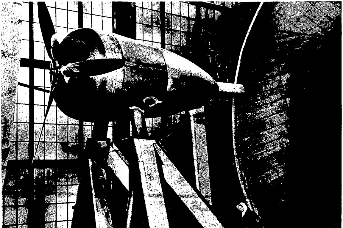
Figure 3.- Set-up 1, nose 2, nacelle 1 with propeller and tail pump in place. The results discussed in this report were obtained with an afterbody having a pointed tail, as shown in fig. 1.
