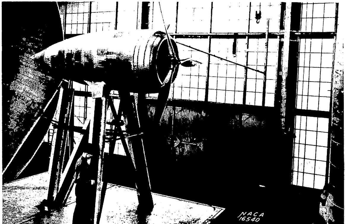
Figure 7.- Set-up 2, nose 1, nacelle 1 with a 1\frac{1}{2} -inch slot opening. The results discussed in this report were obtained with all slots closed and faired.
