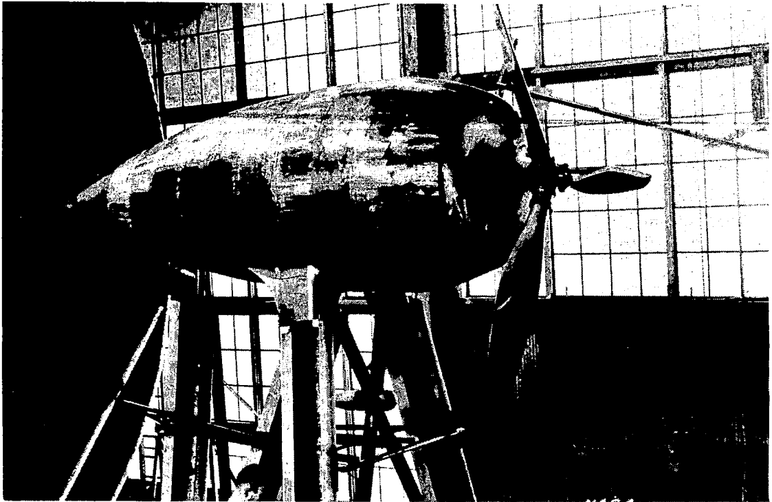
Figure 6.- Set-up 2, nose 5, nacelle 1 with propeller in place.
