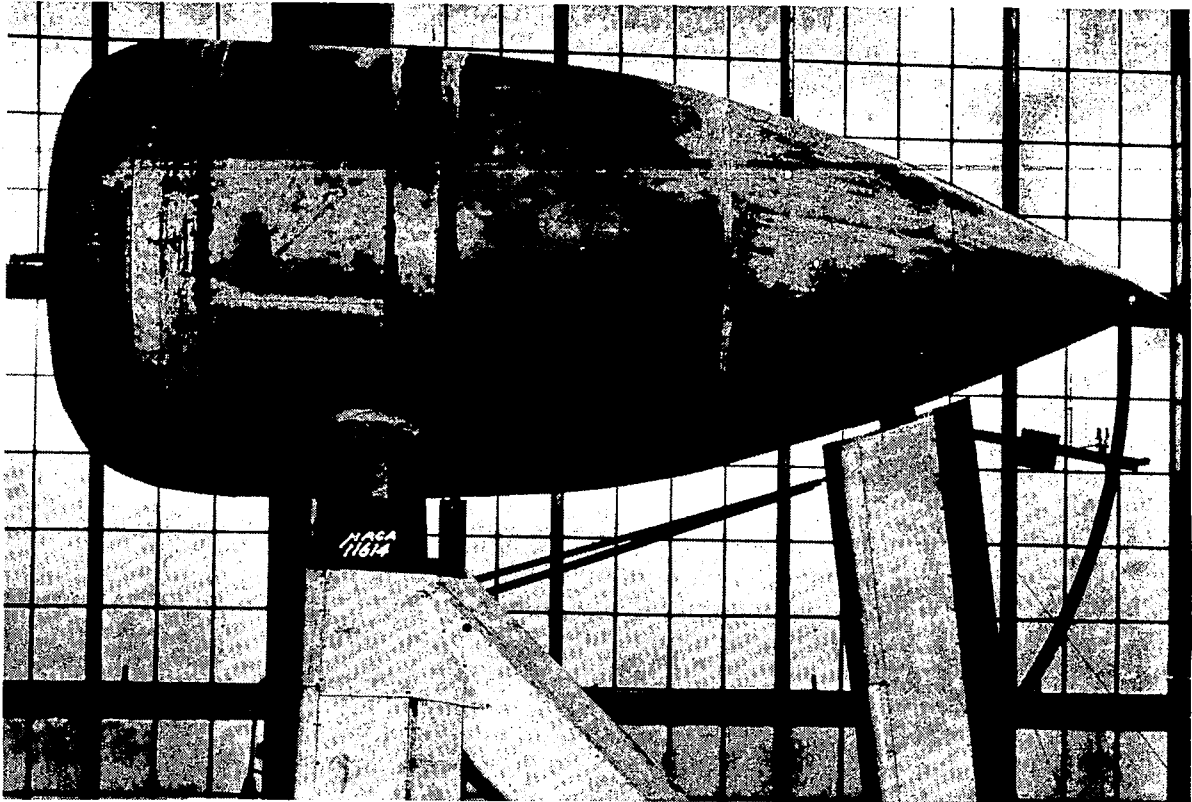
Figure 4.- Side view of set-up 1, nose 2, nacelle 2.
