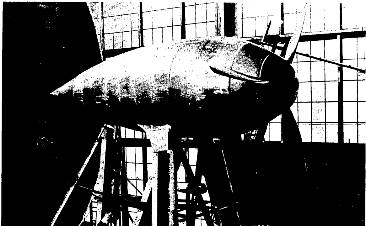
Figure 5.- The streamline shape used with set-up 2 with the propeller in place.
